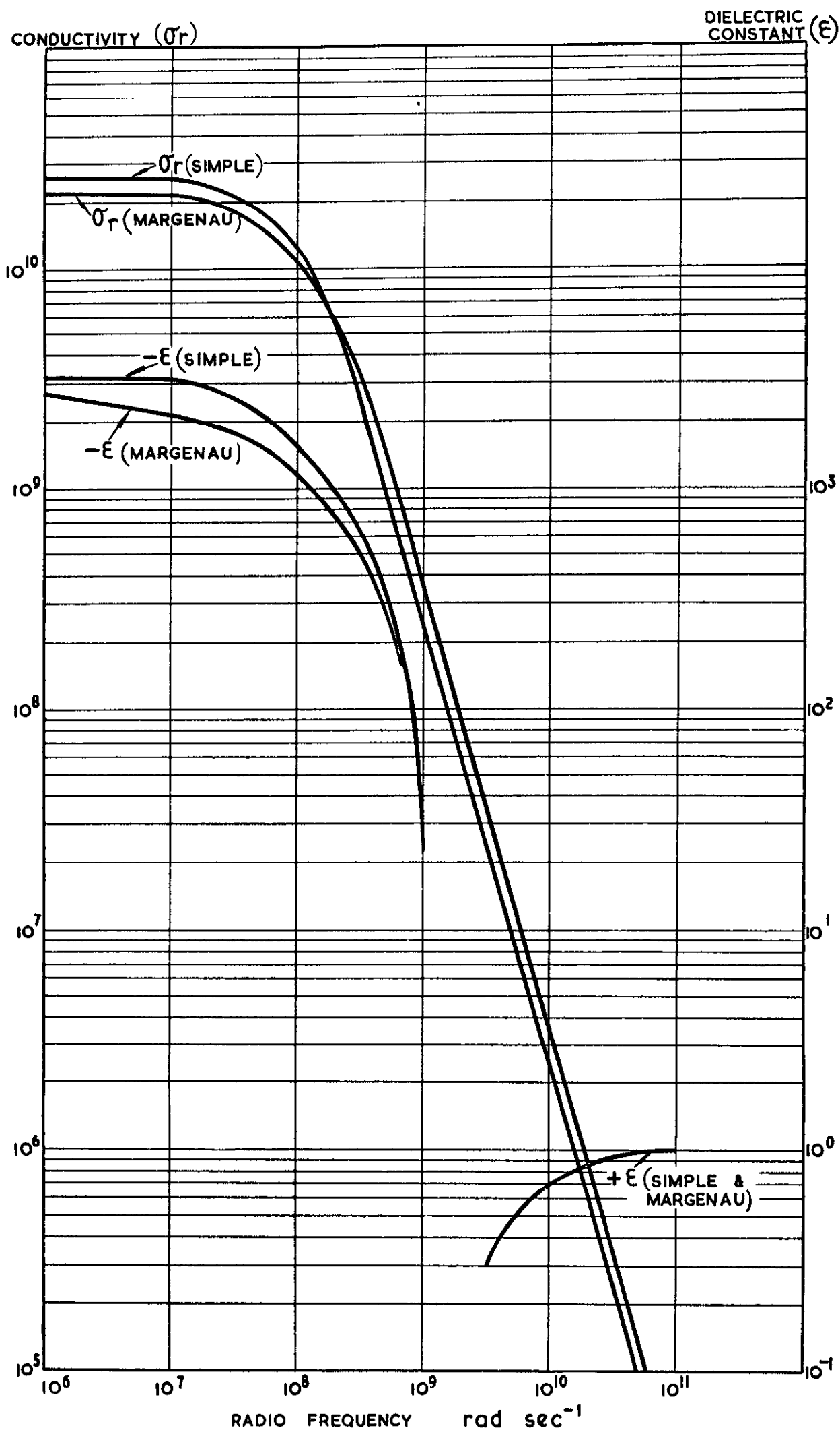
FIG. 1 COMPARISON OF SIMPLE THEORY WITH THAT OF MARGENAU N=10^{10} \text{ cm}^{-3} \omega_p=10^8 \text{ sec}^{-1}
