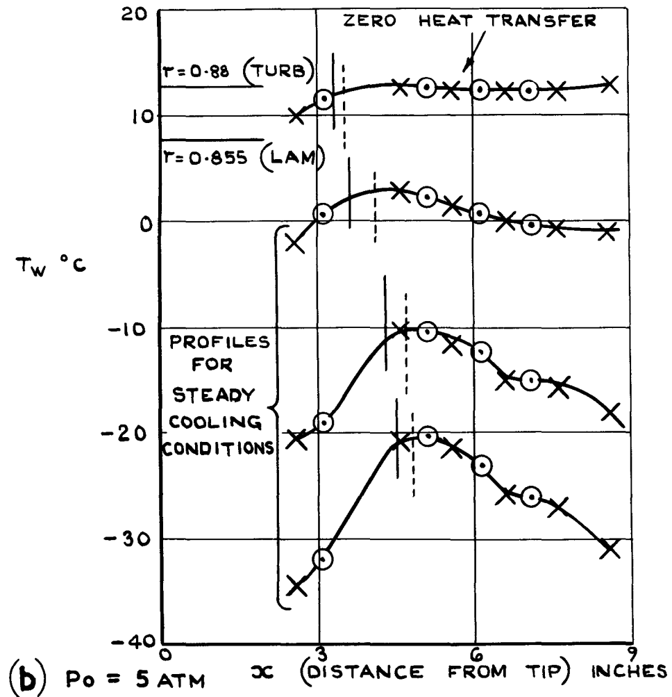
FIG. 3. (a & b.) TYPICAL DISTRIBUTIONS OF SURFACE TEMPERATURE ALONG THE 15^\circ STEEL CONE AT M_\infty = 3.13 WITH COOLANT FLOWING FROM BASE TO TIP (ZERO INCIDENCE.)
