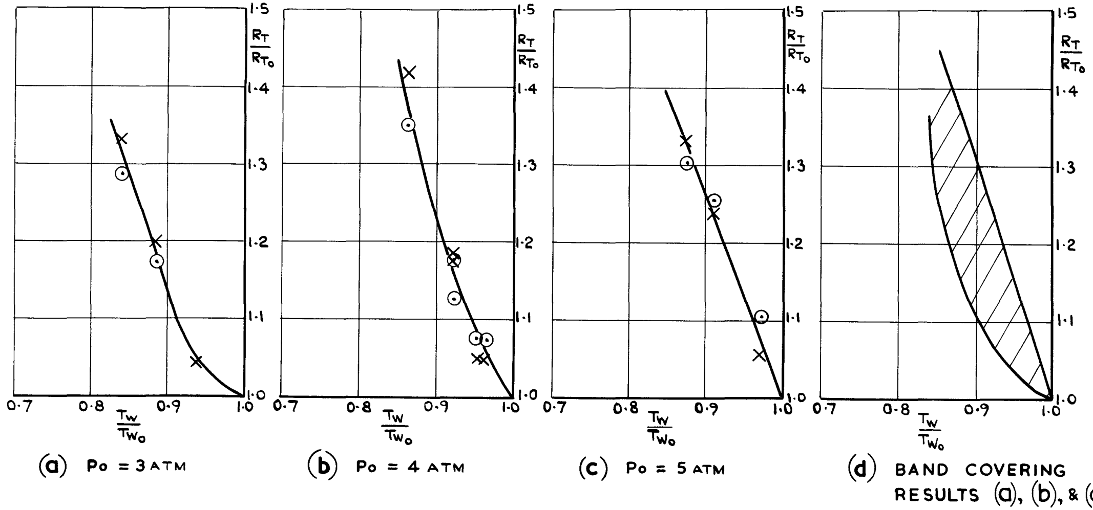
FIG. 6. (a, b, c, & d) EFFECT OF COOLING ON TRANSITION REYNOLDS NUMBER (FROM SHADOWGRAPH) AT M_{\infty} = 3.13 , ( M_1 = 2.93 ), AND P_0 = 3-5 \text{ ATM} . (ZERO INCIDENCE) ( R_{T_0} VALUES USED BEING THOSE INDICATED IN FIG. 5.)
