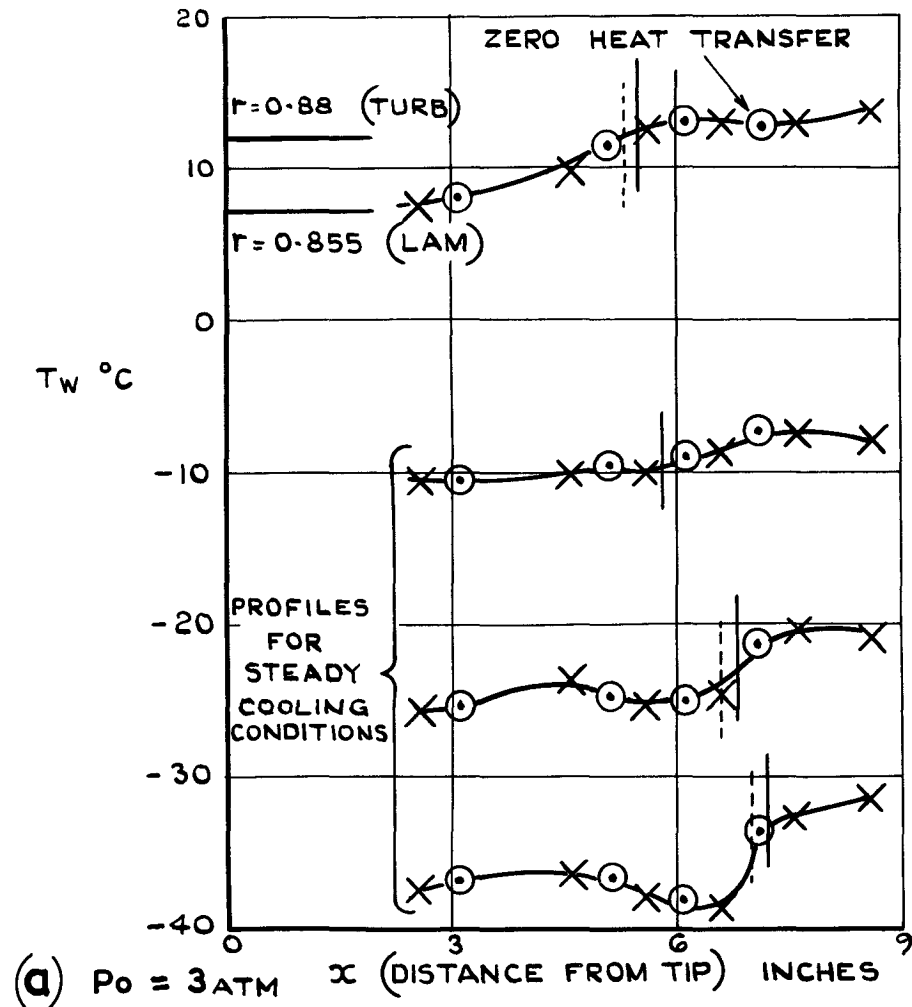
FIG. 3. (a & b.) TYPICAL DISTRIBUTIONS OF SURFACE TEMPERATURE ALONG THE 15^\circ STEEL CONE AT M_\infty = 3.13 WITH COOLANT FLOWING FROM BASE TO TIP (ZERO INCIDENCE.)
