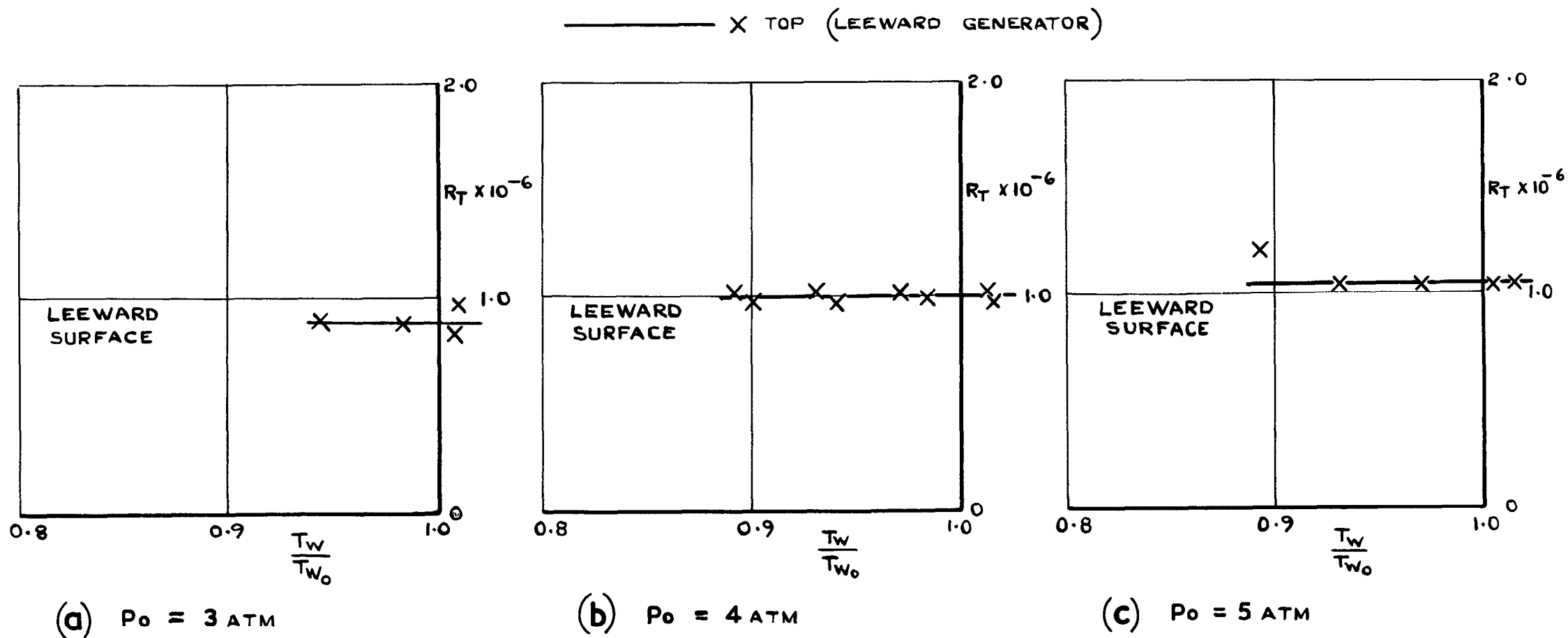
FIG. 14. (a, b, & c) EFFECT OF 2^\circ POSITIVE INCIDENCE ON MOVEMENT WITH COOLING OF TRANSITION POSITION ON THE LEEWARD GENERATOR OF A 15^\circ CONE AT M_\infty = 3.8 (TRANSITION DID NOT OCCUR ON THE WINDWARD GENERATOR AT THESE PRESSURES.) (FROM SHADOWGRAPH.)
