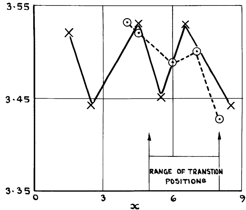
(b) M_\infty = 3.8
