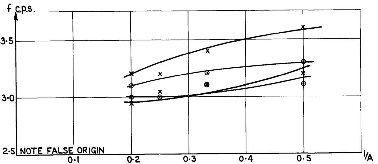
FIG. 3. THE VARIATION OF FLUTTER SPEED AND FREQUENCY WITH ASPECT RATIO FOR THE ROLL-AILERON ROTATION TYPE FLUTTER.
