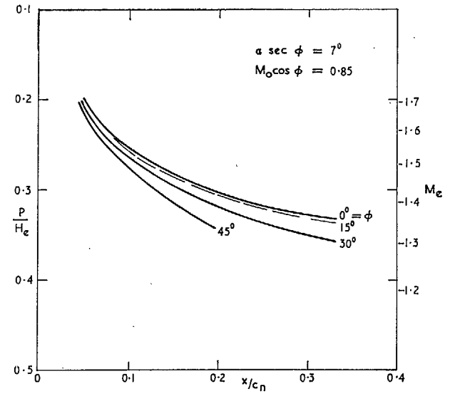
FIG. 17. Reconstruction, from Fig. 16, of the chordwise distribution of p/H_e at four sweep-back angles. M_e is the Mach number corresponding to p/H_e . Supersonic attached flow was not obtained in the test Mach number range with \phi = 60^\circ .
