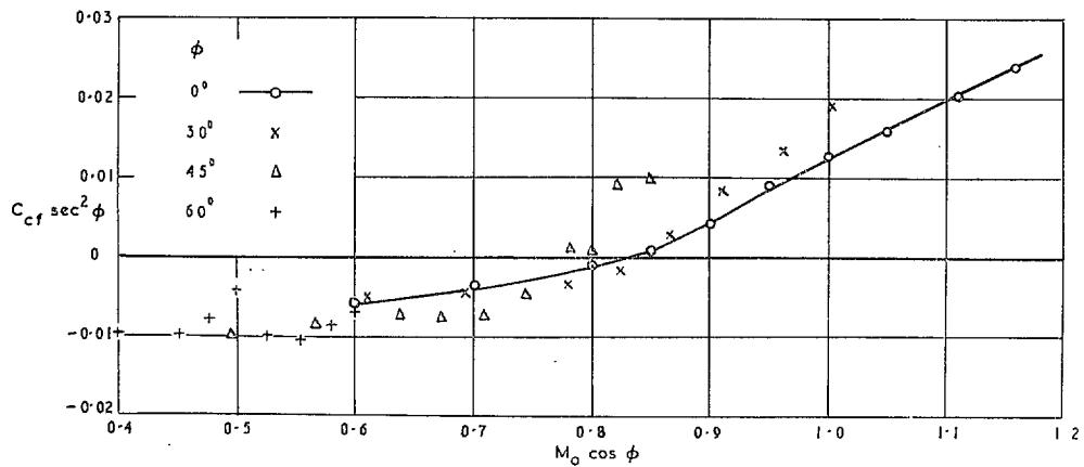
FIG. 31b. Correlation of reduced chordwise pressure-force coefficients for single-wedge profile at zero incidence (coefficients determined for front half of 7% thick double-wedge section).
