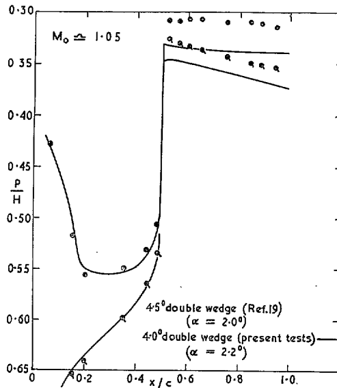
FIG. 13b. Comparison of present results for \phi = 0^\circ with two-dimensional data at incidence.
