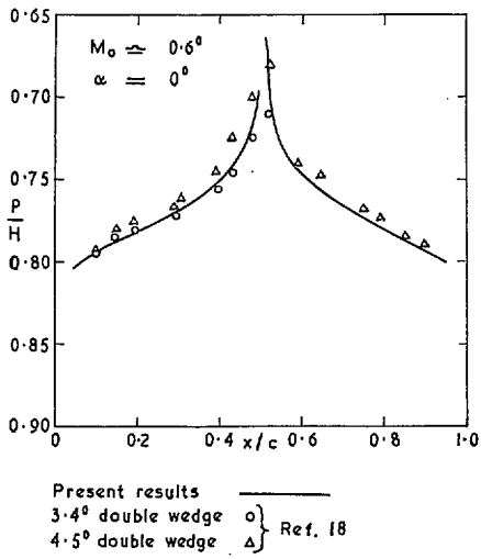
FIG. 13a. Comparison of present results for \phi = 0^\circ with two-dimensional data at zero incidence.
