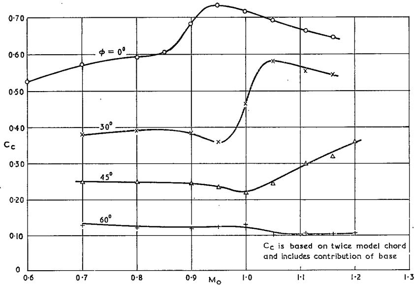
FIG. 33. Chordwise force coefficient of complete single-wedge profile at zero lift.
