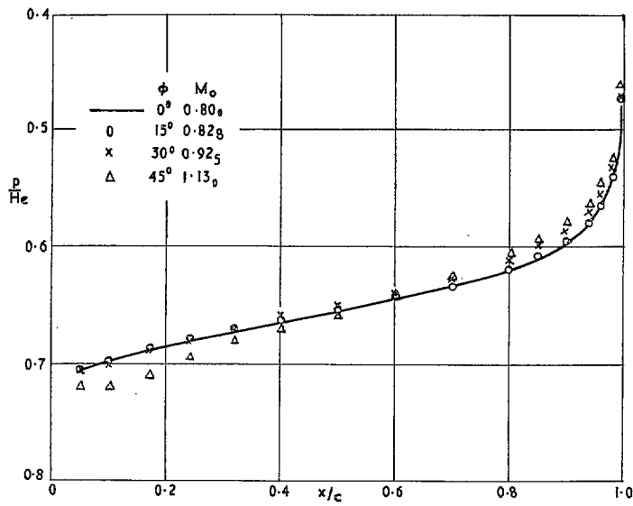
FIG. 15b. Comparison of pressure on forward face of single wedge at zero incidence and M_0 \cos \phi = 0.80 .
