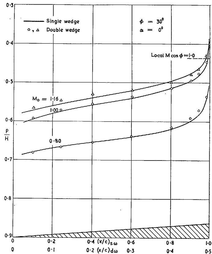
FIG. 21b. Comparison of forebody pressures at \phi = 30^\circ .
