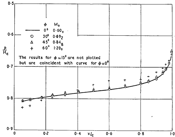
FIG. 15a. Comparison of pressures on forward face of single wedge at zero incidence and M_\infty \cos \phi = 0.60 .
