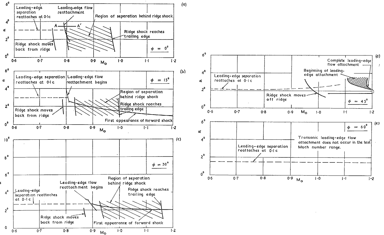
FIG. 6. Approximate flow boundaries for double-wedge wing.
