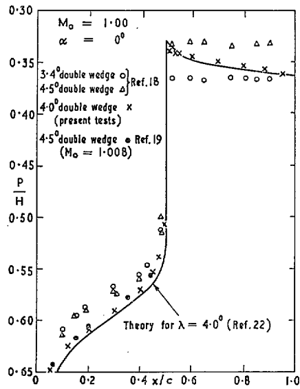
FIG. 13a. Comparison of present results for \phi = 0^\circ with two-dimensional data at zero incidence.
