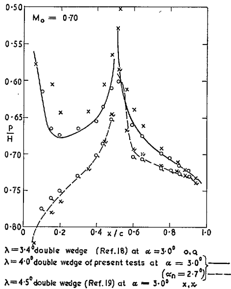
FIG. 13b. Comparison of present results for \phi = 0^\circ with two-dimensional data at incidence.
