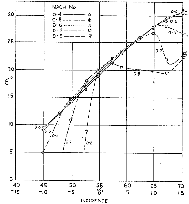
FIG. 4. Cascade 10C4/25C50.
