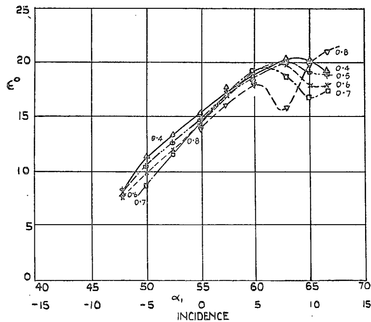
FIG. 12. Cascade 8.5CT(S)/25C50. \frac{\bar{w}}{P_{tot} - P_1} and \epsilon against \alpha_1 . High Mach numbers.
