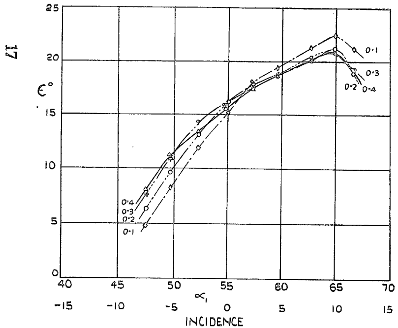
FIG. 11. Cascade 8.5CT(S)/25C50. \frac{\bar{w}}{P_{tot} - P_1} and \epsilon against \alpha_1 . Low Mach numbers.
