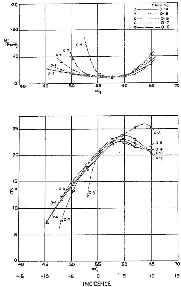
FIG. 14. Cascade 10.5/2A/25C50. \bar{w}/(P_{tot} - P_1) and \epsilon against \alpha_1 . High Mach numbers.
