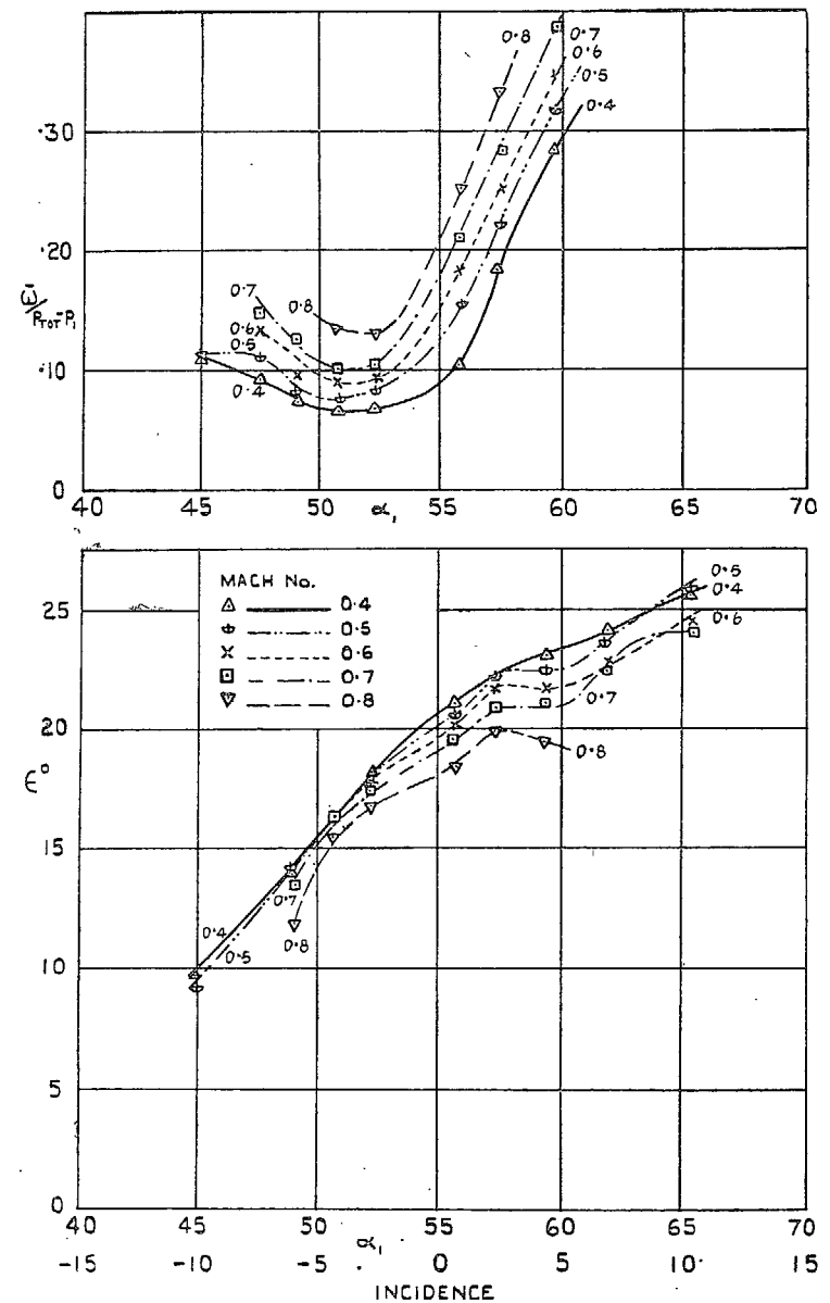
FIG. 10. Cascade 7.2CT/25P40. \frac{\bar{w}}{P_{tot} - P_1} and \epsilon against \alpha_1 . High Mach numbers.
