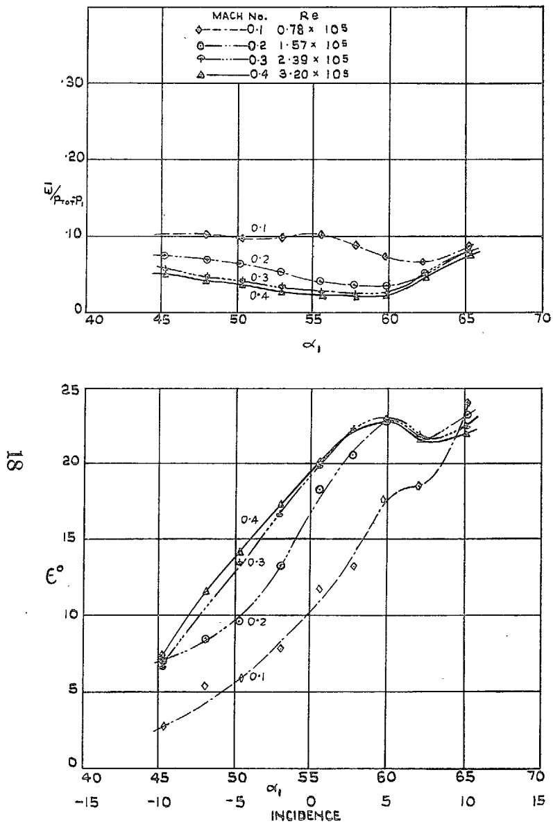
FIG. 13. Cascade 10.5/2A/25C50. \bar{w}/(P_{tot} - P_1) and \epsilon against \alpha_1 . Low Mach numbers.
