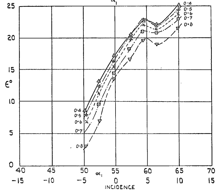
FIG. 8. Cascade 7.2CT/25C50.
