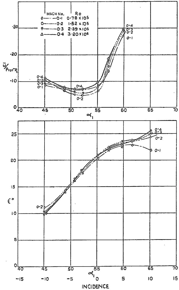
FIG. 9. Cascade 7.2CT/25P40. \frac{\bar{w}}{P_{tot} - P_1} and \epsilon against \alpha_1 . Low Mach numbers.
