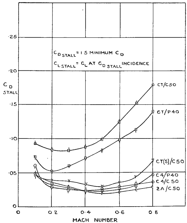
Stalling C_D against Mach number.
