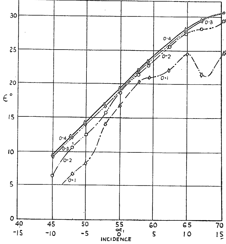
FIG. 3. Cascade 10C4/25P40.
