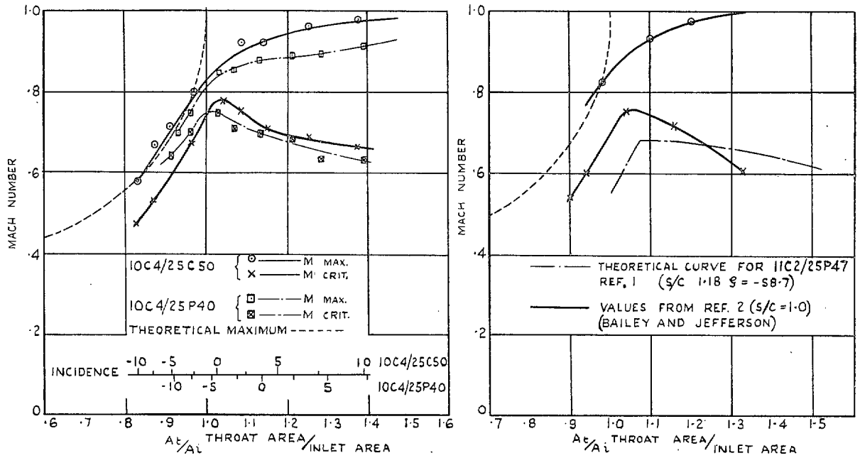
FIG. 20. Maximum and critical Mach numbers. Maximum M based on zero pressure rise (measured). Critical M based on 1.5 \times minimum loss.
