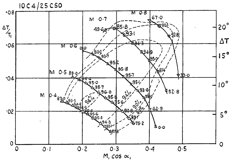
FIG. 19. \Delta T/T_1 against M \cos \alpha_1 . Values are for one blade row, i.e., half a stage. ——— Constant inlet Mach number. - - - - - Constant two-dimensional efficiency. \Delta T scale for T_1 = 288^\circ \text{K} .
