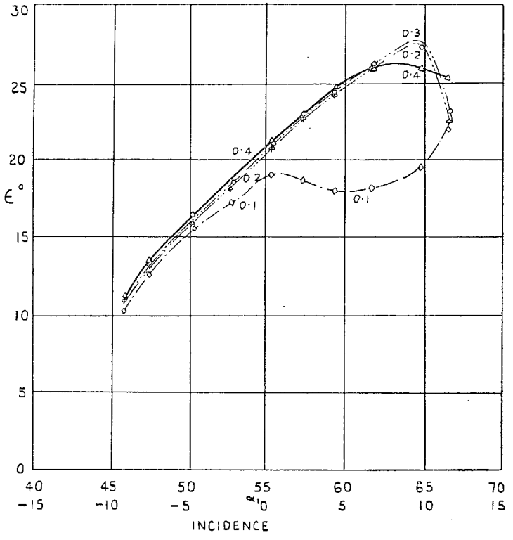
FIG. 5. Cascade 10C4/25P40. \frac{\bar{w}}{P_{tot} - P_1} and \epsilon against \alpha_1 . Low Mach numbers.
