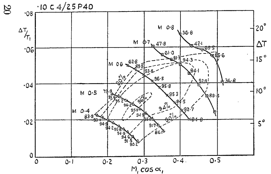
FIG. 17. \Delta T / T_1 against M \cos \alpha_1 . Values are for one blade row, i.e., half a stage. ——— Constant inlet Mach number. - - - - - Constant two-dimensional efficiency. \Delta T scale for T_1 = 288^\circ \text{K} .
