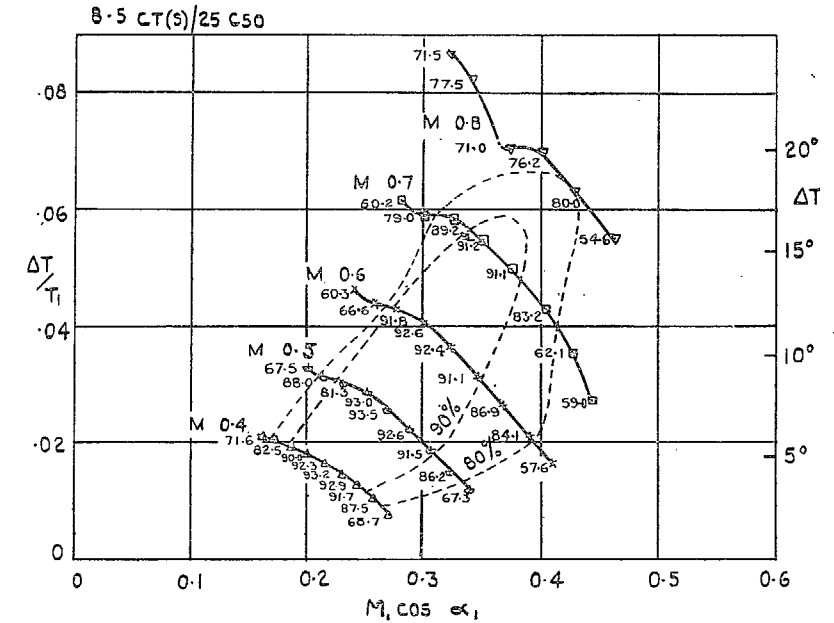
FIG. 18. \Delta T / T_1 and \Delta P / P_1 against M \cos \alpha_1 . Values are for one blade row, i.e., half a stage. ——— Constant inlet Mach number. - - - - - Constant two-dimensional efficiency \Delta T scale for T_1 = 288^\circ \text{K} .
