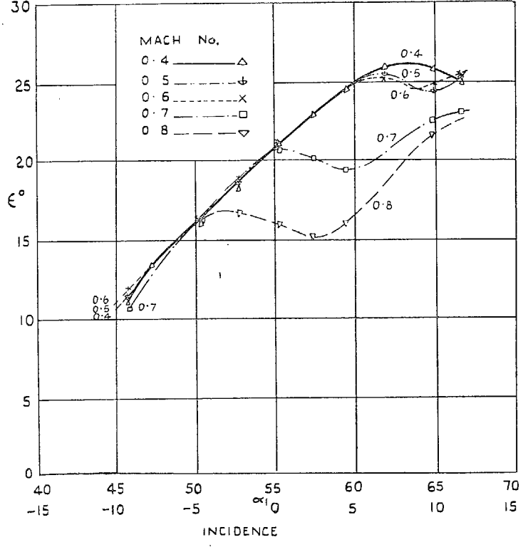
FIG. 6. Cascade 10C4/25P40. \frac{\bar{w}}{P_{tot} - P_1} and \epsilon against \alpha_1 . High Mach numbers.
