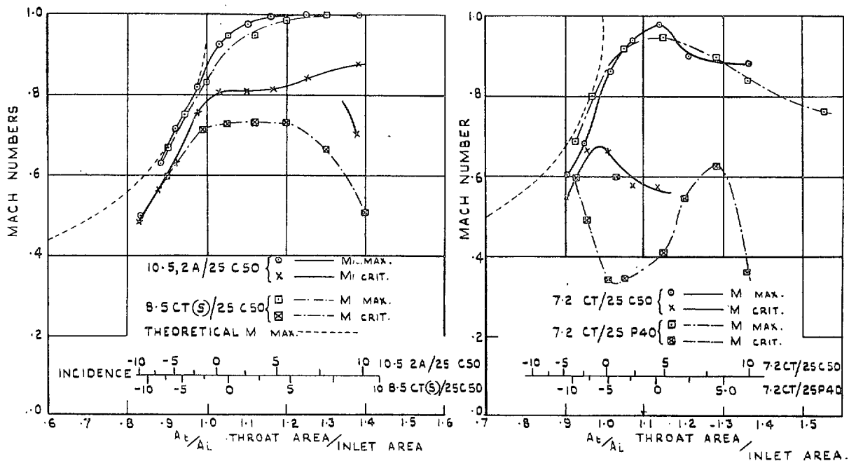
FIG. 21. Maximum and critical Mach numbers. Maximum M based on zero pressure rise (measured). Critical M based on 1.5 \times minimum loss.
