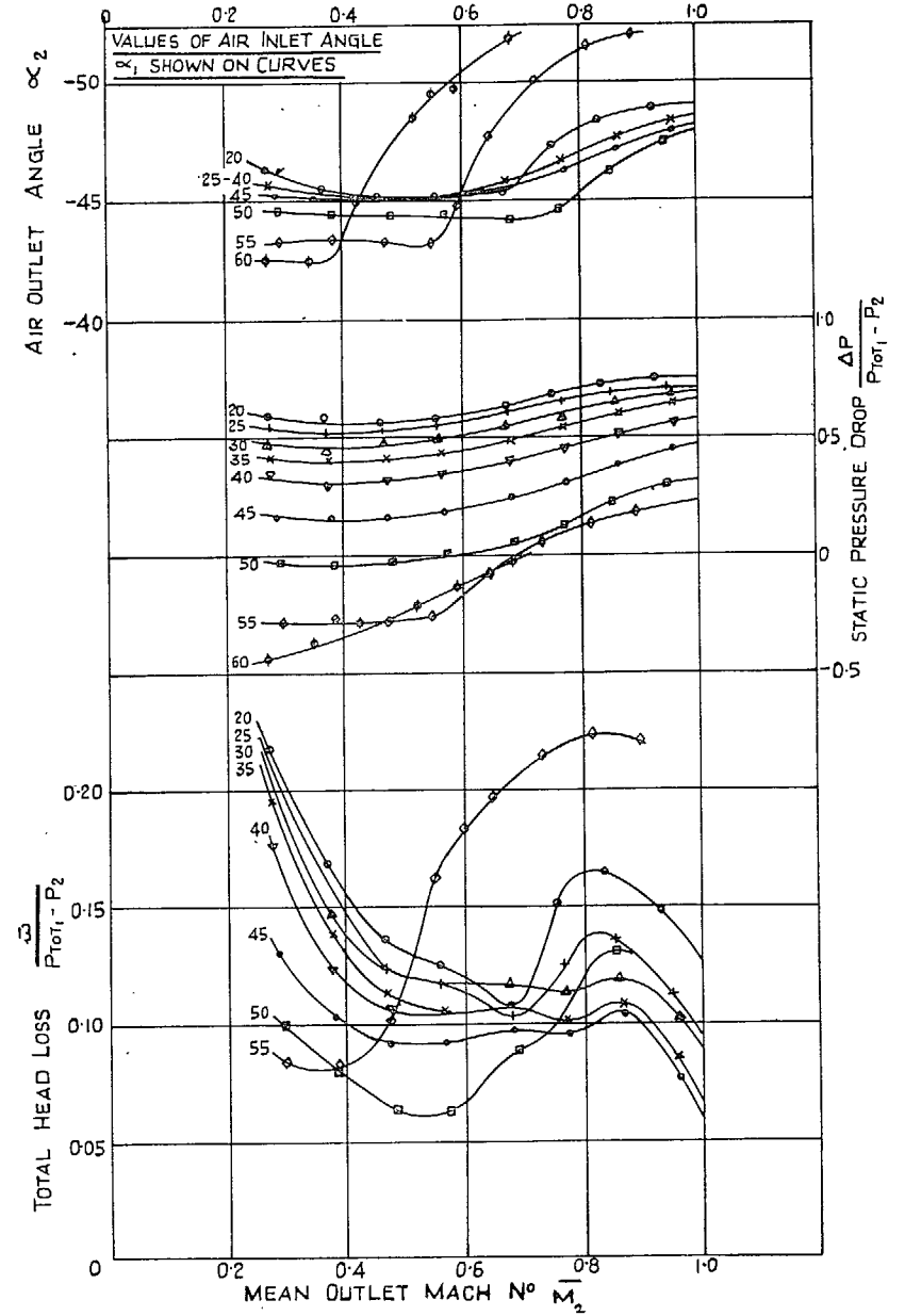
FIG. 10. Cascade No. 5. Design inlet angle 45 deg. \text{Cos}^{-1}(\text{throat/pitch}) = -50 \text{ deg.}
