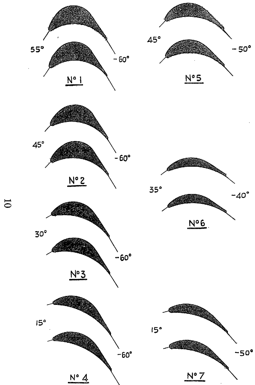
FIG. 5. Cascade details. Pitch/width = 0.625. Values of design inlet angles and \cos^{-1} (throat/pitch) as indicated.
