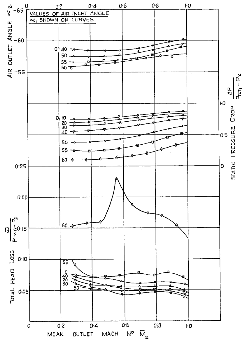
FIG. 8. Cascade No. 3. Design inlet angle 30 deg. \text{Cos}^{-1}(\text{throat/pitch}) = -60 deg.
