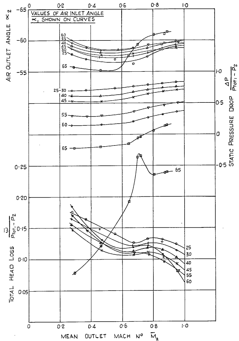
FIG. 6. Cascade No. 1. Design inlet angle 55 deg. \cos^{-1} (throat/pitch) = -60 deg.
