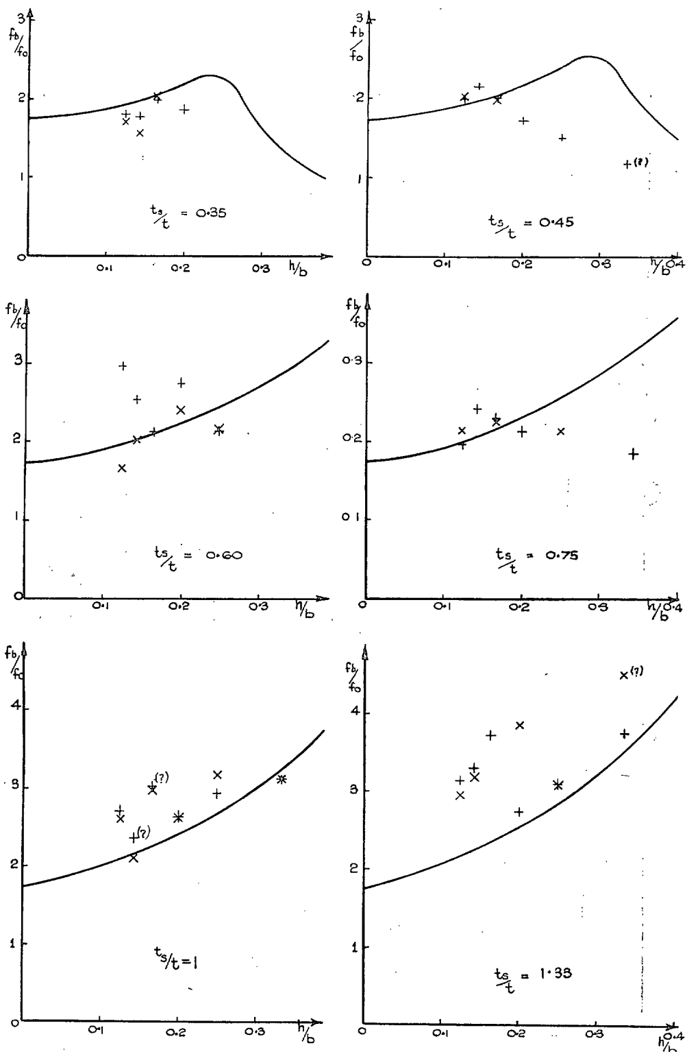
FIG. 8. Comparison of the theoretical results of Fig. 7 with the experimental results obtained by A. J. Monk.
