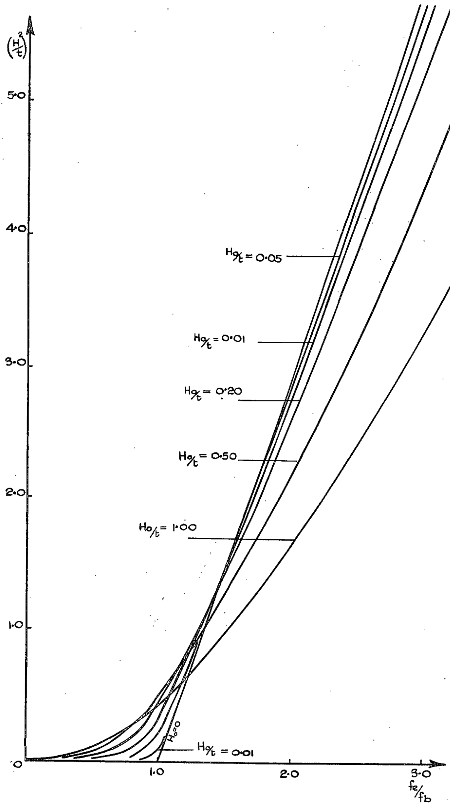
FIG. 11. H^2-f_c curves for various H_0 .
