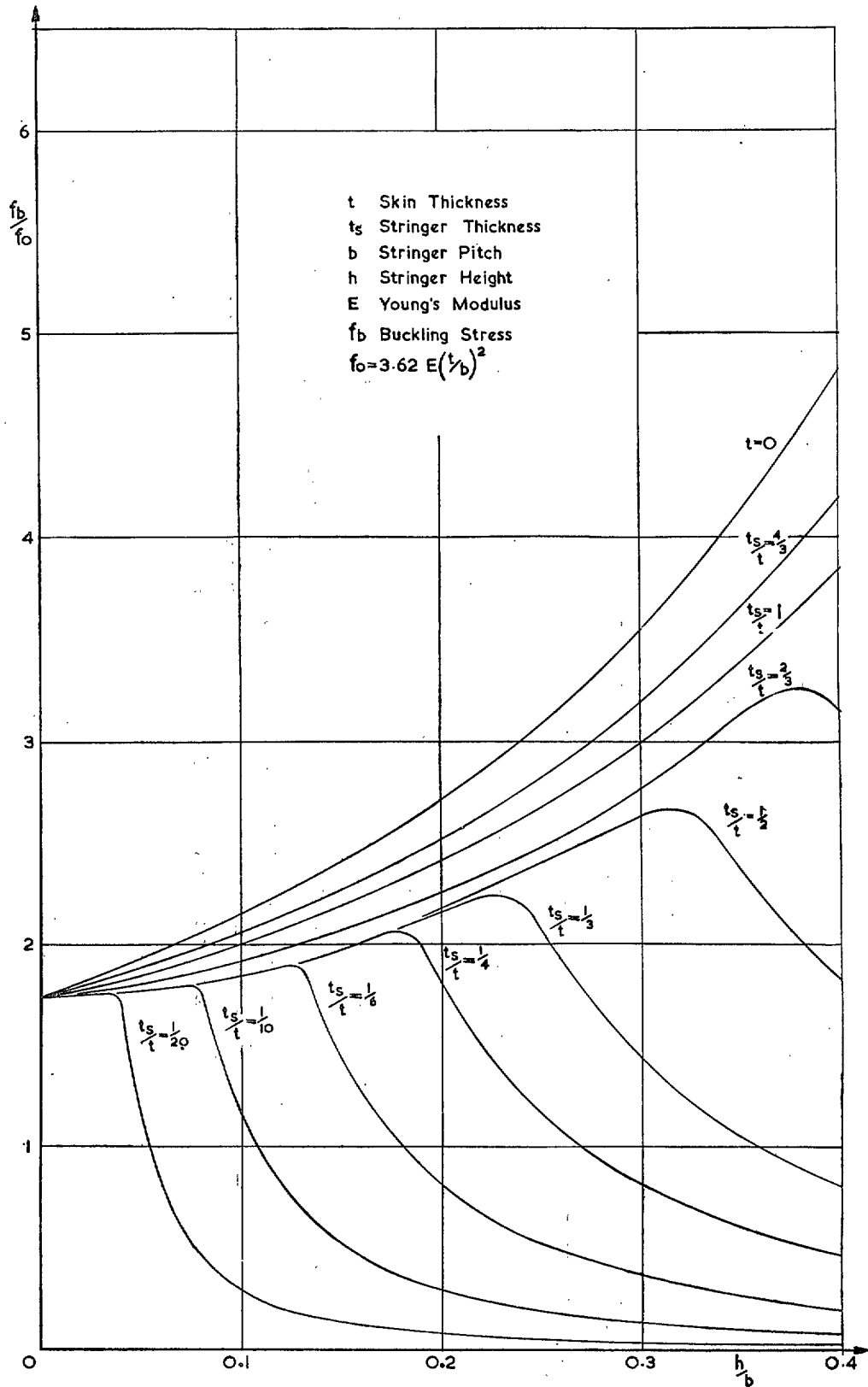
FIG. 7. The buckling stress in compression of panels with square top-hat section stringers.
