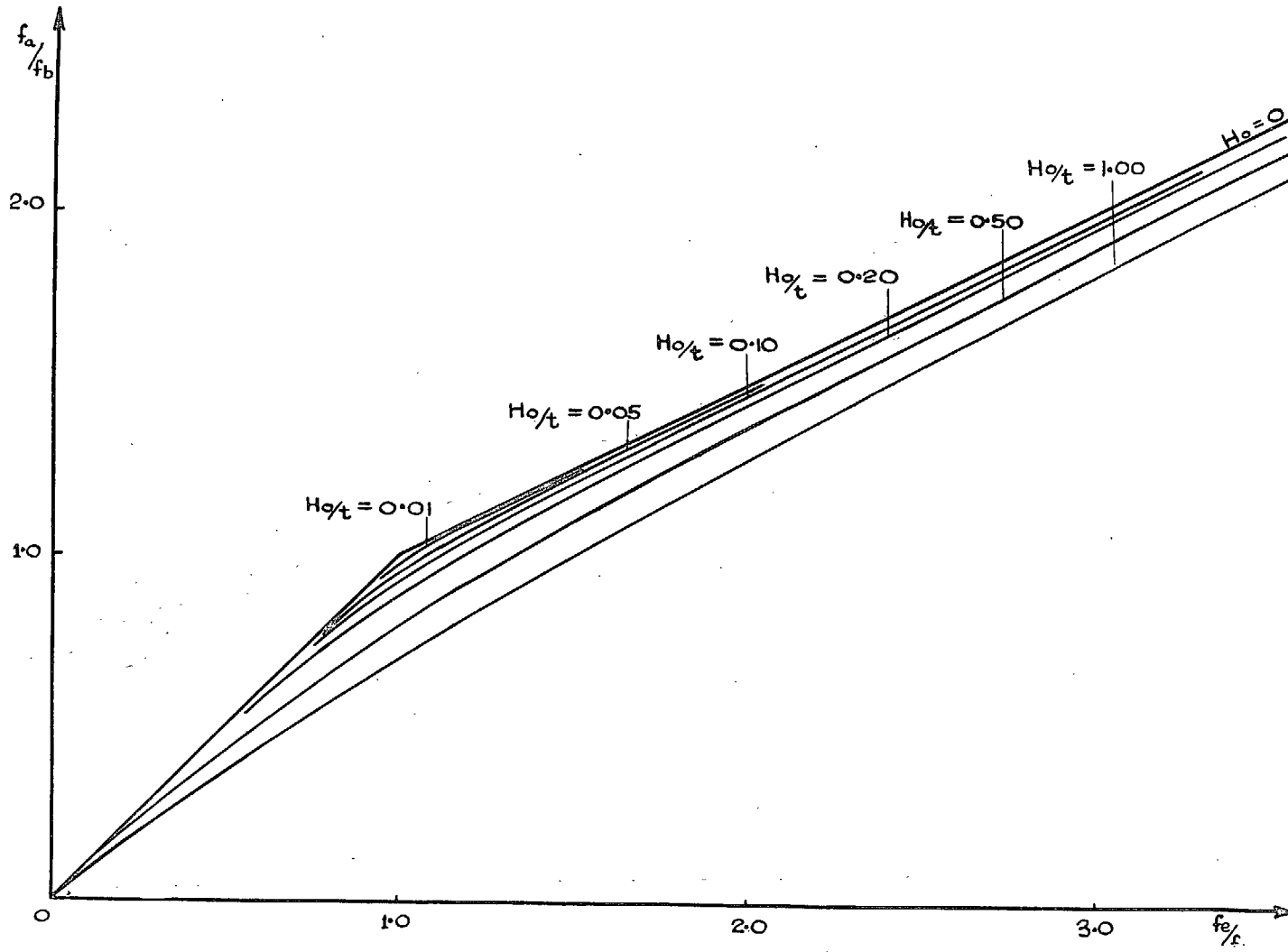
FIG. 10. f_a - f_e curves for various values of the initial eccentricity ( H_0 ).
