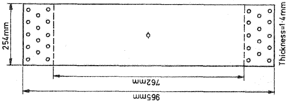
a Test specimen
