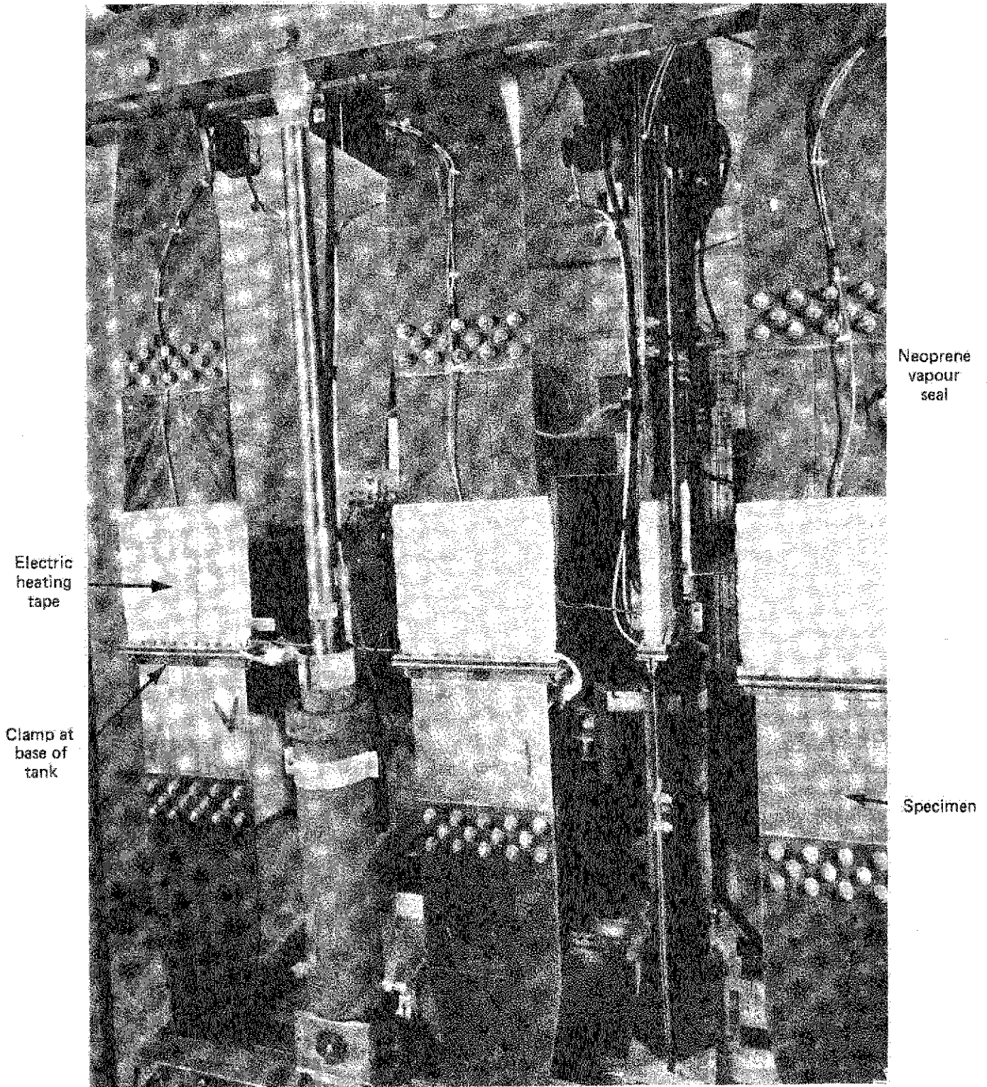
Fig.2 Fatigue test rig
