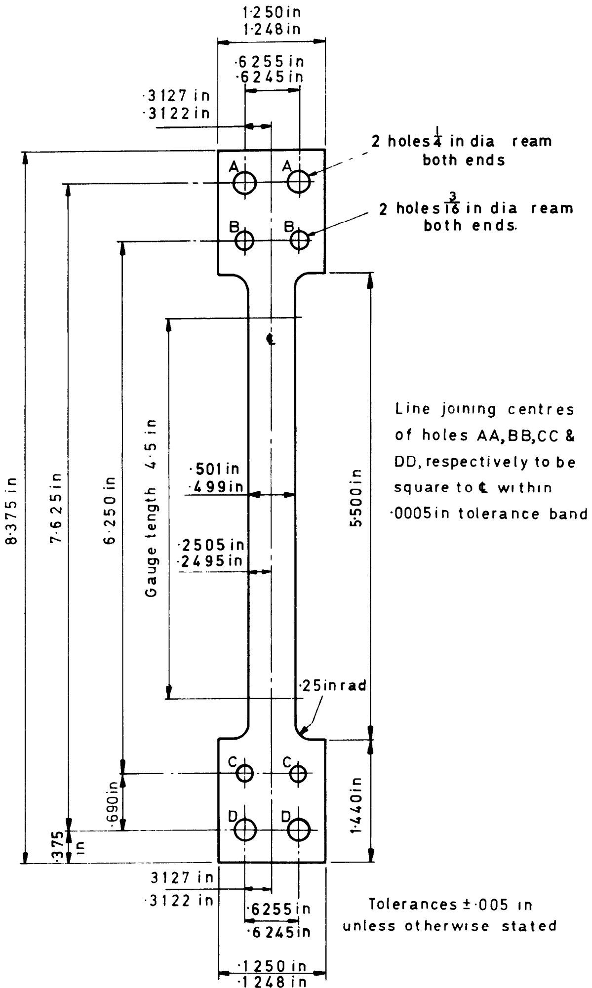
Fig.2 Test specimen of BNF design.
