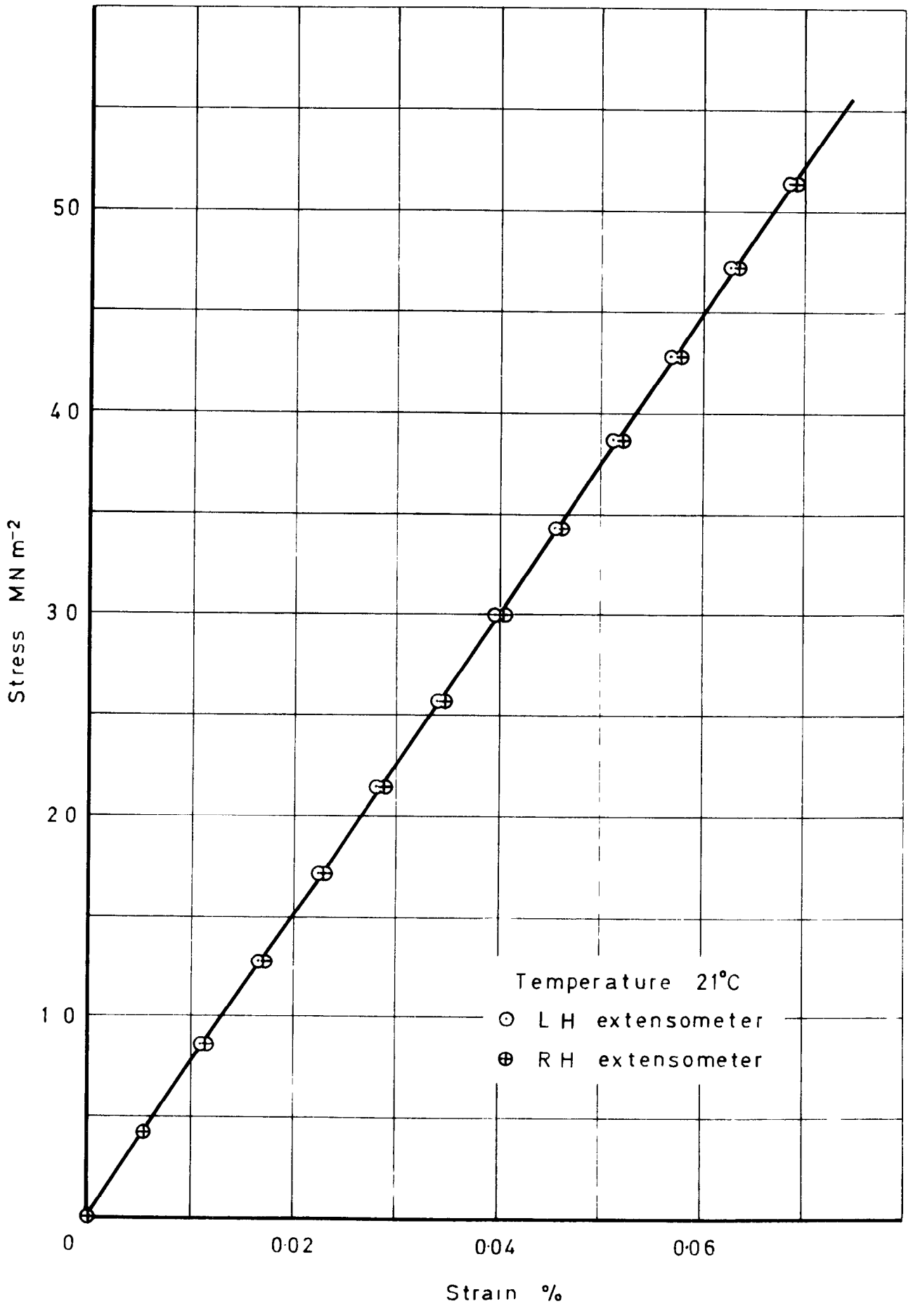
Fig.11 Typical incremental loading test — RE16
