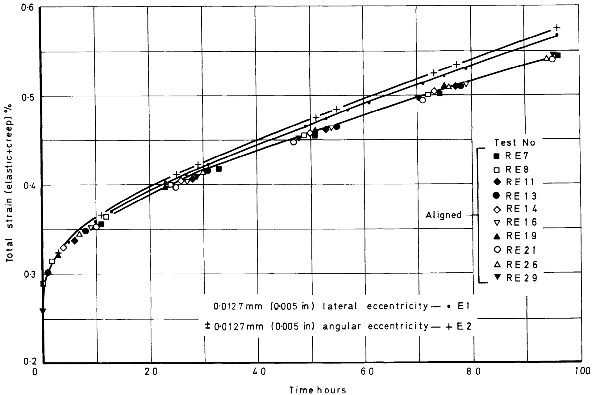
Fig. 21 Effect of eccentricity on creep strain— 170 \text{ MN m}^{-2} ( 11 \text{ ton in}^{-2} ) at 180^\circ\text{C}
