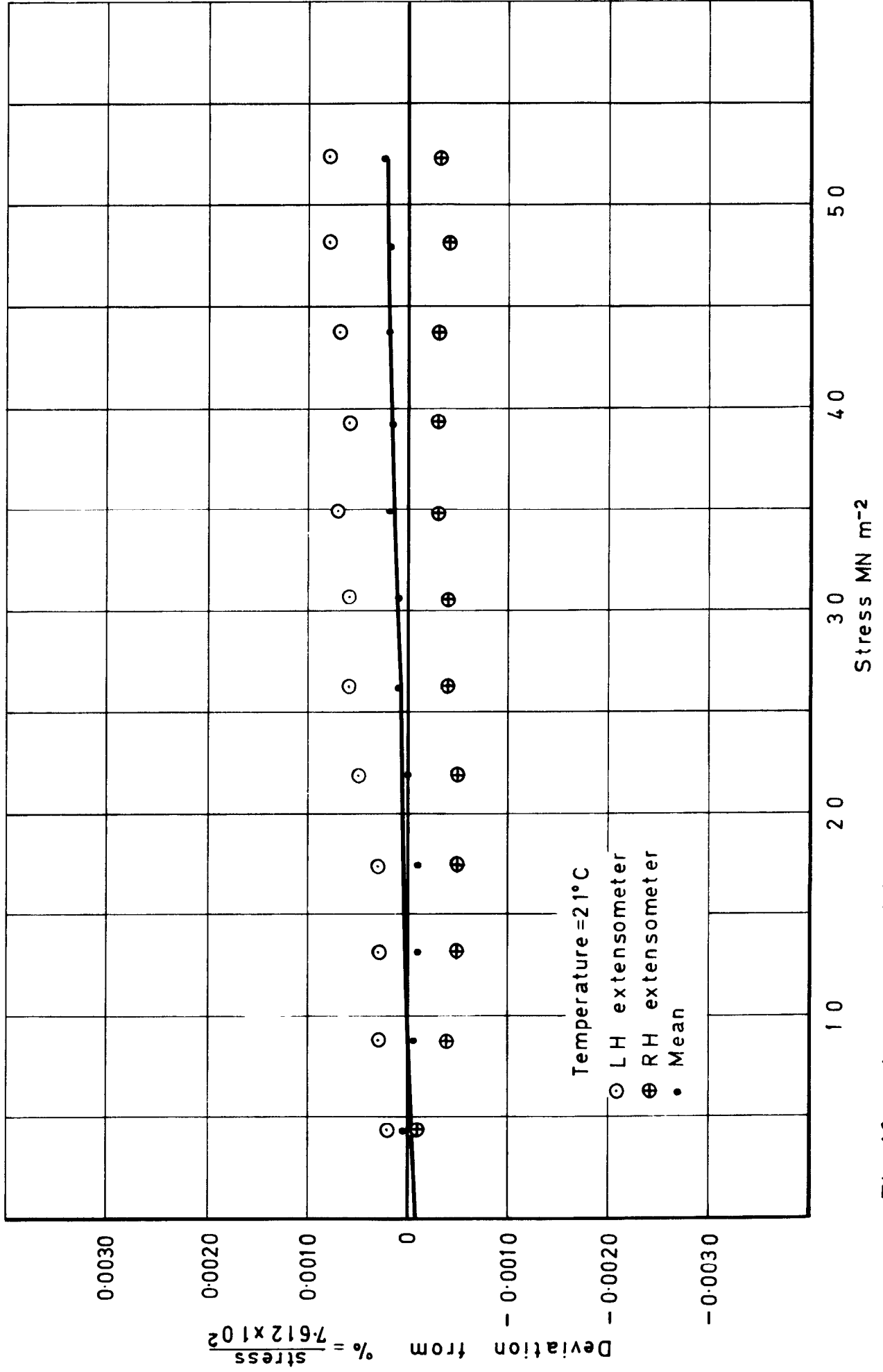
Fig. 19 Incremental loading with ±0.0051mm (0.002 in) angular eccentricity—E3
