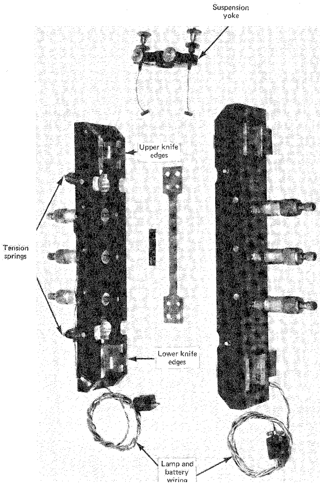
Fig.5 Measuring bars and suspension yoke
