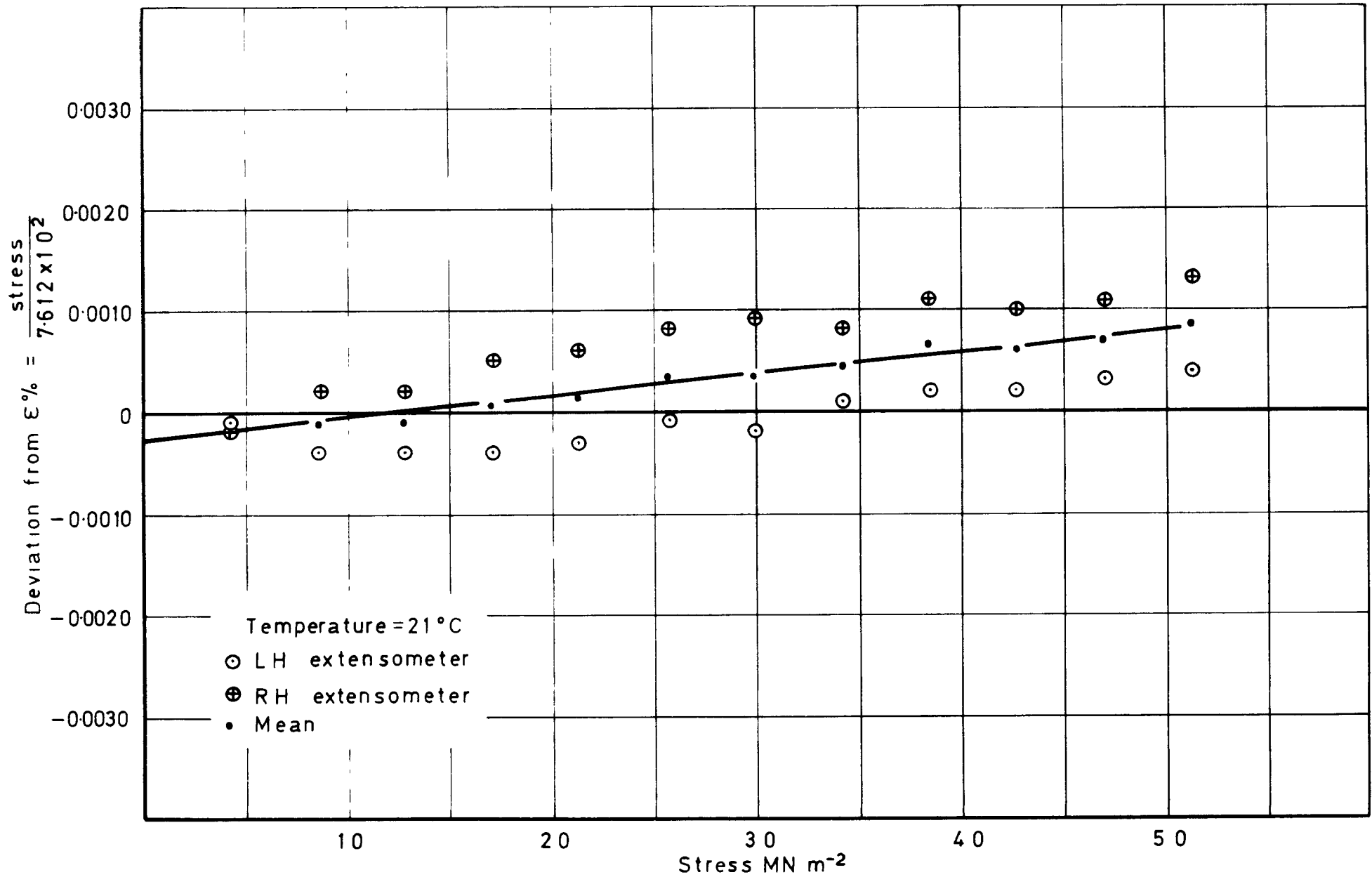
Fig.12 Typical incremental loading with aligned specimen: test — RE16
