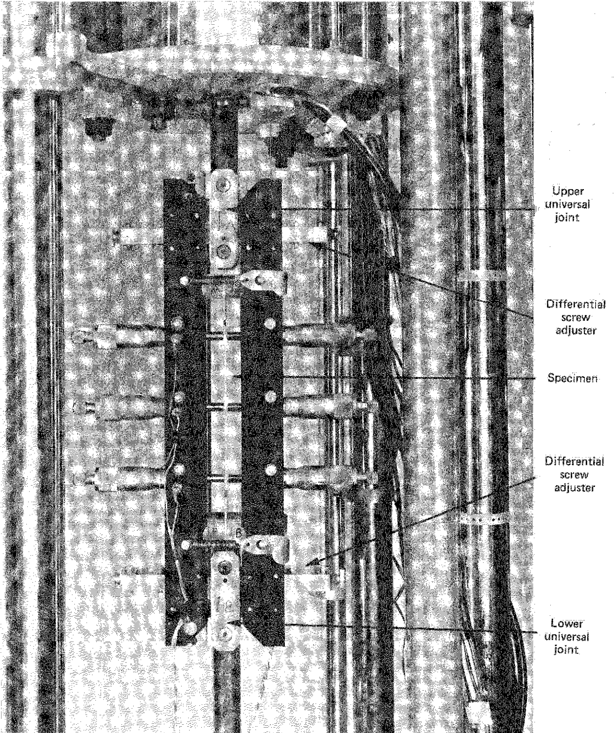
Fig.7 Thickness alignment
