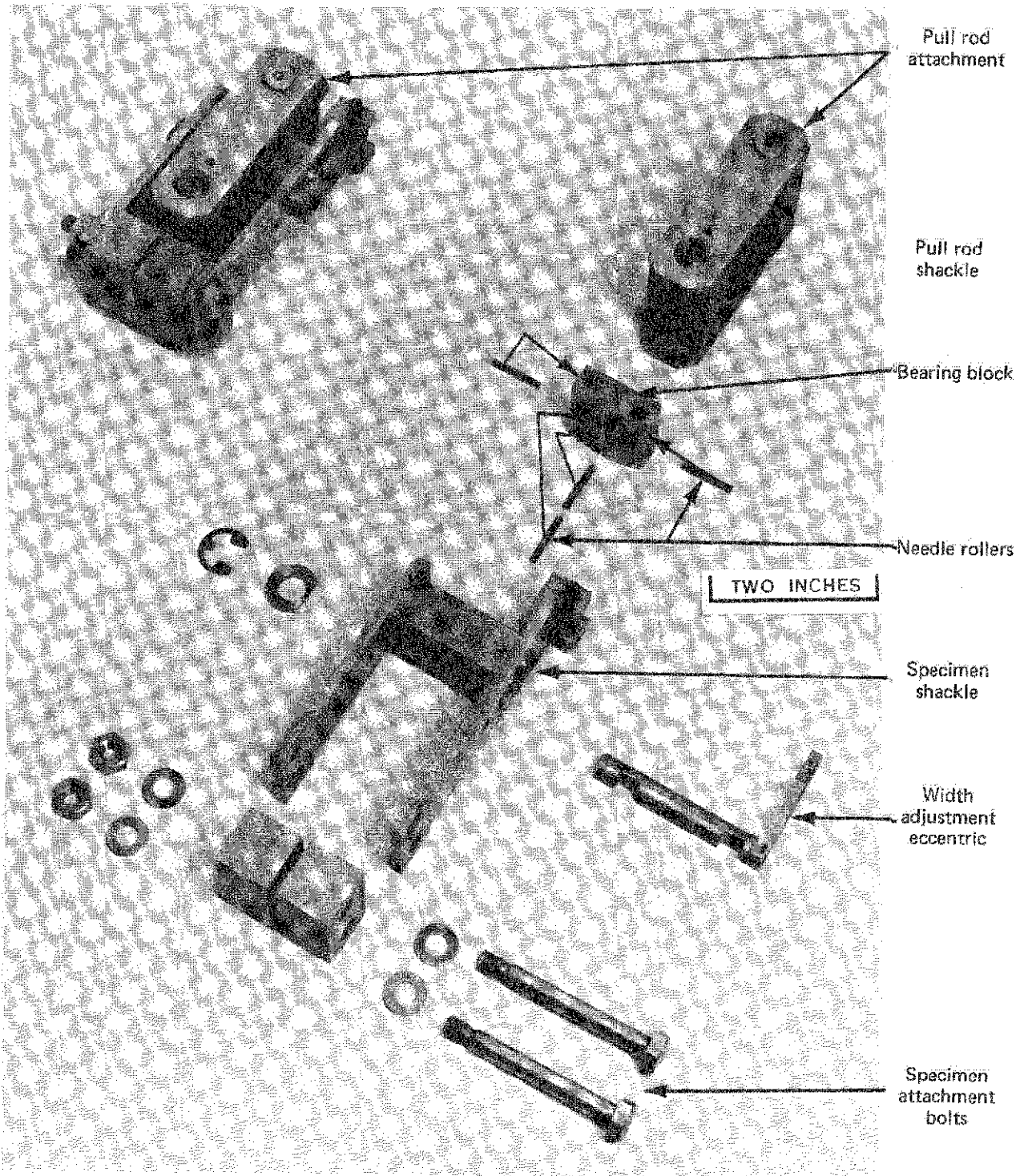
Fig.3 Universal joint construction
