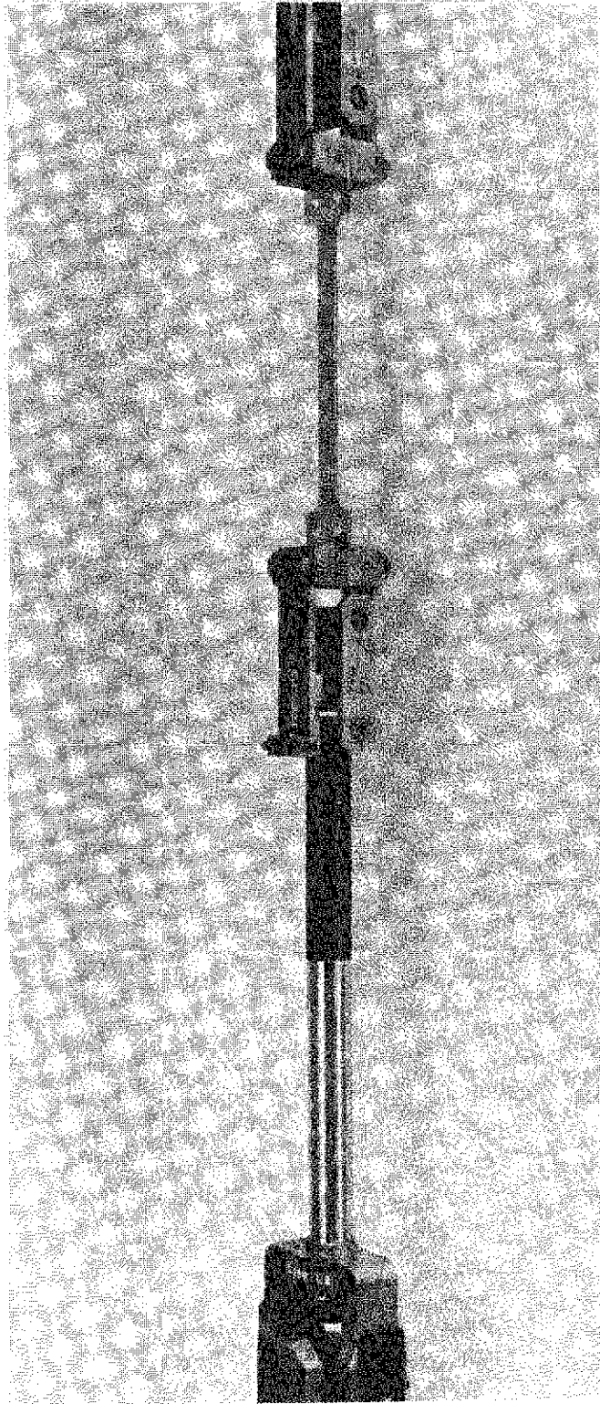
Fig.4 Universal joints and specimen assembly
