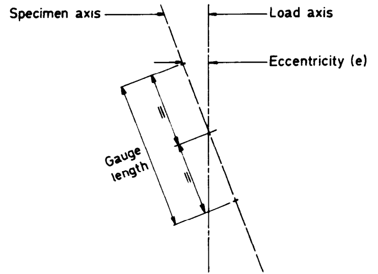
c Angular eccentricity
