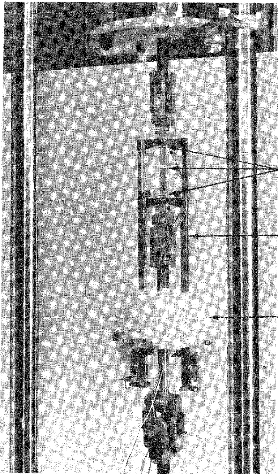
Fig.9 Completed test assembly
