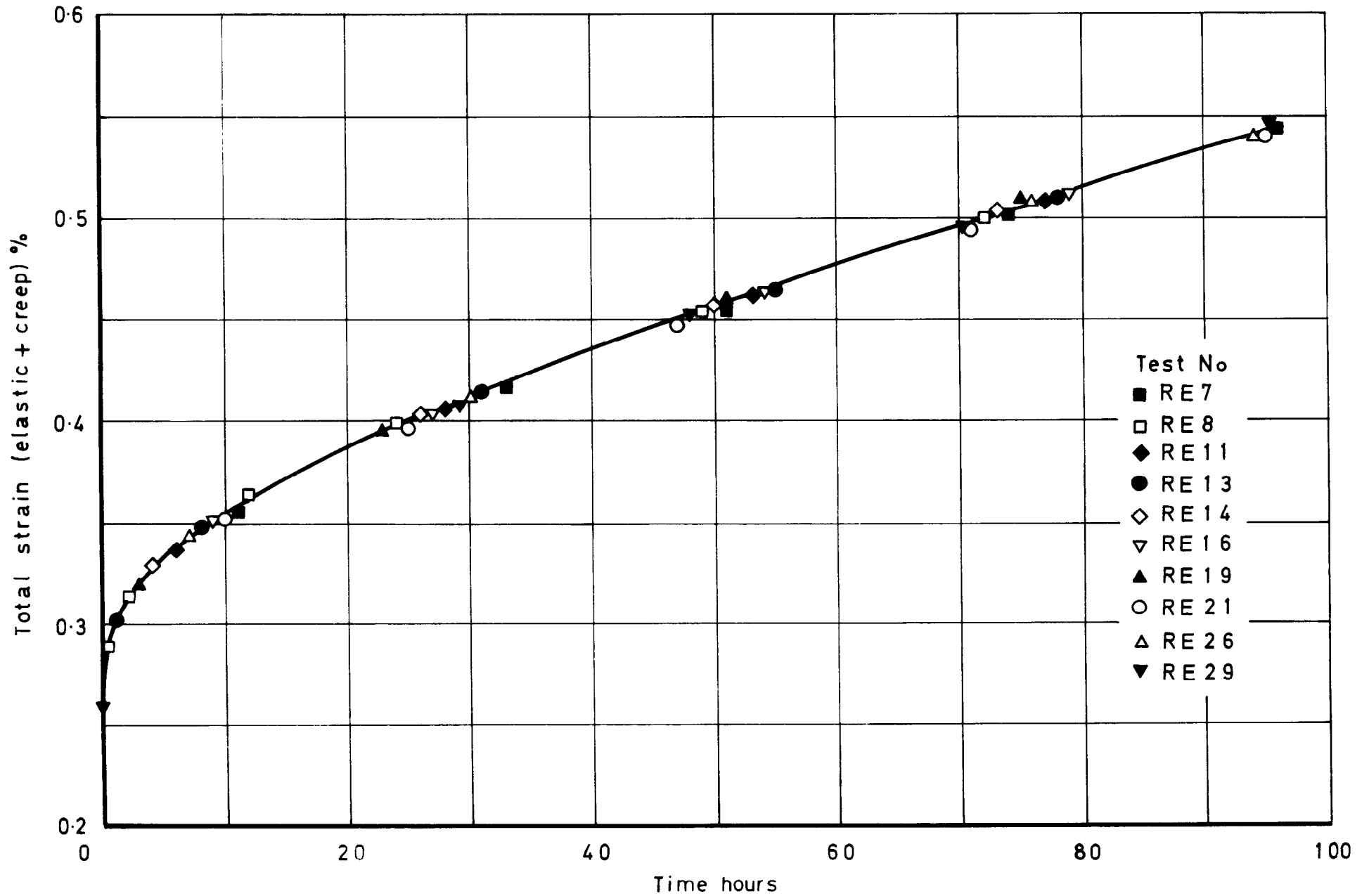
Fig.13 Creep repeatability — 170 \text{ MN m}^{-2} ( 11 \text{ ton in}^{-2} ) at 180^\circ\text{C}
