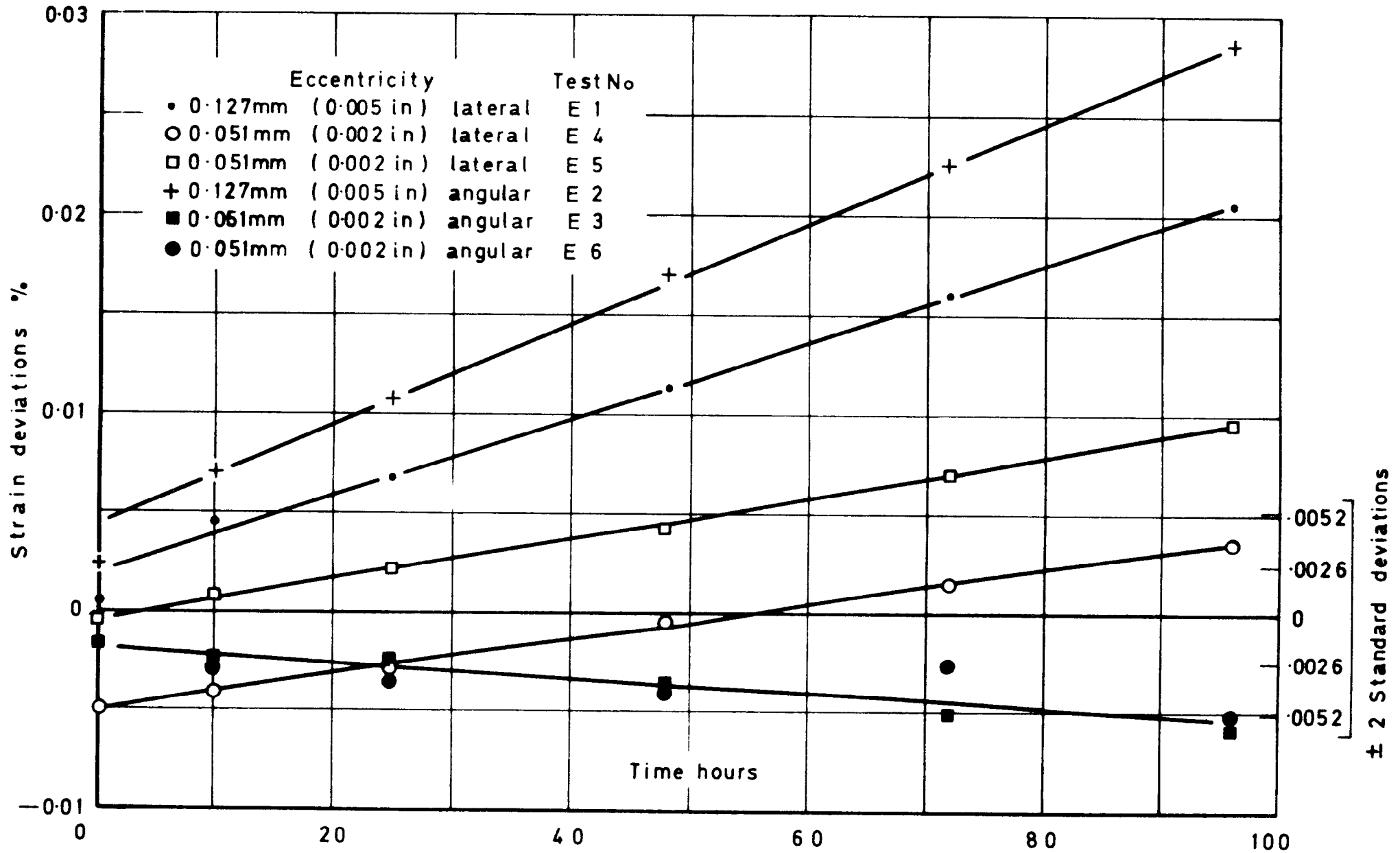
Fig. 22 Deviations of eccentric tests from mean creep curve— 170 \text{ MN.m}^{-2} ( 11 \text{ ton in}^{-2} ) at 180^\circ\text{C}
