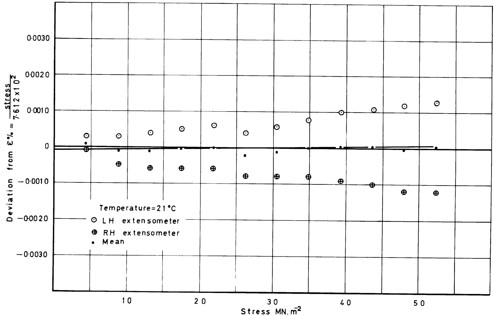
Fig.16 Incremental loading with 0.0051mm (0.002in) lateral eccentricity—E4
