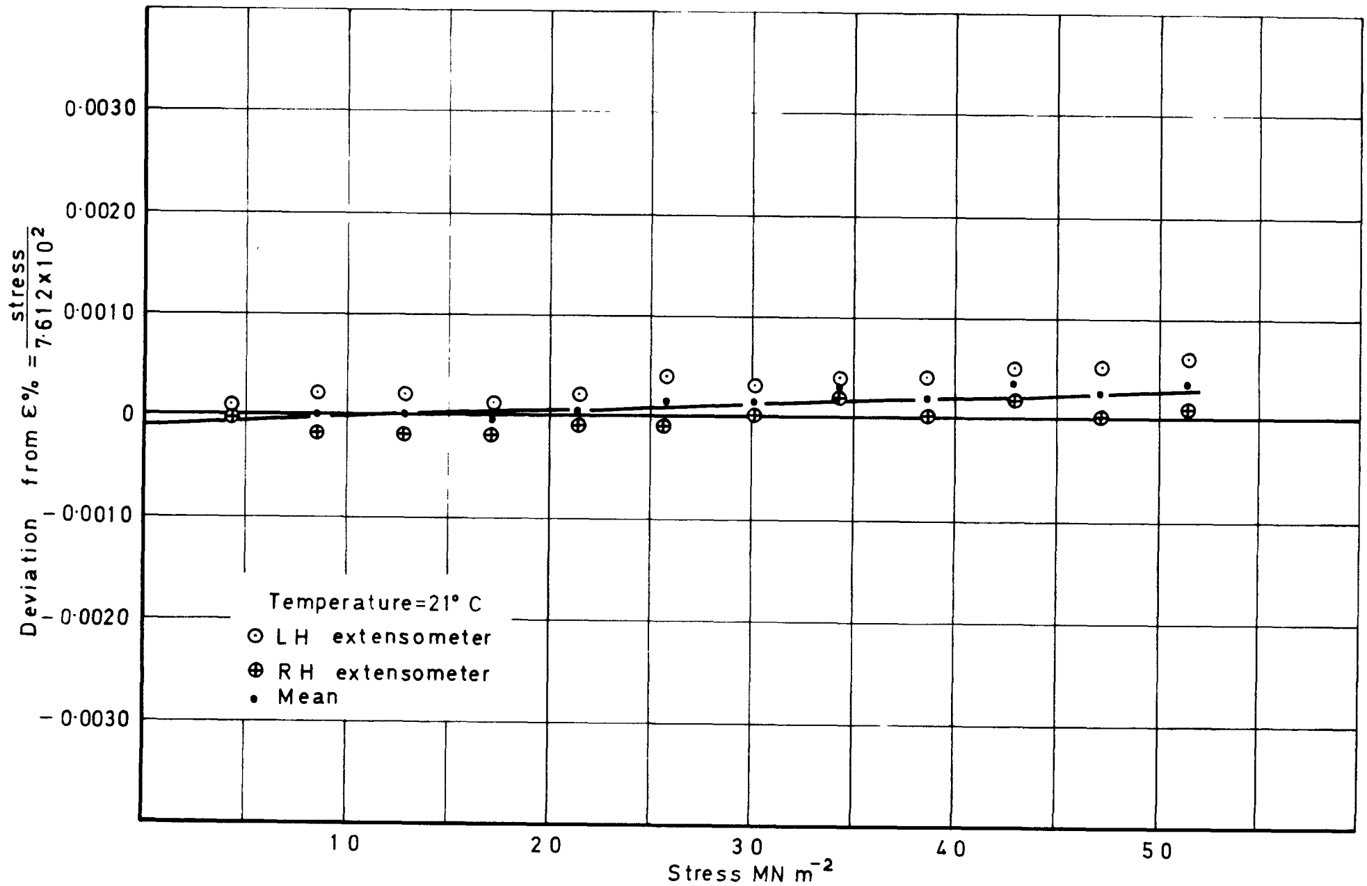
Fig. 2.0 Incremental loading with \pm 0.0051 mm (0.002 in) angular eccentricity—E6
