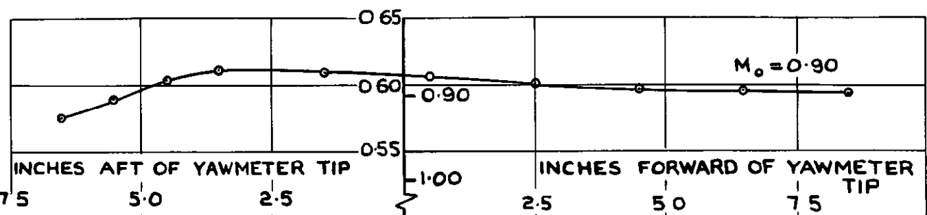
FIG. 9. RESULTS OF PROBE TRAVERSES.
