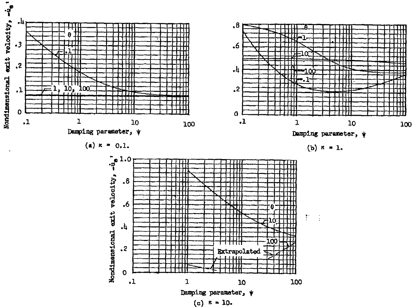
Figure 4.- Variation of nondimensional exit velocity with damping parameter \psi and spring parameter \theta for different values of the approach parameter \kappa , with the damping exponent n = 2 .
