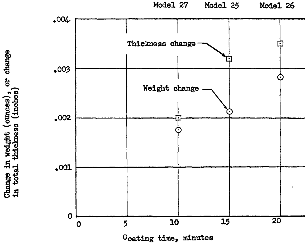
Figure 2.- Change in weight and thickness plotted against coating time.
