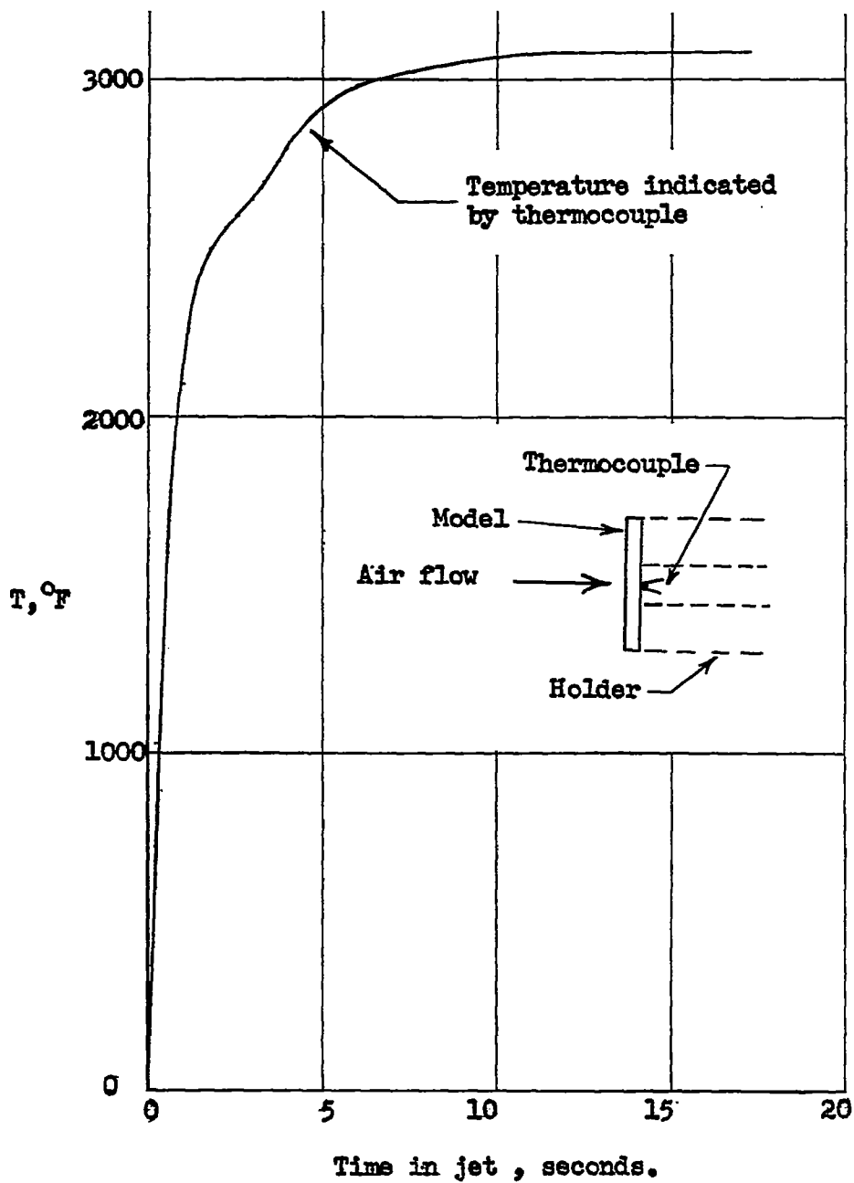
Figure 4.- Typical temperature time history of coated models.
