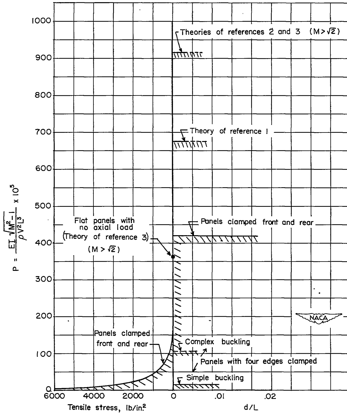
Figure 9.- Comparison of the critical values of the panel flutter parameter at M = 1.3 .
