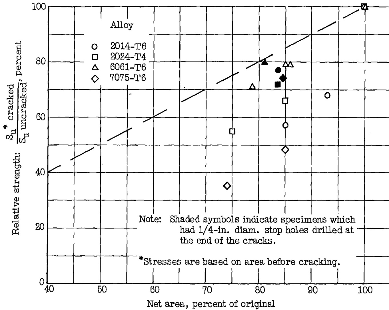
Figure 7.- Effect of fatigue crack on static strength of aluminum alloys.
