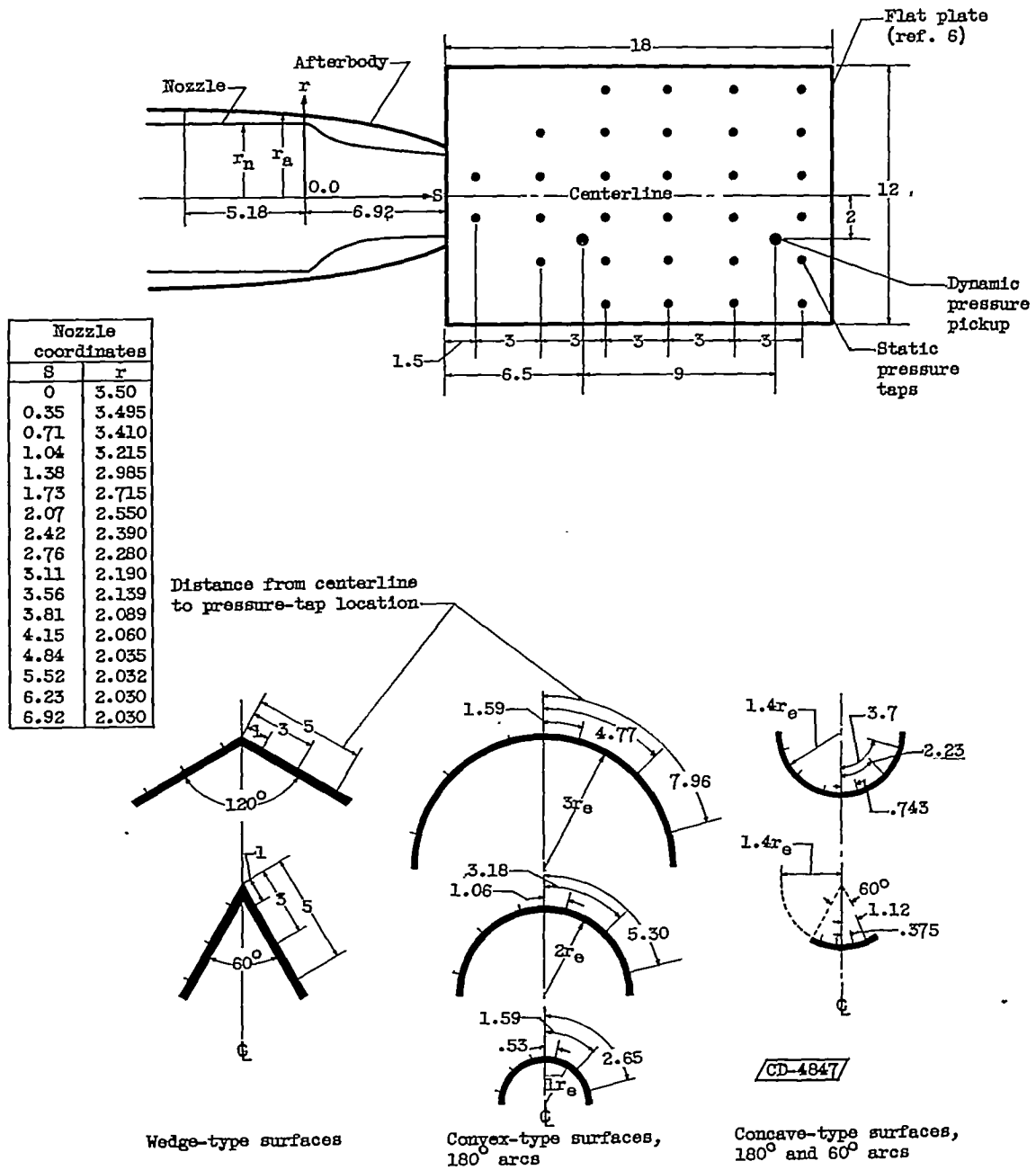
Figure 2. - Surface and boattail details (all dimensions in inches). Equation of parabolic afterbody: r_a = 4.125 - \frac{4.125}{(18)^2} (S \pm 5.18)^2 . Length for all surface types is 18 inches.
