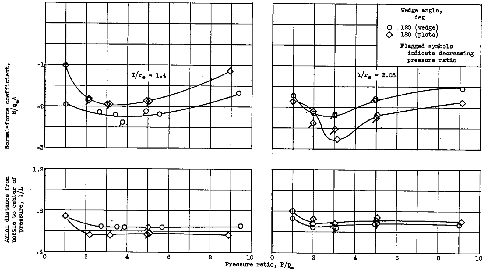
Figure 4. - Concluded. Results of varying wedge angle.
