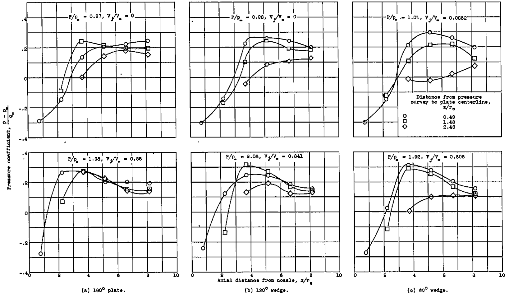
Figure 5. - Pressure profiles on wedge-type surfaces. Vertical distance between plate and nozzle, Y/r_0 , 2.03.
