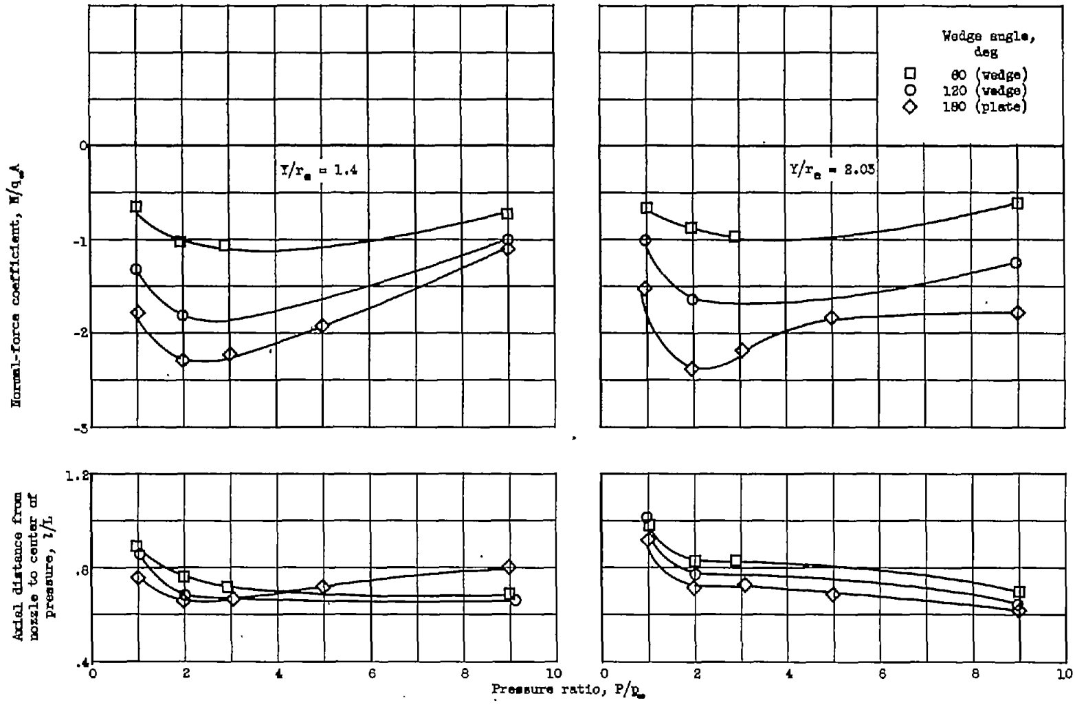
Figure 4. - Results of varying wedge angle.
