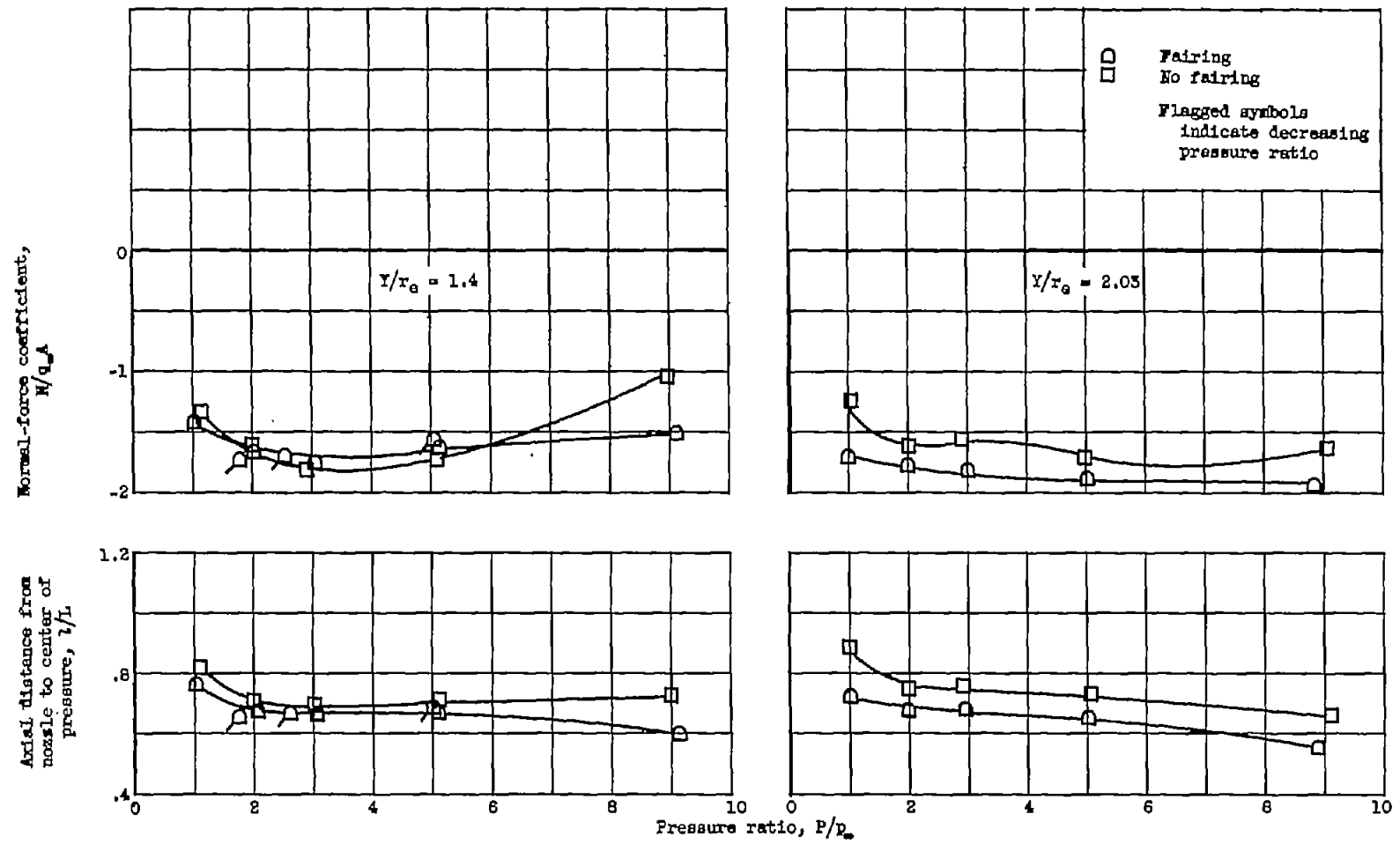
(b) With and without fairings. Radius of surface curvature, 2r_e .
