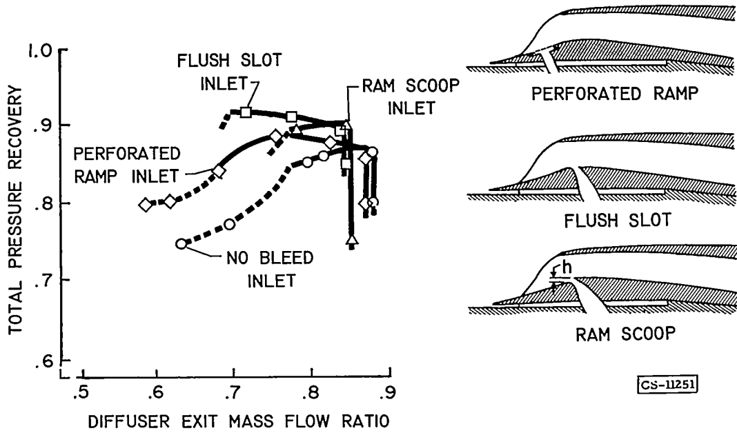
Figure 3. - Effect of throat bleed. Double ramp inlet; free-stream Mach number, 2.0; angle of attack, 0°.
