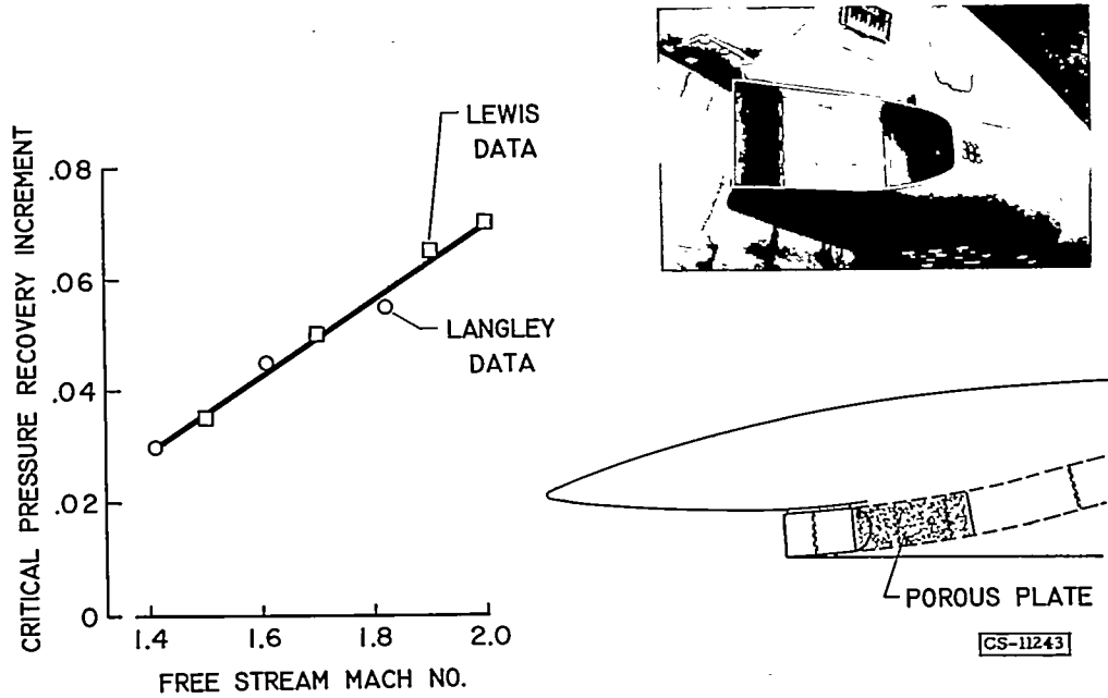
Figure 4. - Effectiveness of throat bleed with Mach number.
