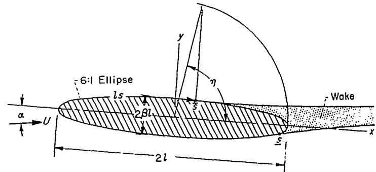
FIGURE 1.—Notation and coordinate system for elliptic airfoil at angle of attack.
