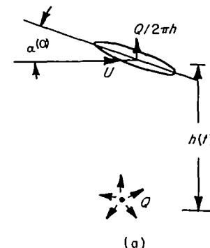
Sketch (a) Airfoil and source.
