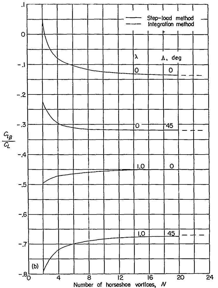
(b) Tapered wings, A=1.5 .
