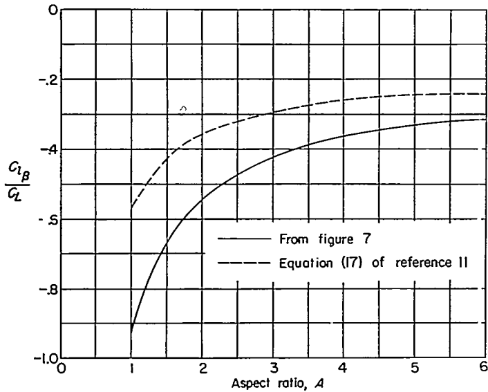
FIGURE 10.—Comparison of values of \frac{C_{iB}}{C_L} from figure 7 with theoretical values from reference 11. \Delta = 45^\circ ; \lambda = 1.00 .
