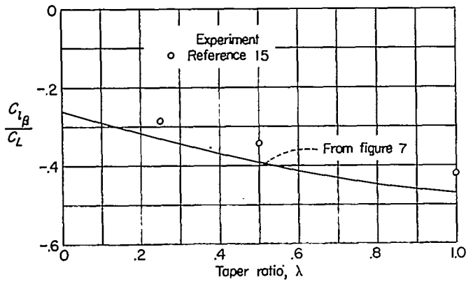
FIGURE 12.—Comparison of experimental and calculated effect of \lambda on \frac{C_{i\beta}}{C_L} . A=2.61 ; \Lambda=45^\circ .
