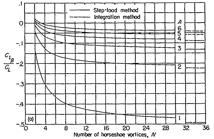
(a) Elliptic wings. FIGURE 13.—Effect of N on estimated value of \frac{C_{i\beta}}{C_L} .
