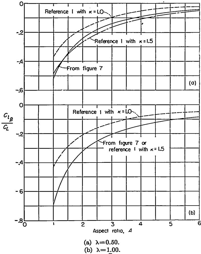
FIGURE 9.—Comparison of values of \frac{C_{iB}}{C_L} from figure 7 with theoretical values from reference 1. \Delta = 0^\circ .
