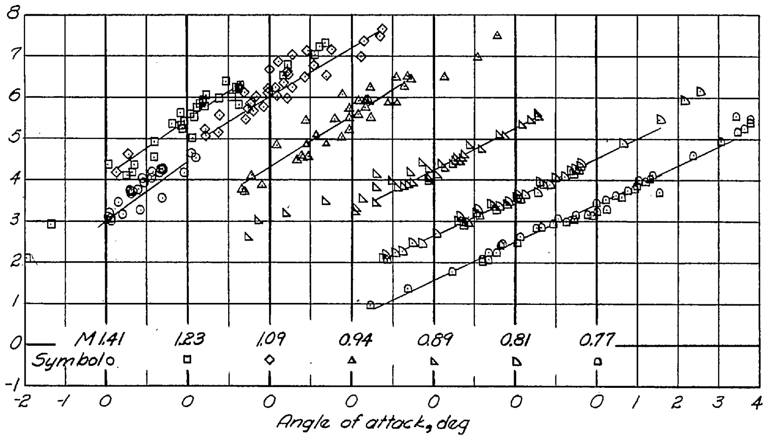
Figure 14.- Variation of downflow angle with angle of attack at several Mach numbers for the symmetric model.
