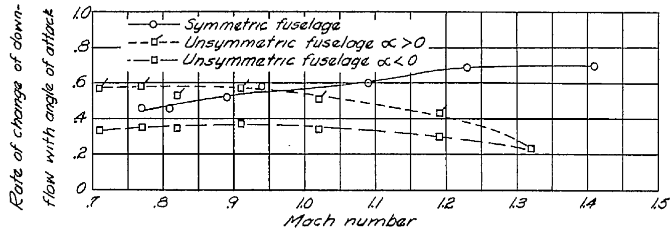
(a) Slope of downflow with angle of attack.
