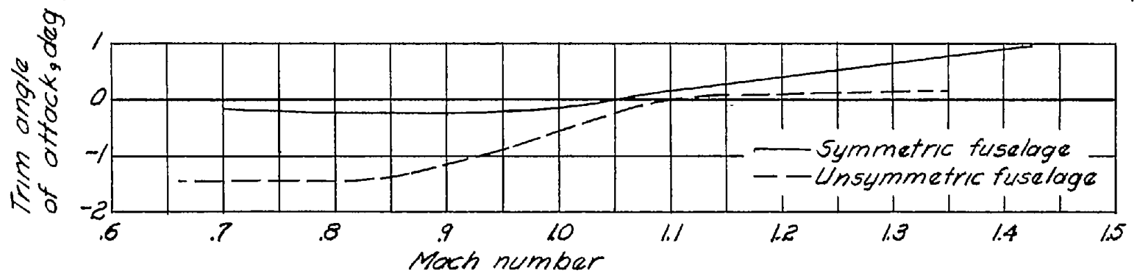
(b) Variations of trim angles of attack.
