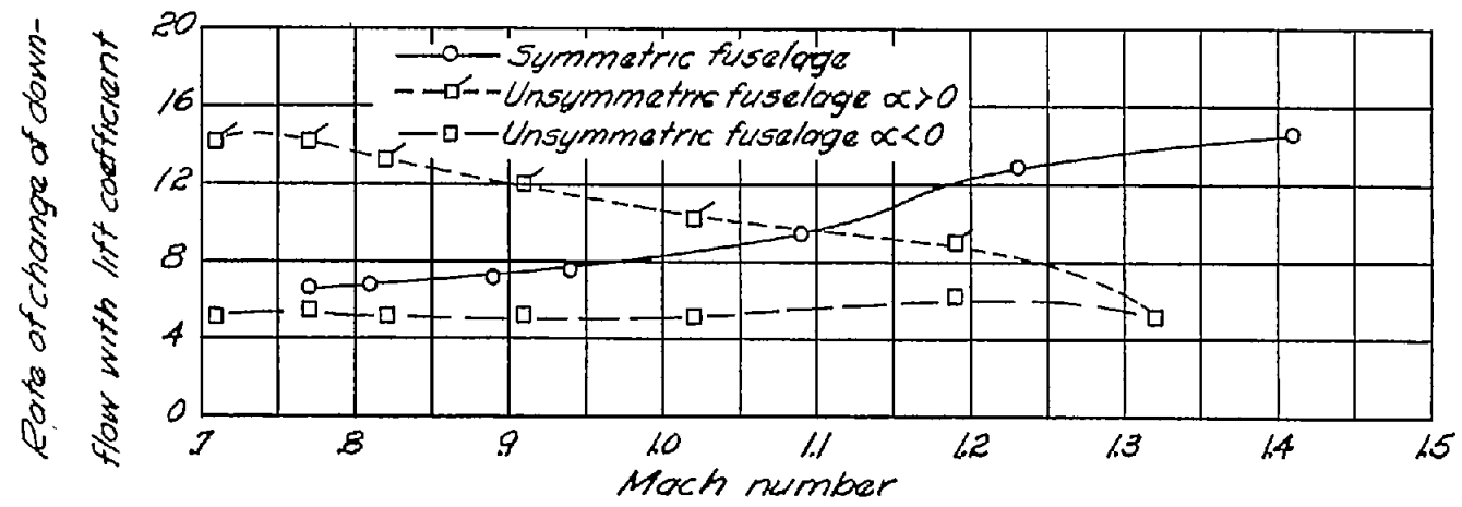
(b) Slope of downflow with lift coefficient.
