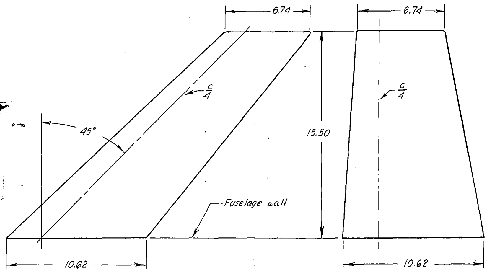
(a) Models 1 to 6. \Lambda = 45^\circ .
