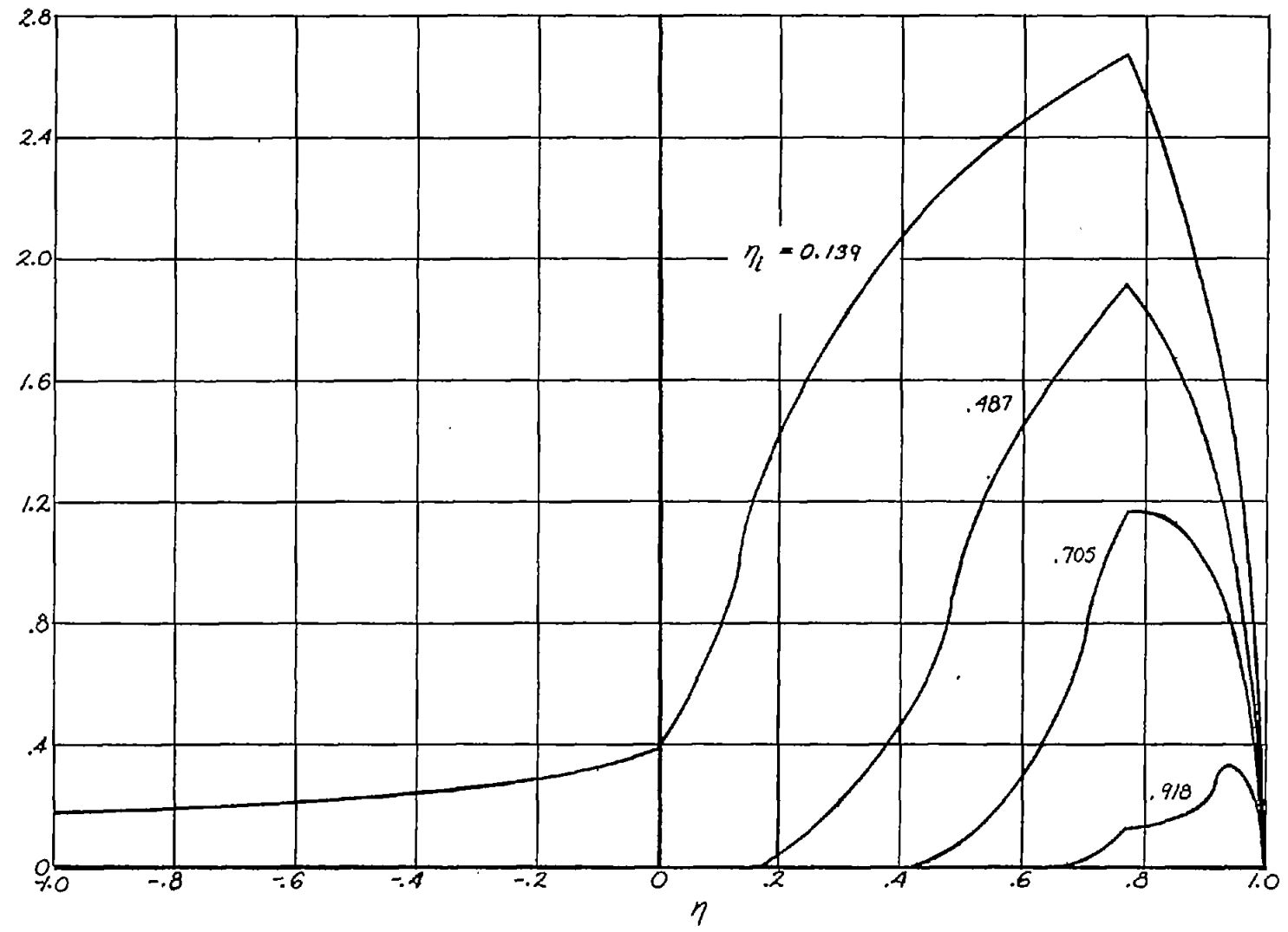
Figure 12.- Span load distribution for models tested. \beta_m = 0.765 .
