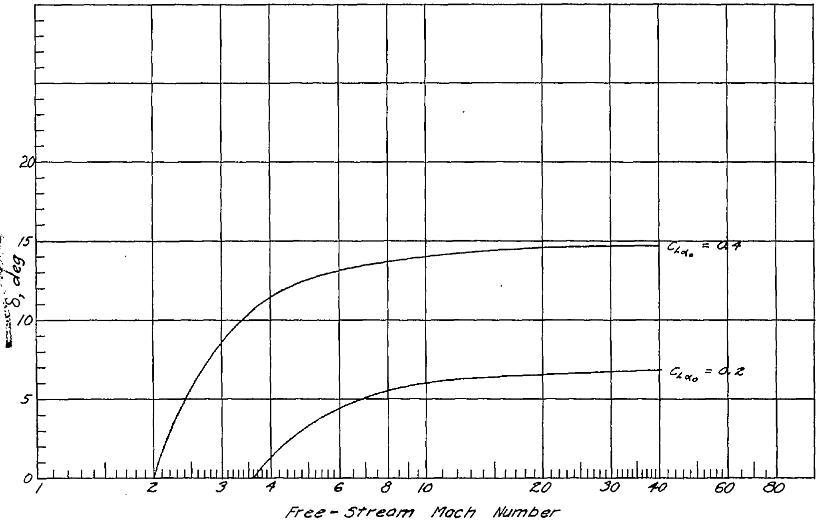
Figure 6.- Variation of wedge half angle with Mach number for two lift-curve slopes.
