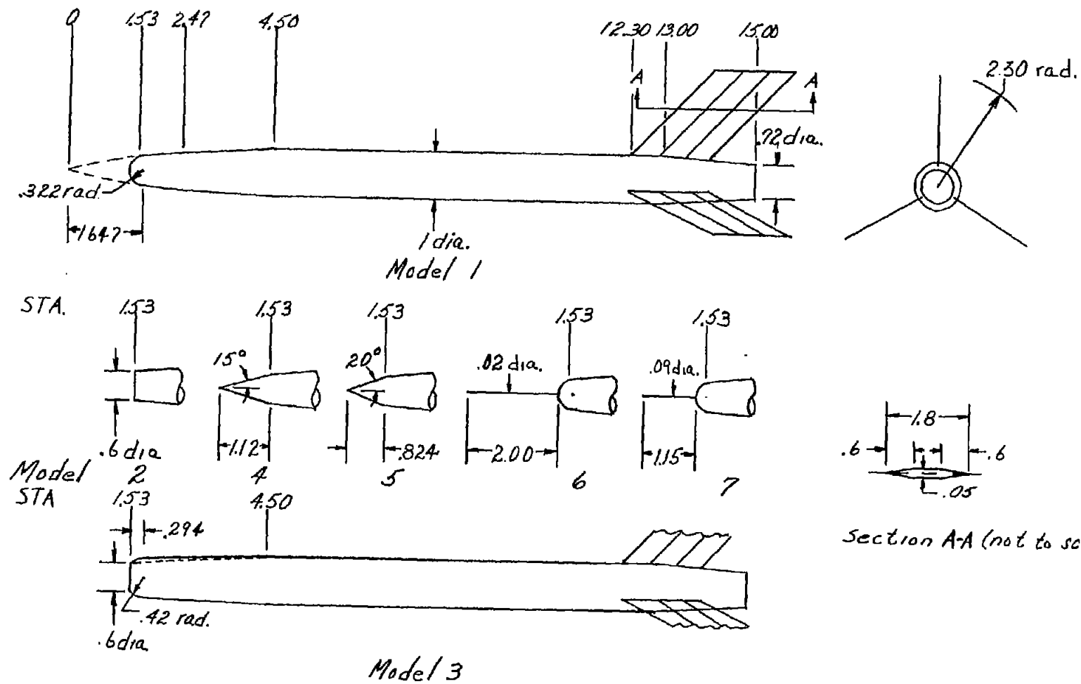
Figure 1.- Sketch of models tested.
