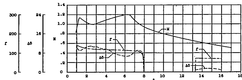
(c) Model 3; \frac{t}{c} = 0.09 ; \Lambda = 35^\circ .
