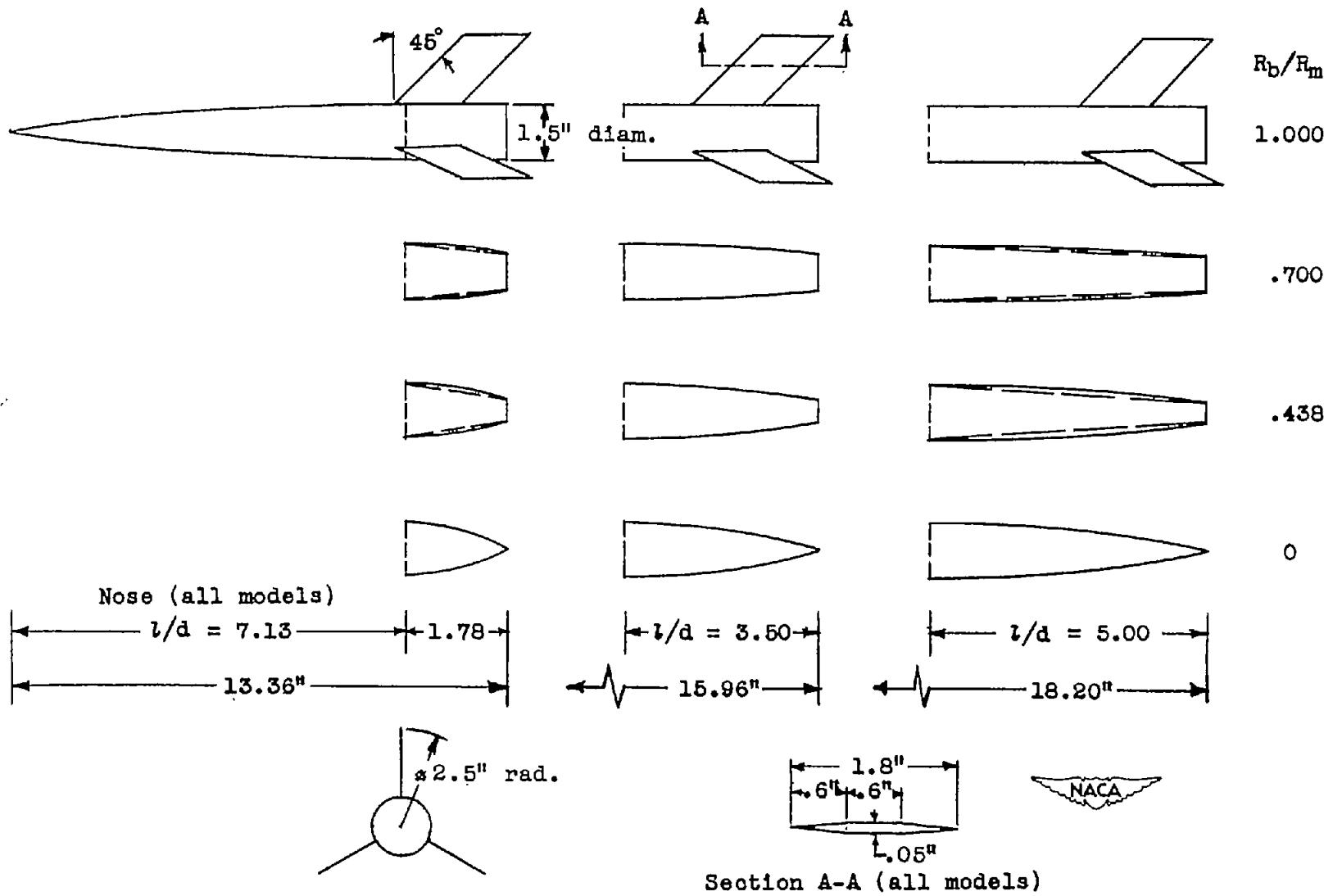
Figure 1.- Test configurations.
