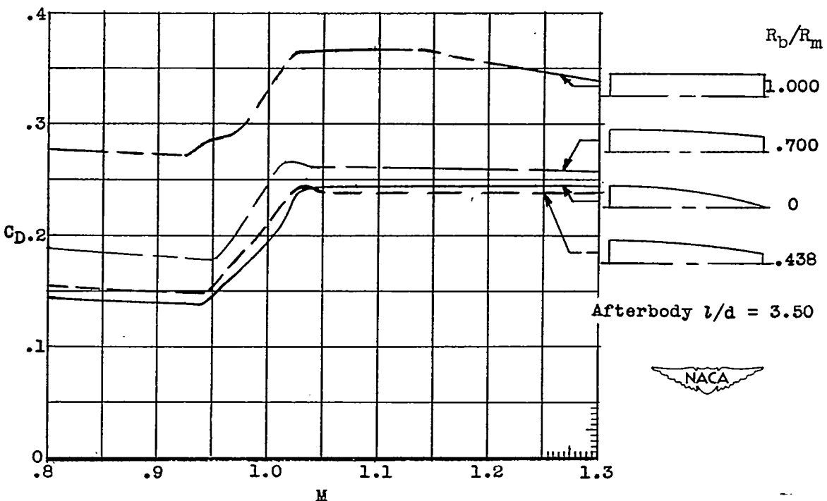
Figure 3.- Total-configuration drag coefficients of parabolic afterbodies.
