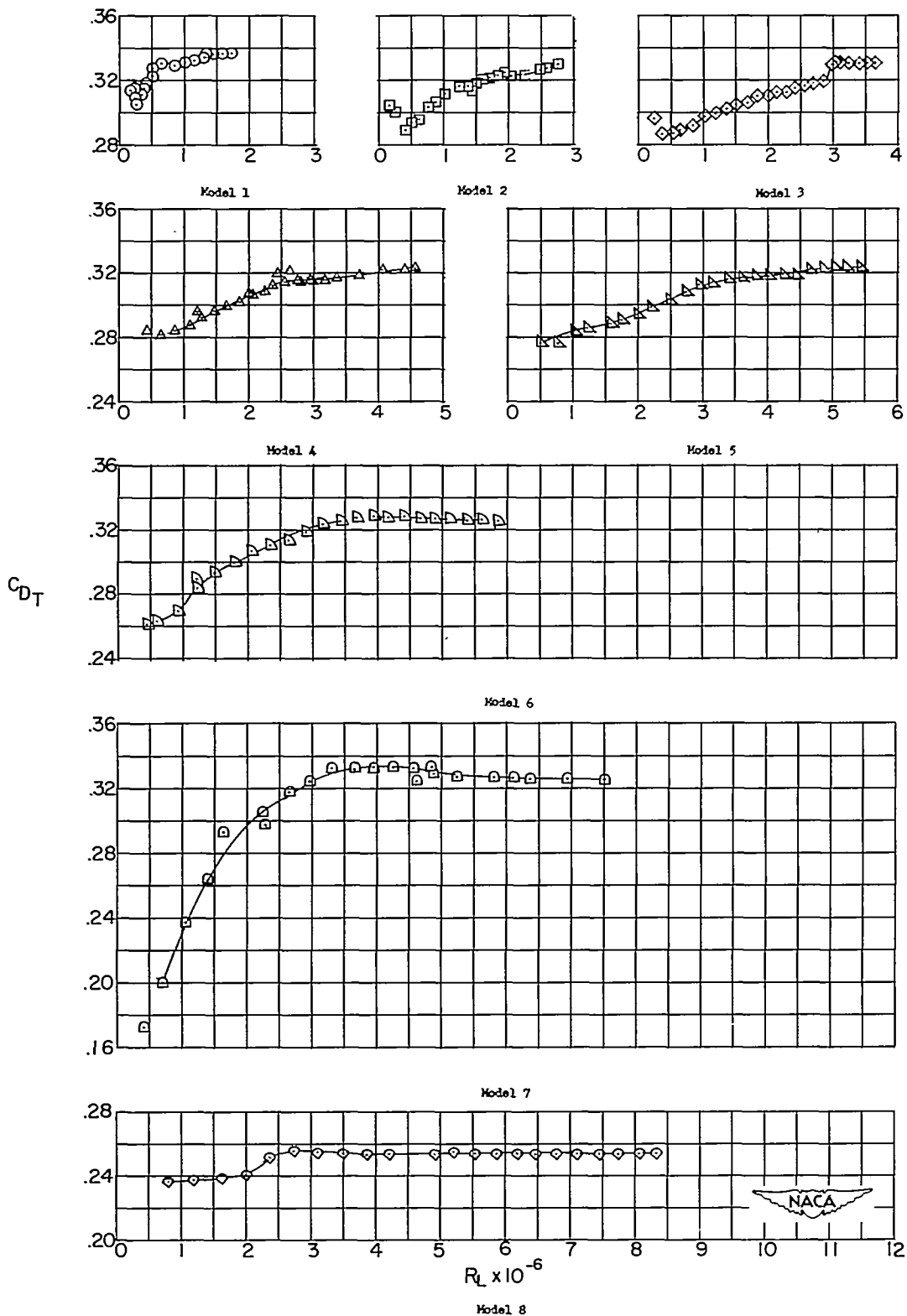
Figure 3.- Variation of total-drag coefficient with Reynolds number at M = 2.41 .
