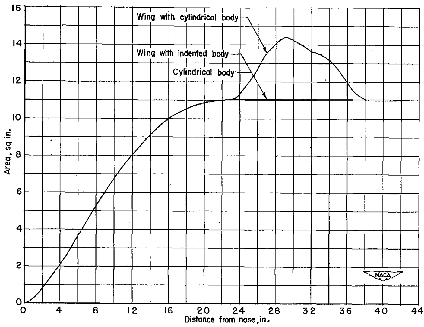
Figure 2.- Cross-sectional areas of models.
