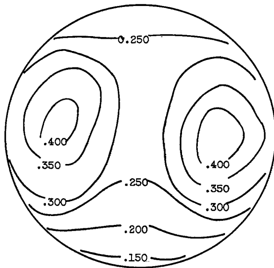
(f) \theta_1, 44.7^\circ ; \alpha, 10^\circ ; cone deflection, 10^\circ ; super-critical pressure recovery.
