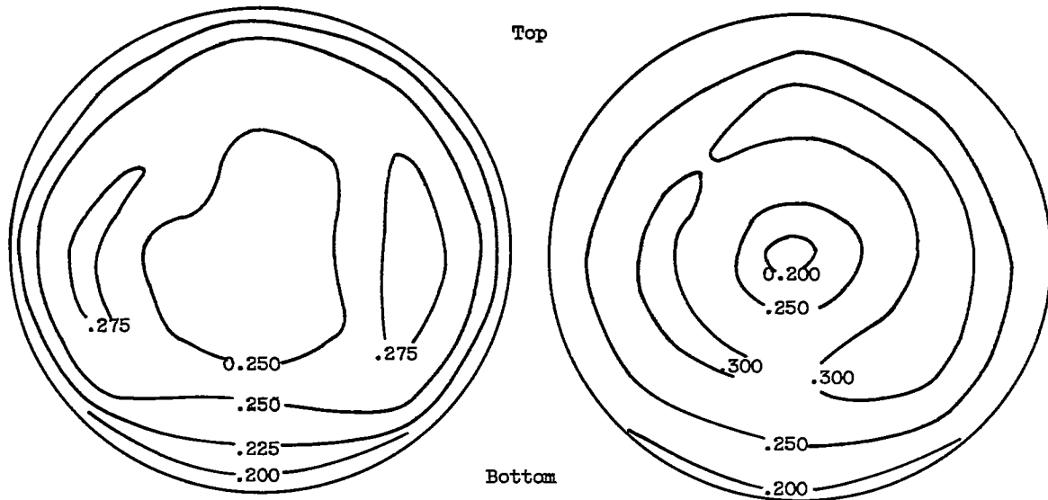
(a) \theta_1, 41.8^\circ ; \alpha, 0^\circ ; cone deflection, 0^\circ ; critical pressure recovery.
