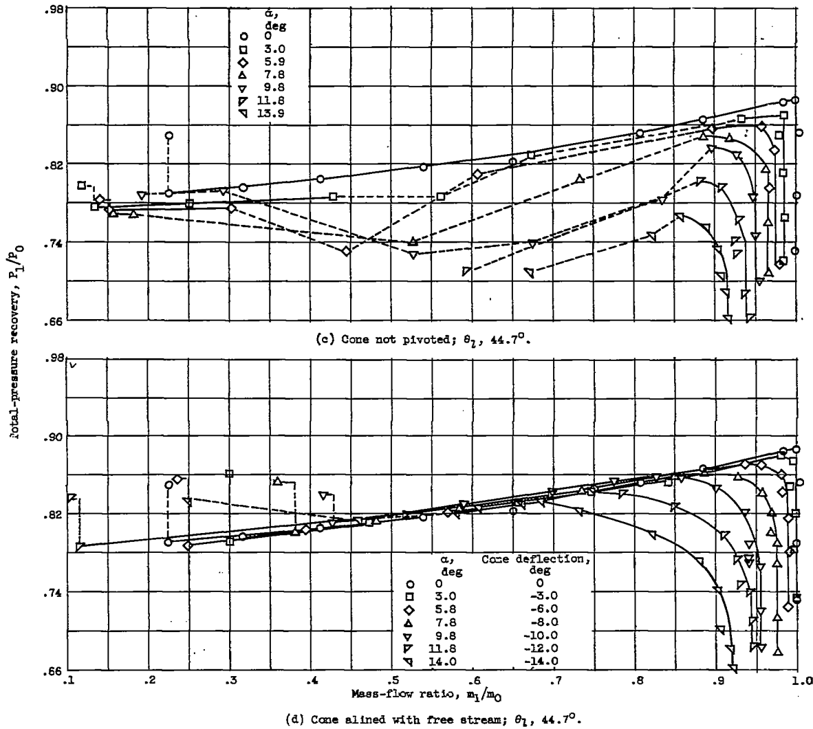
Figure 5. - Concluded. Effect of aligning cone with free stream on diffuser performance at angle of attack.
