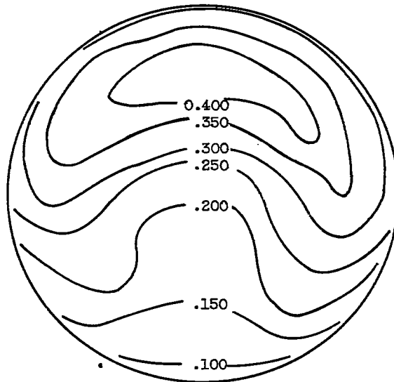
(c) \theta_1, 44.7^\circ ; \alpha, 6^\circ ; cone deflection, 6^\circ ; critical pressure recovery.
