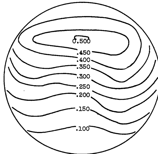
(e) \theta_1, 44.7^\circ ; \alpha, 10^\circ ; cone deflection, 0^\circ ; critical pressure recovery.
