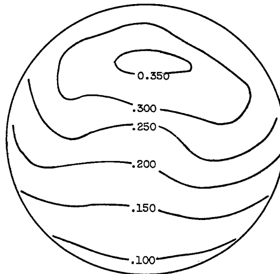
(g) \theta_1, 44.7^\circ ; \alpha, 10^\circ ; cone deflection, 10^\circ ; peak pressure recovery.
