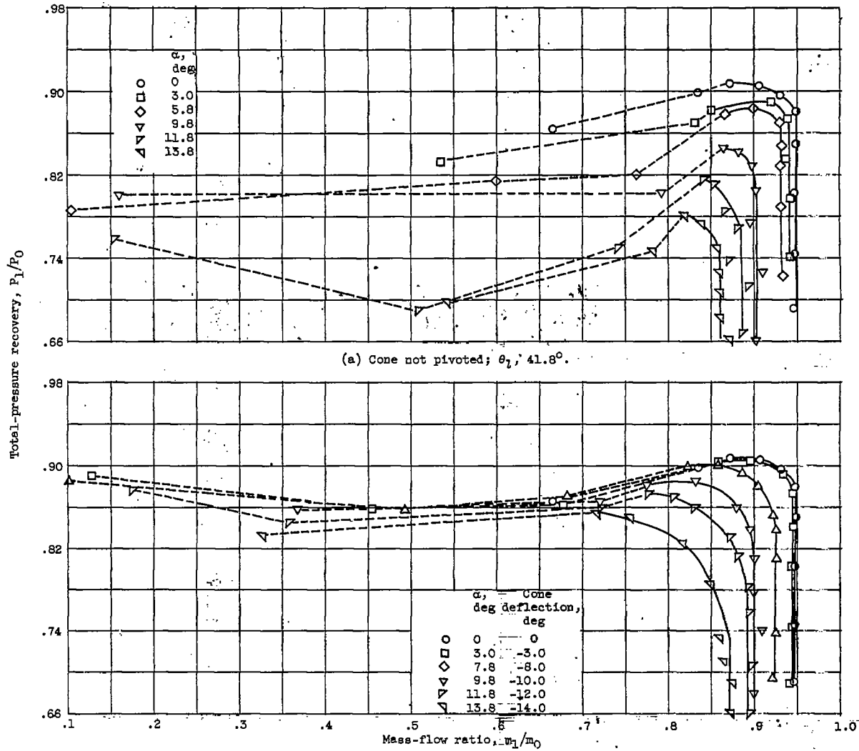
Figure 5. - Effect of slining cone with free stream on diffuser performance at angle of attack.
