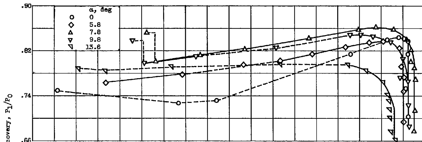
(c) Cone deflection, -6^\circ .
