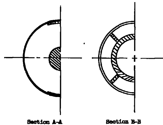
Figure 1. - Schematic diagram showing principal dimensions of model.
