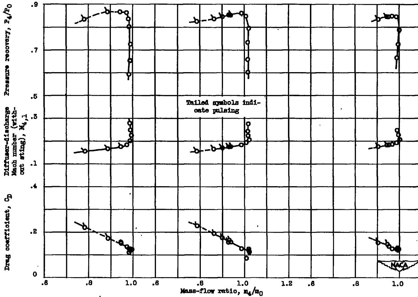
(a) Upstream spike position; model 25-42-12.
