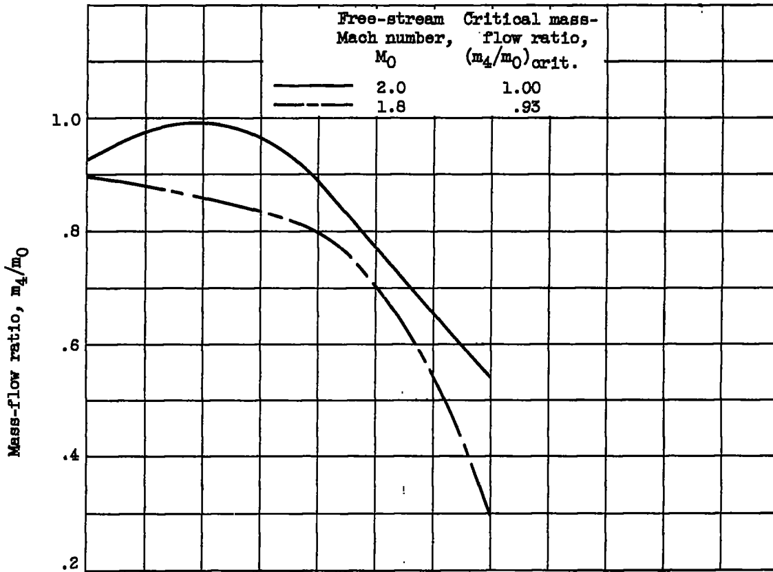
(a) Minimum stable mass-flow ratio.
