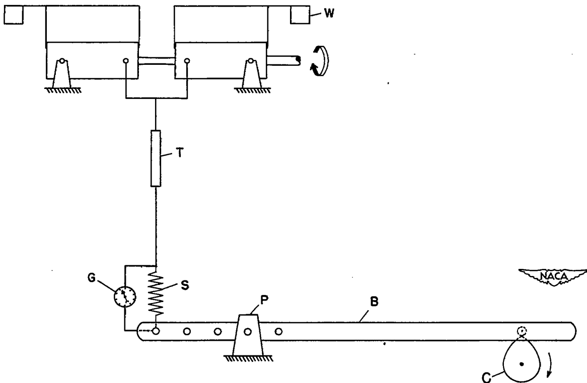
Figure 2.- Loading device for rotating-beam tests in which the amplitude varies continuously.
