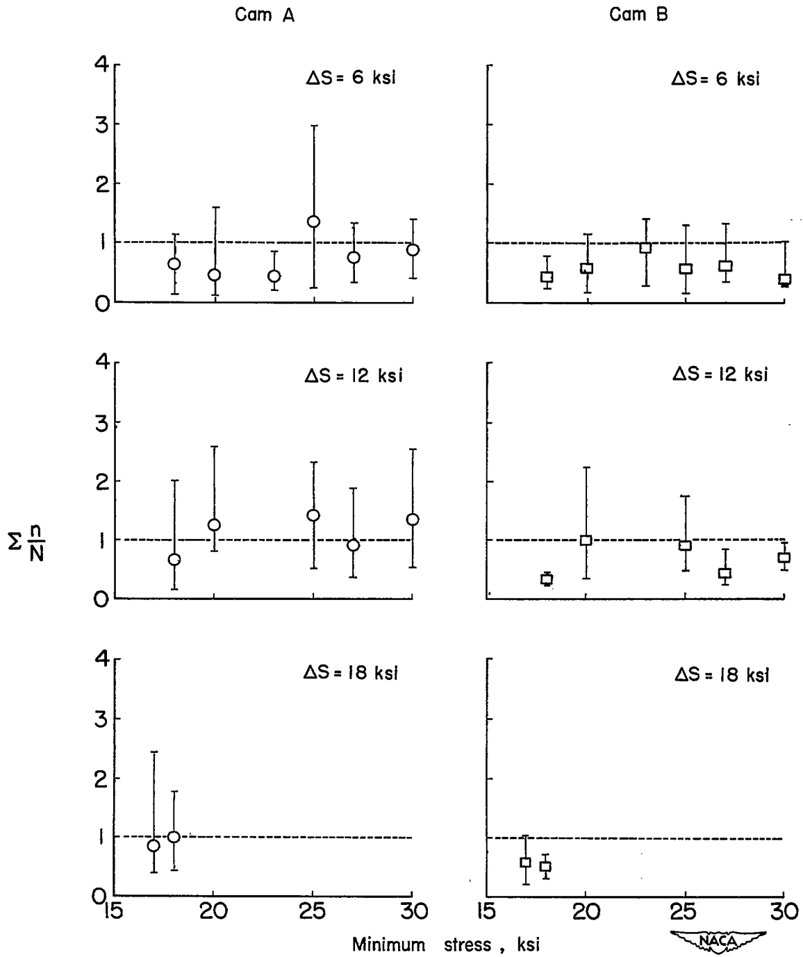
Figure 5.- \sum \frac{n}{N} for tests with variable stress amplitude.
