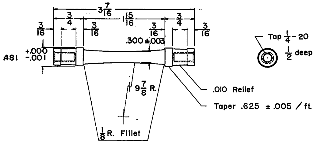
Figure 1.- Rotating-beam specimen.
