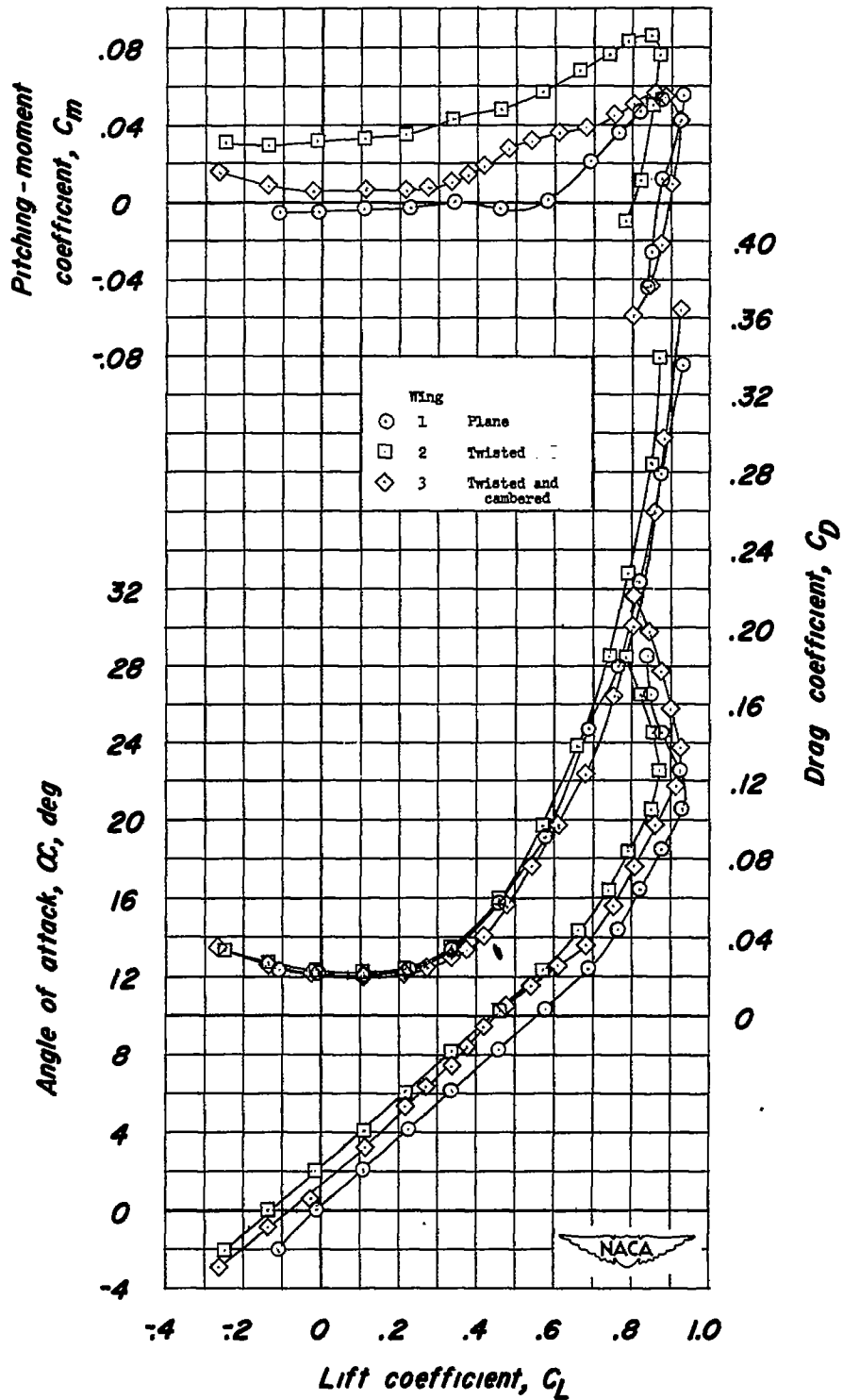
Figure 7.- Effects of twist and camber on variation of C_m , C_D , and \alpha with C_L for a 45^\circ sweptback wing of aspect ratio 4 and taper ratio 0.6. Reynolds number = 0.895 \times 10^6 ; Mach number = 0.17; transition strips on.
