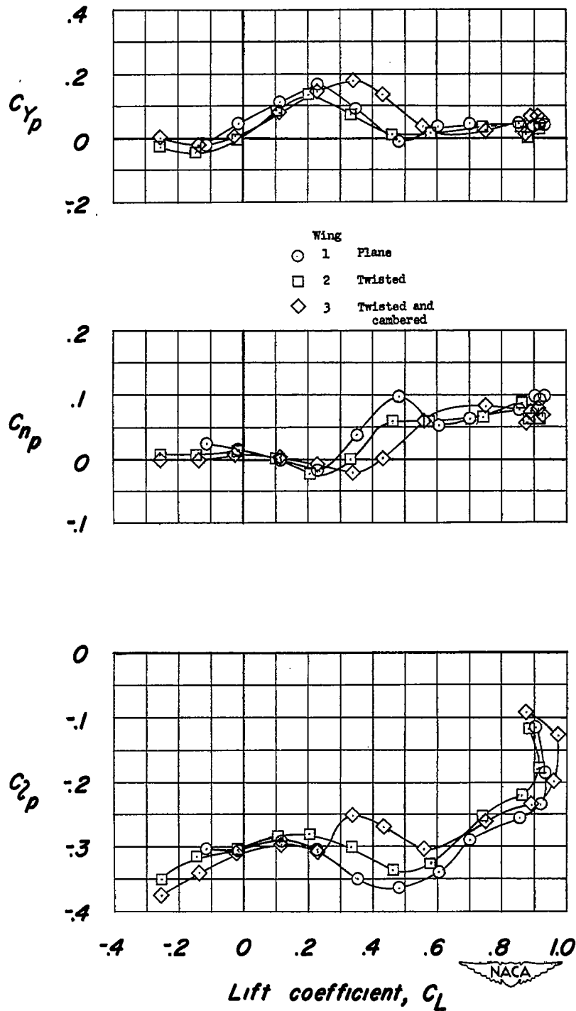
Figure 11.- Effects of twist and camber on variation of C_{y_p} , C_{n_p} , and C_{l_p} with C_L for a 45^\circ sweptback wing of aspect ratio 4 and taper ratio 0.6. Reynolds number = 0.895 \times 10^6 ; Mach number = 0.17; transition strips off.
