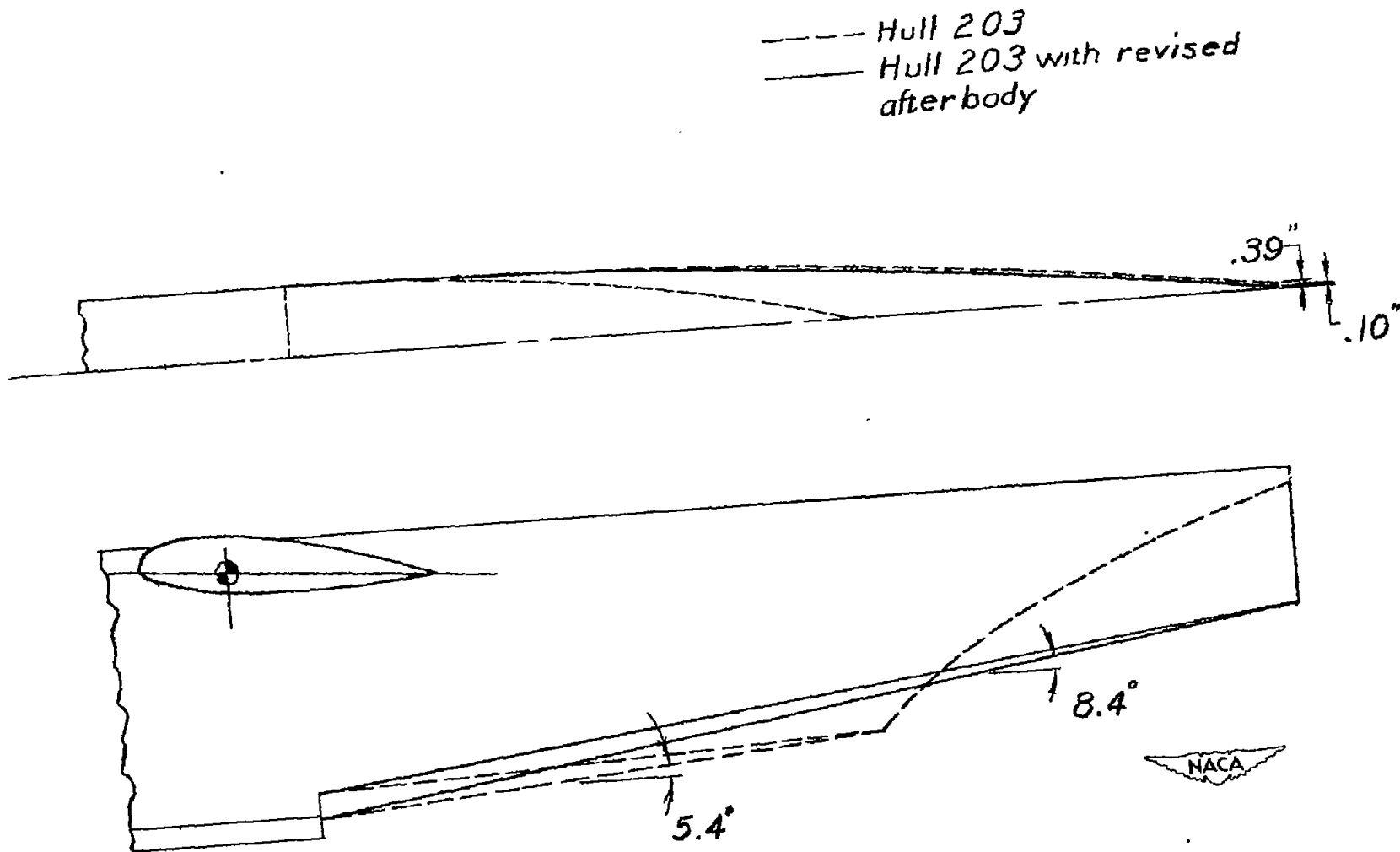
Figure 5.- Revisions to Langley tank model 203 afterbody.
