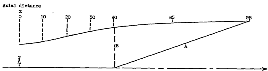
Figure 5. - Unsymmetric circular inlet or nozzle for Mach number of 2.98.
