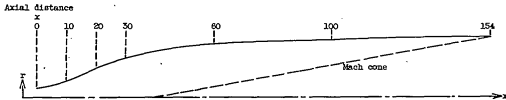
Figure 4. - Square nozzle for Mach number of 5.70.
