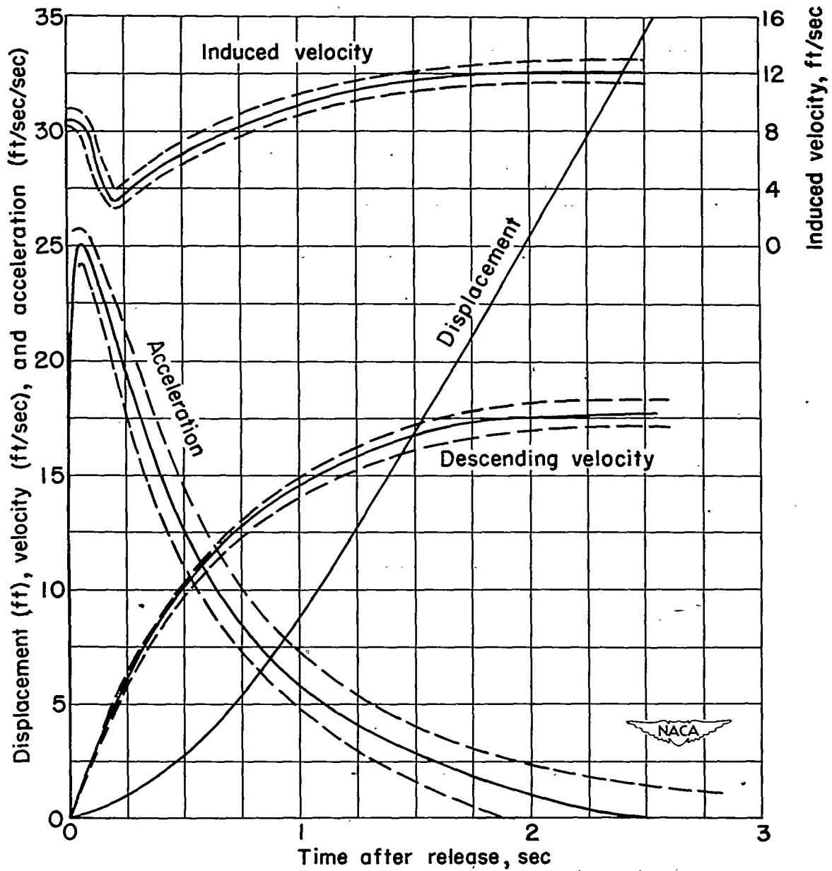
Figure 6.- Calculated limits of accuracy of velocity, acceleration, and induced-velocity curves worked out for a sample case. w = 0.2 ;
