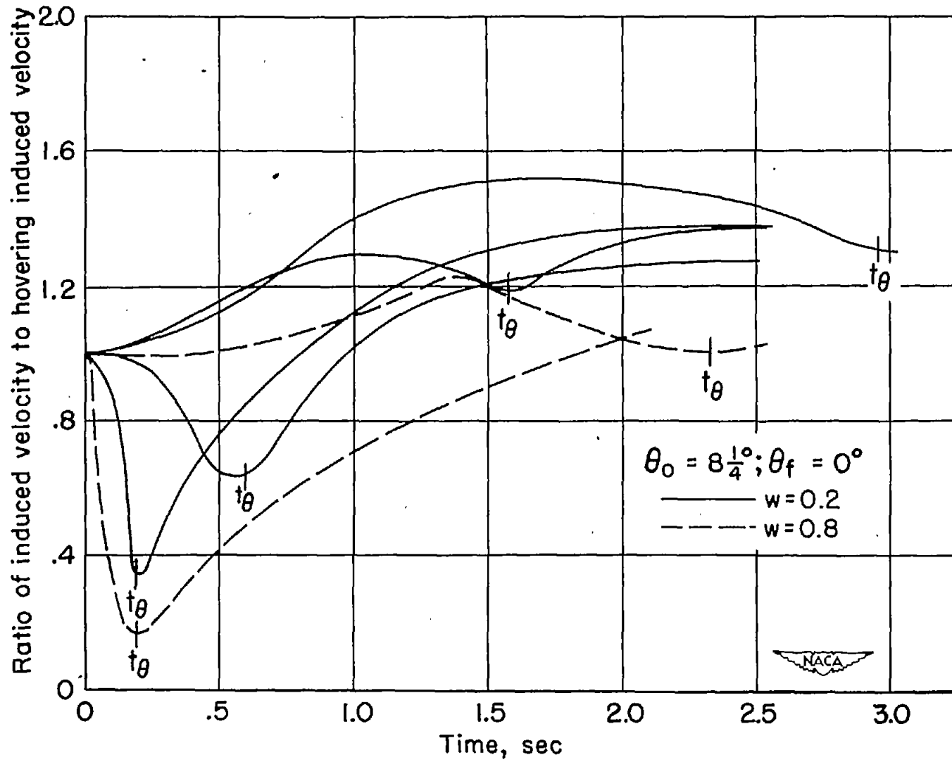
Figure 9.- Effect of variation in t_\theta on induced-velocity ratio for the 6-foot model.
