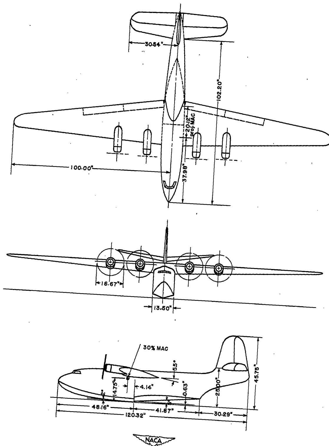
Figure 4.- General arrangement of the conventional-hull model.
