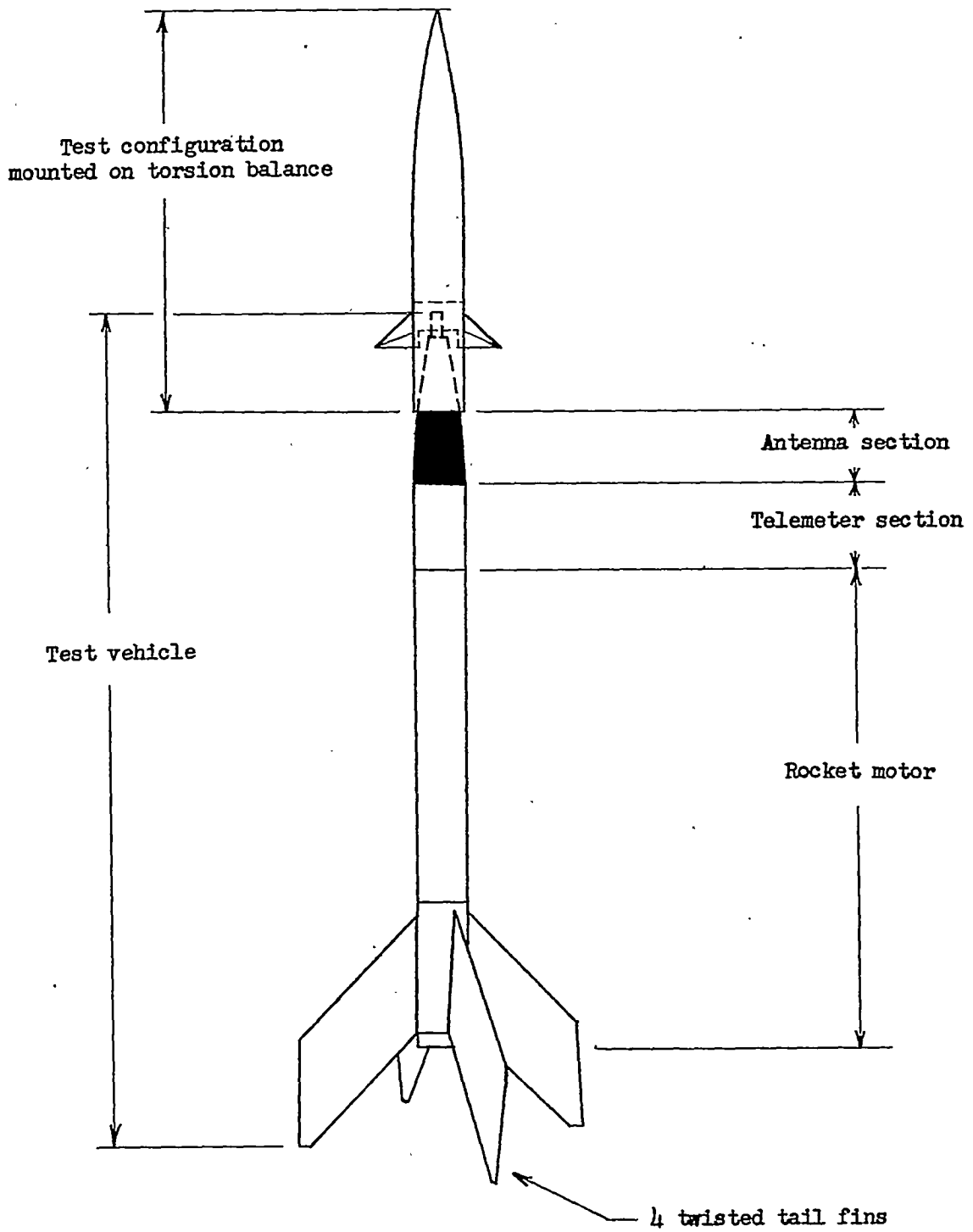
Figure 3.- Test configuration mounted on test vehicle.
