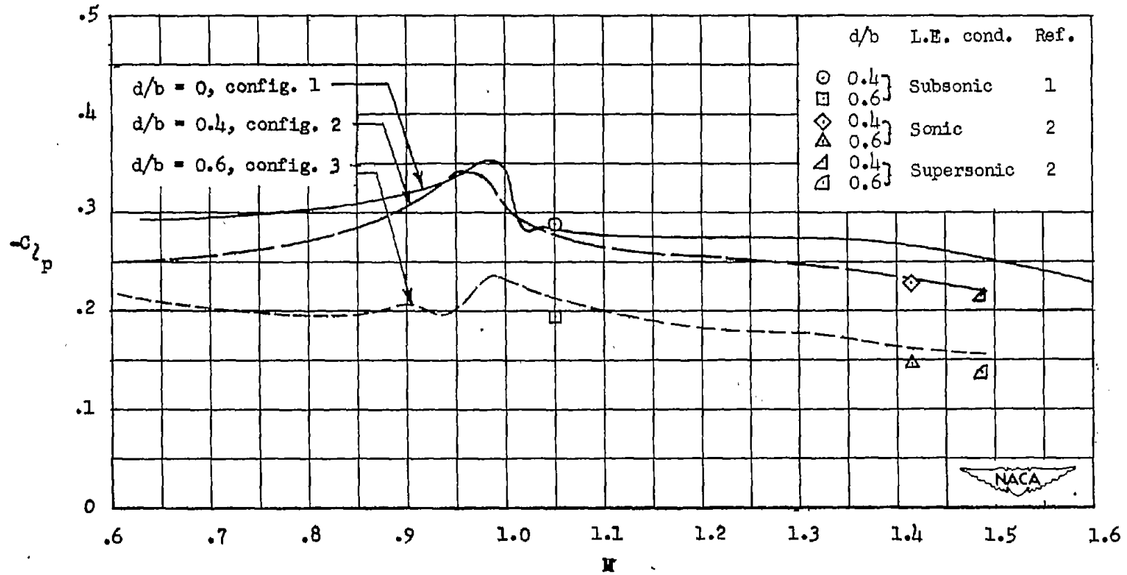
Figure 4.- Effect of fuselage-diameter - wing-span ratio on the variation of the damping-in-roll coefficient with Mach number.
