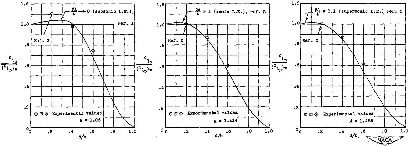
(a) Subsonic wing leading edges. (b) Sonic wing leading edges. (c) Supersonic wing leading edges.
