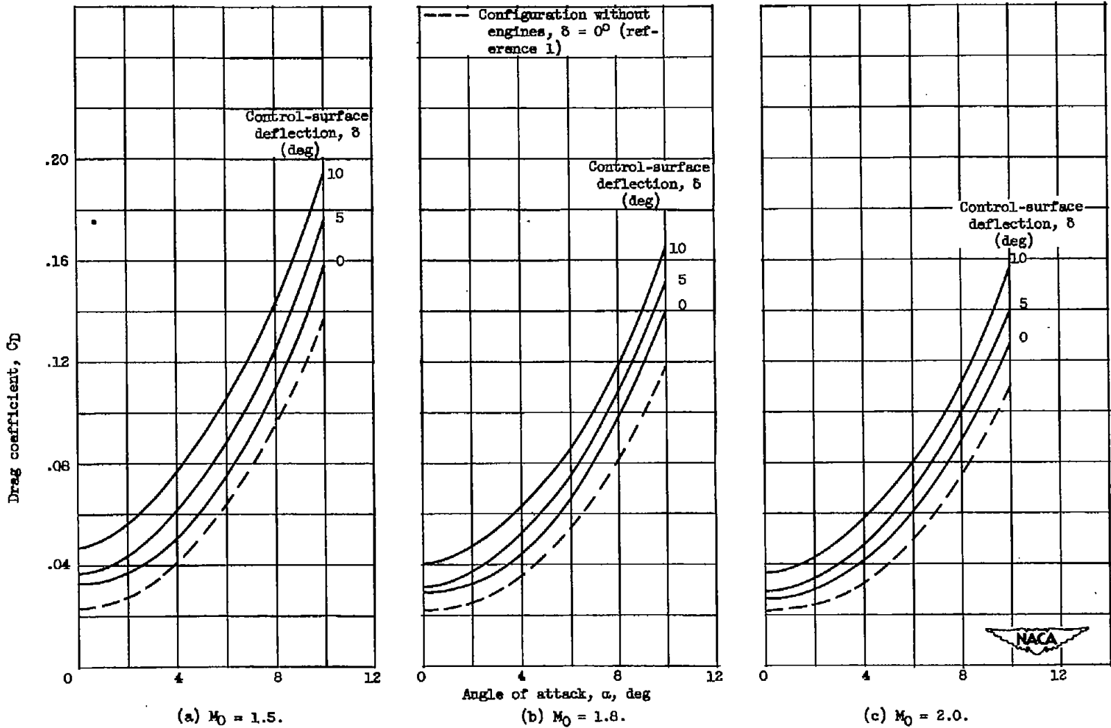
Figure 6. - Variation of configuration drag coefficient with angle of attack for several control-surface deflections and three Mach numbers. (Supercritical inlet operation.)
