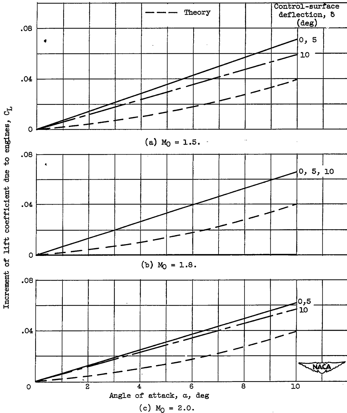
Figure 10. - Variation of increment of lift coefficient due to engines with angle of attack for several control-surface deflections and three Mach numbers. (Supercritical inlet operation.)
