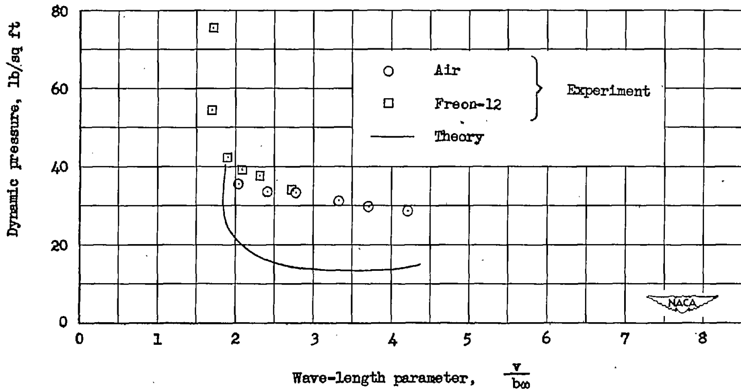
Figure 14.- Dynamic pressure at flutter plotted against wave-length parameter v/b\infty for model 17-32-3.
