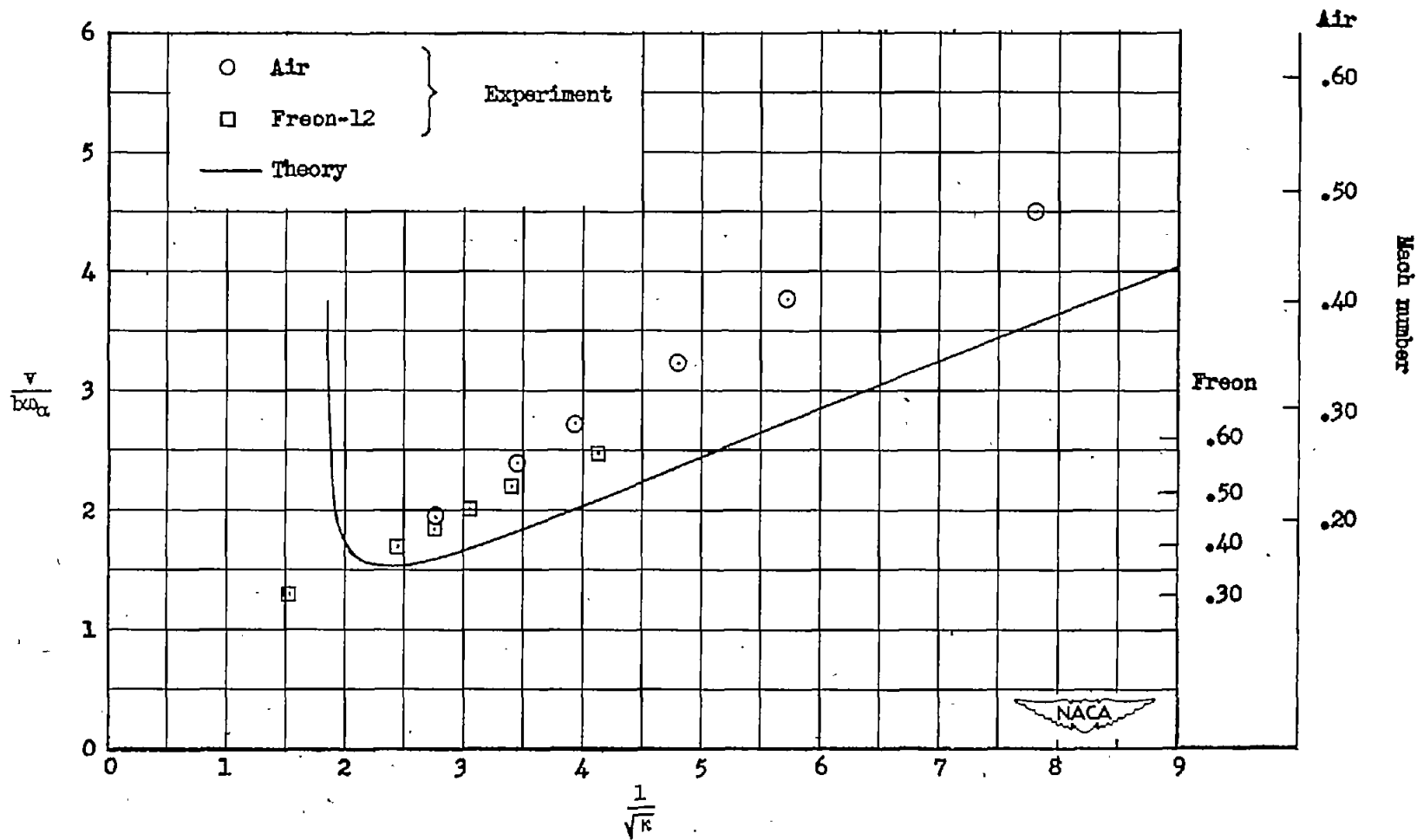
Figure 6.- Variation of flutter-speed coefficient v/bu_\alpha with the relative-density parameter 1/\sqrt{\kappa} for model 27-38-3.
