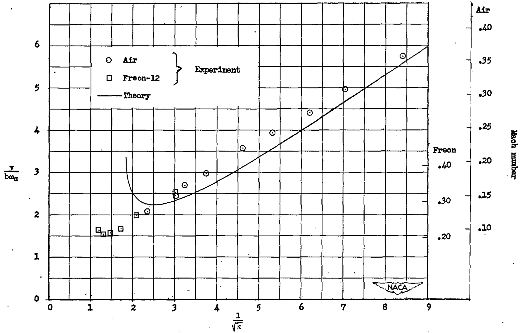
Figure 2.- Variation of flutter-speed coefficient v/b\omega\alpha with the relative-density parameter 1/\sqrt{K} for model 17-32-4.
