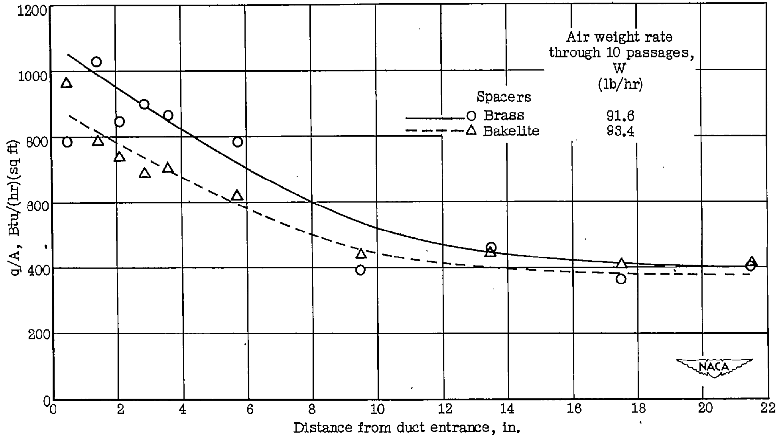
Figure 7.- Effect of thermal resistance between inner and outer skins of rectangular ducts.
