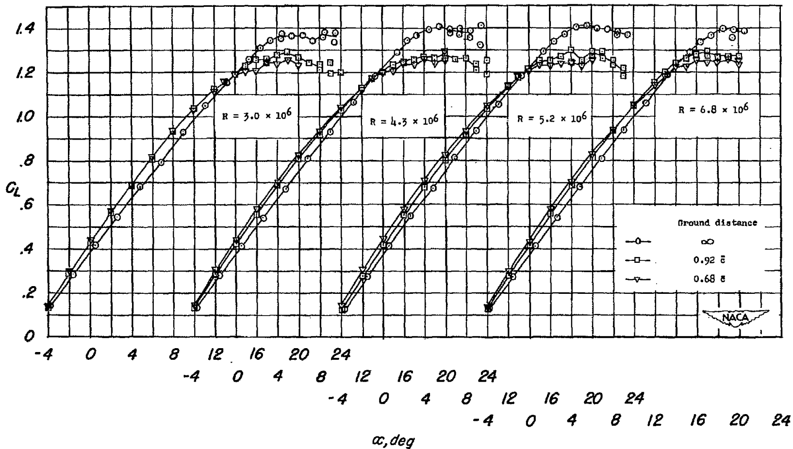
(a) Lift.
