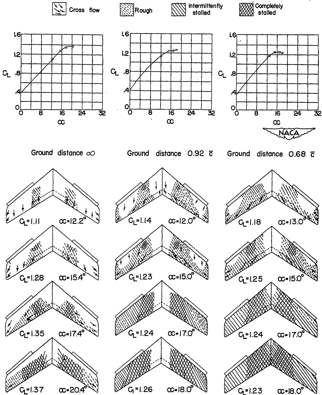
Figure 8.- Effect of ground on the stalling characteristics of a 42° sweptback wing. Reynolds number = 6.8 \times 10^6 ; flaps deflected.
