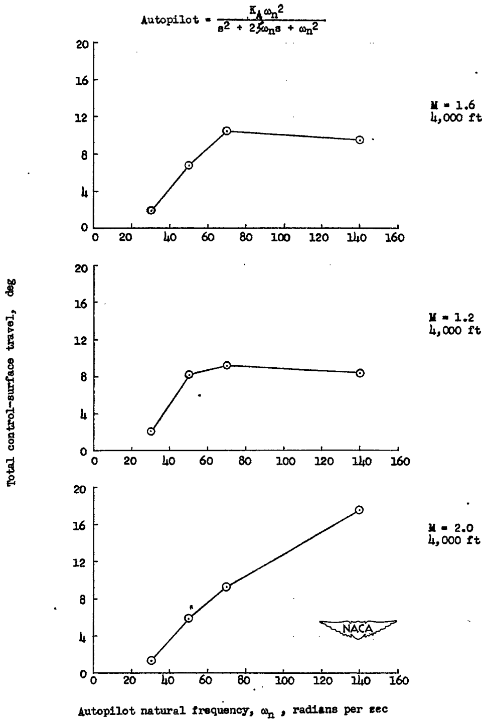
Figure 17.- Plot of total \delta travel against autopilot natural frequency in response to a step input \theta_1 . Static margin, 0.0948 at M = 1.6 ; \zeta of autopilot, 0.5.
