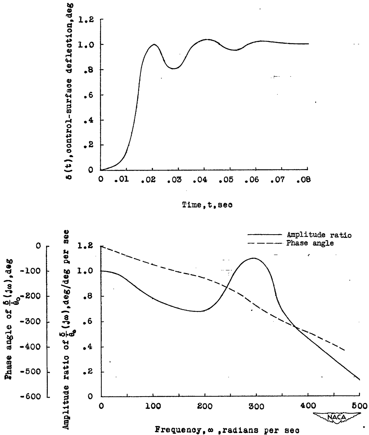
Figure 3.- Experimental transient response of the rate gyro and servo combination to a unit step, \dot{\theta}_0 , and the frequency response determined from this transient by Fourier series.
