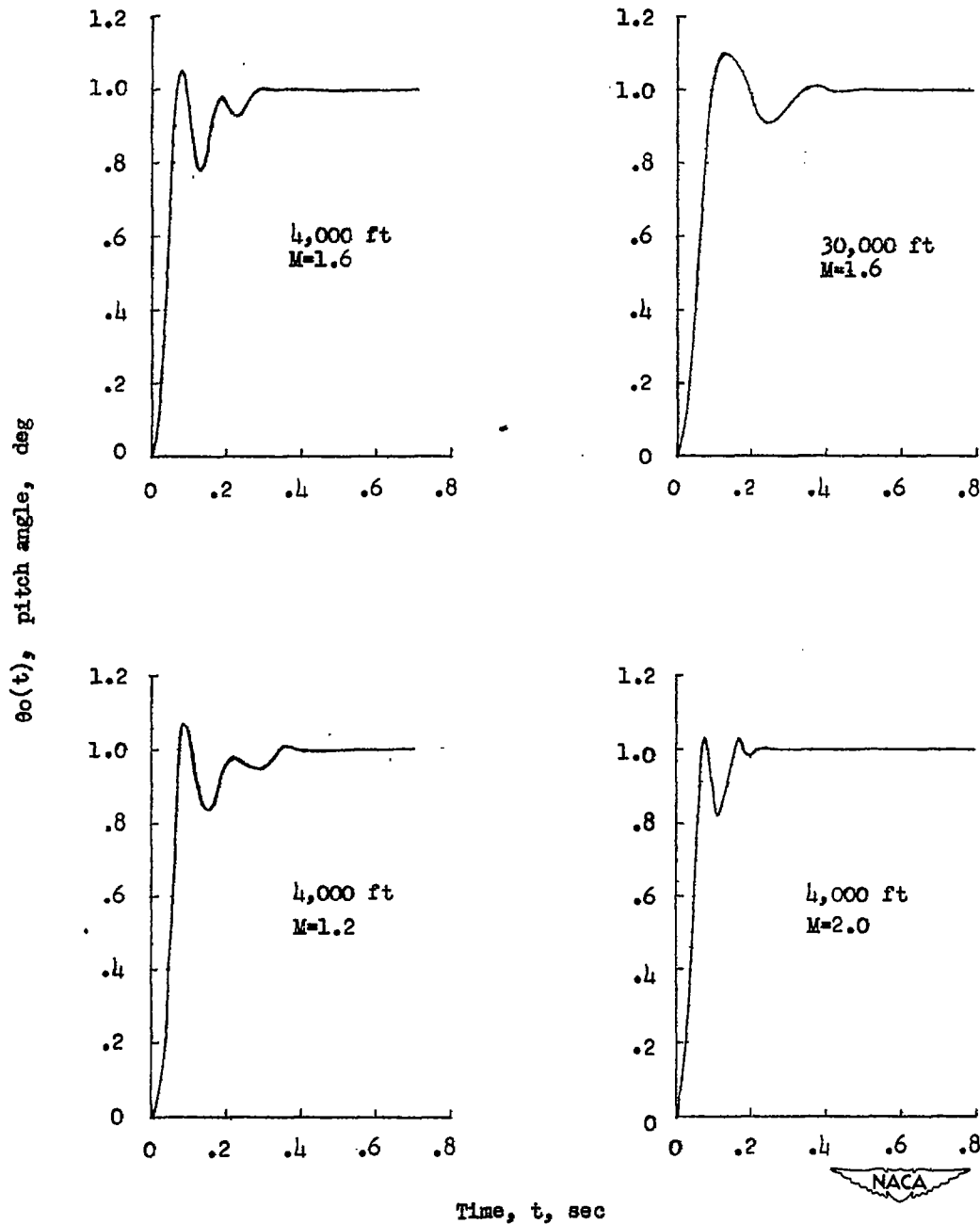
Figure 7.- Longitudinal transient responses \theta_0(t) of the missile to a unit step input signal calling for a change in attitude of 1^\circ . Static margin, 0.0945 at M = 1.6 ; K_T = 0.13 ; K_A = 2.43 .
