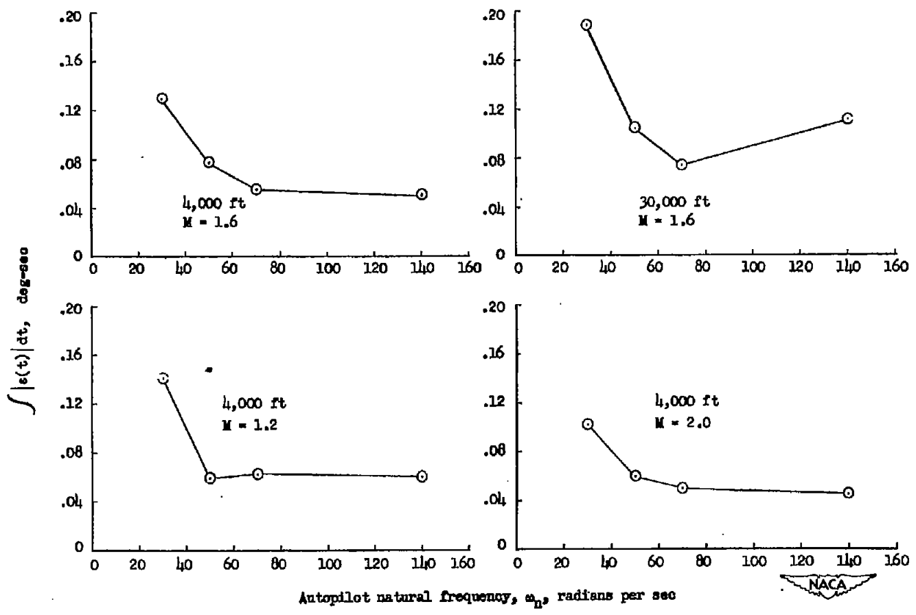
Figure 10.- Plot of \int |\epsilon(t)| dt for the rate-damped airframe and autopilot combination against autopilot natural frequency in response to a step \theta_1 . Static margin, 0.094c at M = 1.6; \zeta of autopilot, 0.5.
