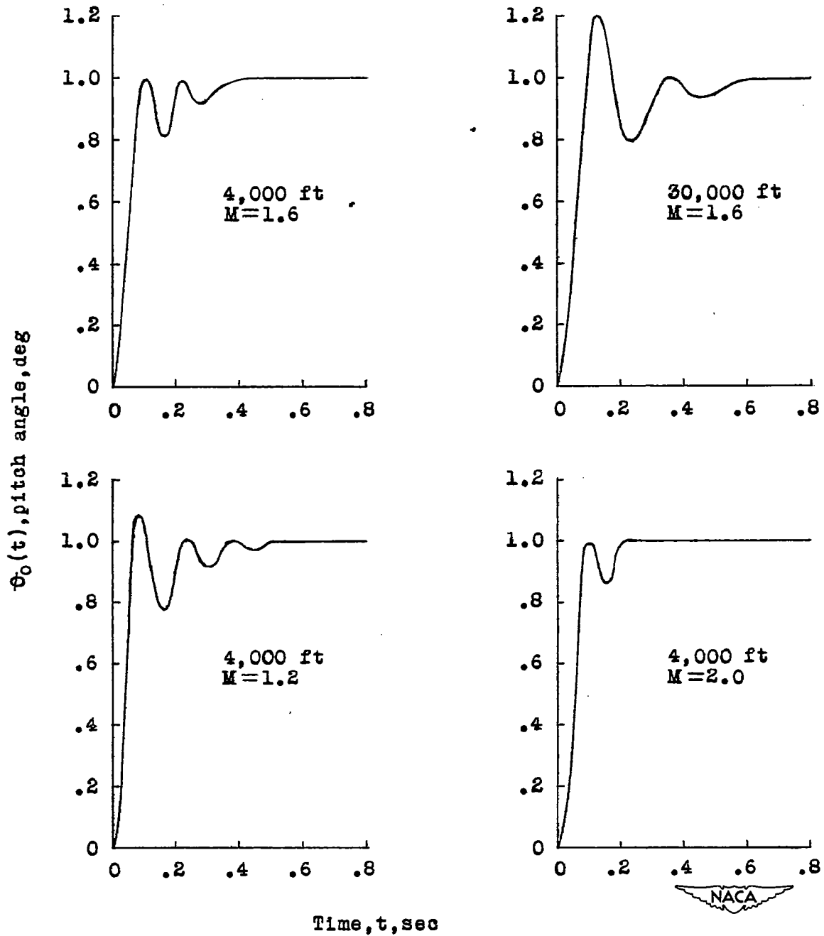
Figure 6.- Longitudinal transient responses \theta_0(t) of the missile to a unit step input signal calling for a change in attitude of 1^\circ . Static margin, 0.094c at M = 1.6 ; K_r = 0.16 ; K_A = 2.82 .
