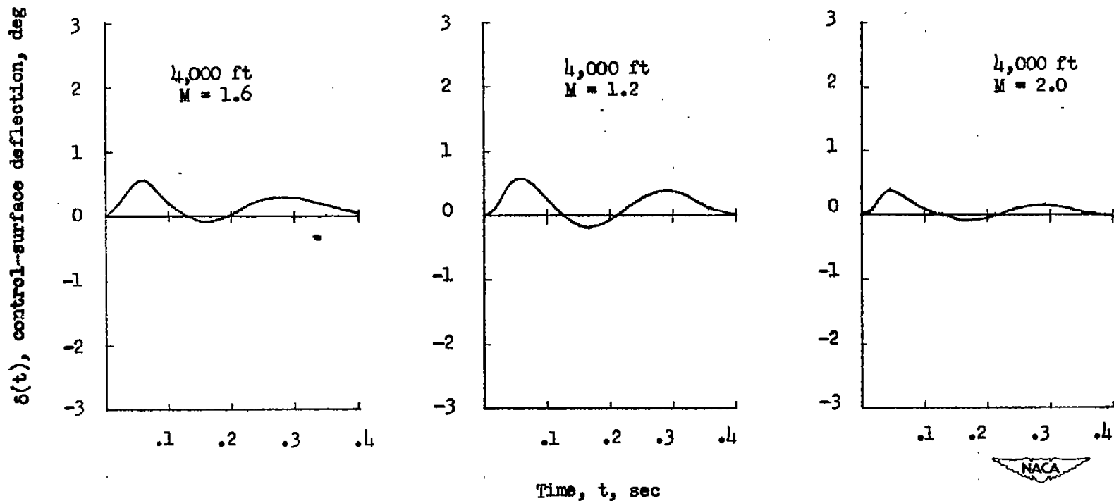
Figure 11.- Longitudinal transient responses \delta(t) of the missile to a unit step input signal calling for a change in attitude of 1^\circ . Static margin, 0.094\bar{c} at M = 1.6 ; K_R = 0.10 ; K_A = 1.26 .
