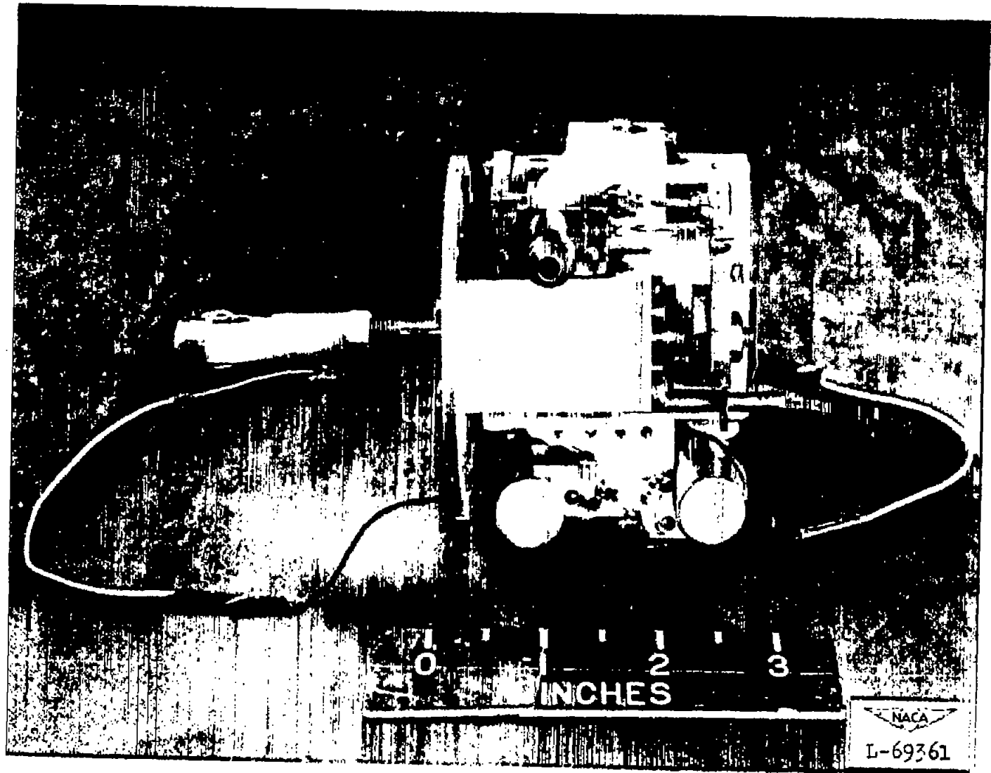
Figure 2.- Photograph of the rate gyro-servo.
