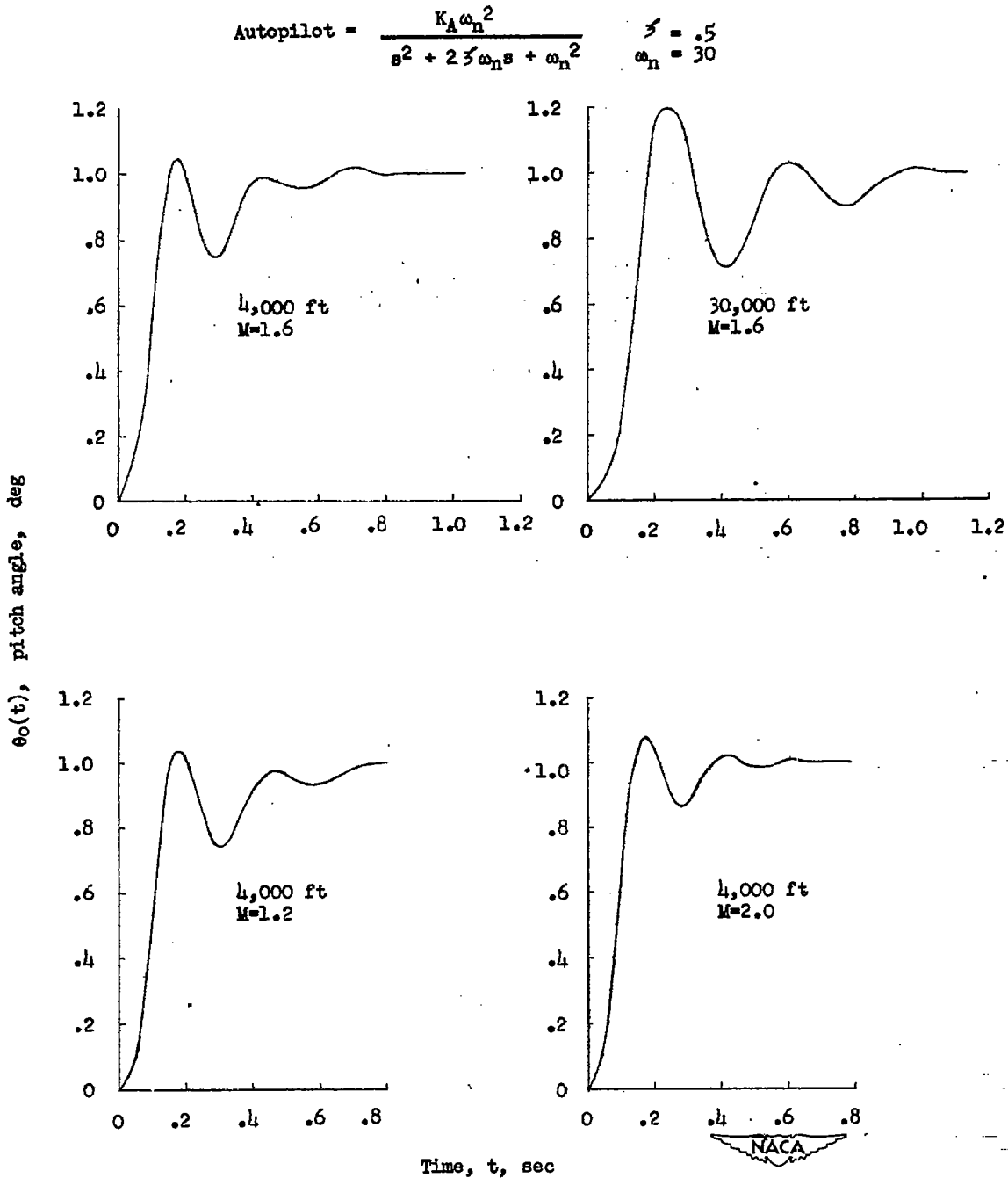
Figure 5.- Longitudinal transient responses \theta_0(t) of the missile to a unit step input signal calling for a change in attitude of 1^\circ . Static margin, 0.094\bar{c} at M = 1.6 ; K_T = 0.10 ; K_A = 1.26 .
