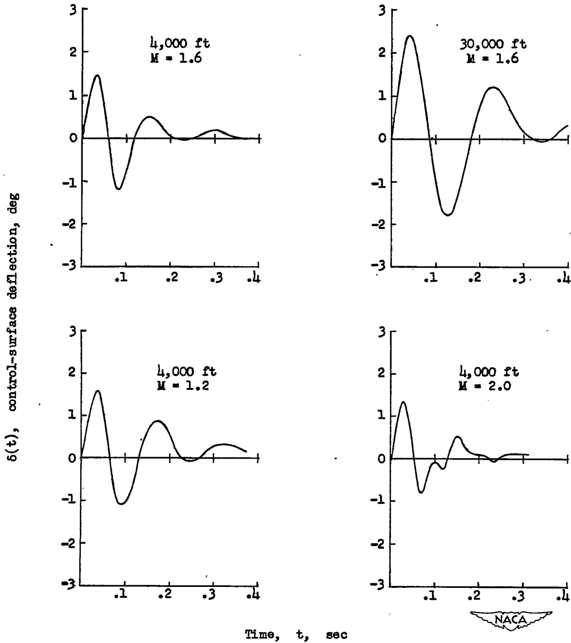
Figure 12.- Longitudinal transient responses \delta(t) of the missile to a unit step input signal calling for a change in attitude of 1^\circ . Static margin, 0.094\bar{c} at M = 1.6 ; K_r = 0.16 ; K_A = 2.82 .
