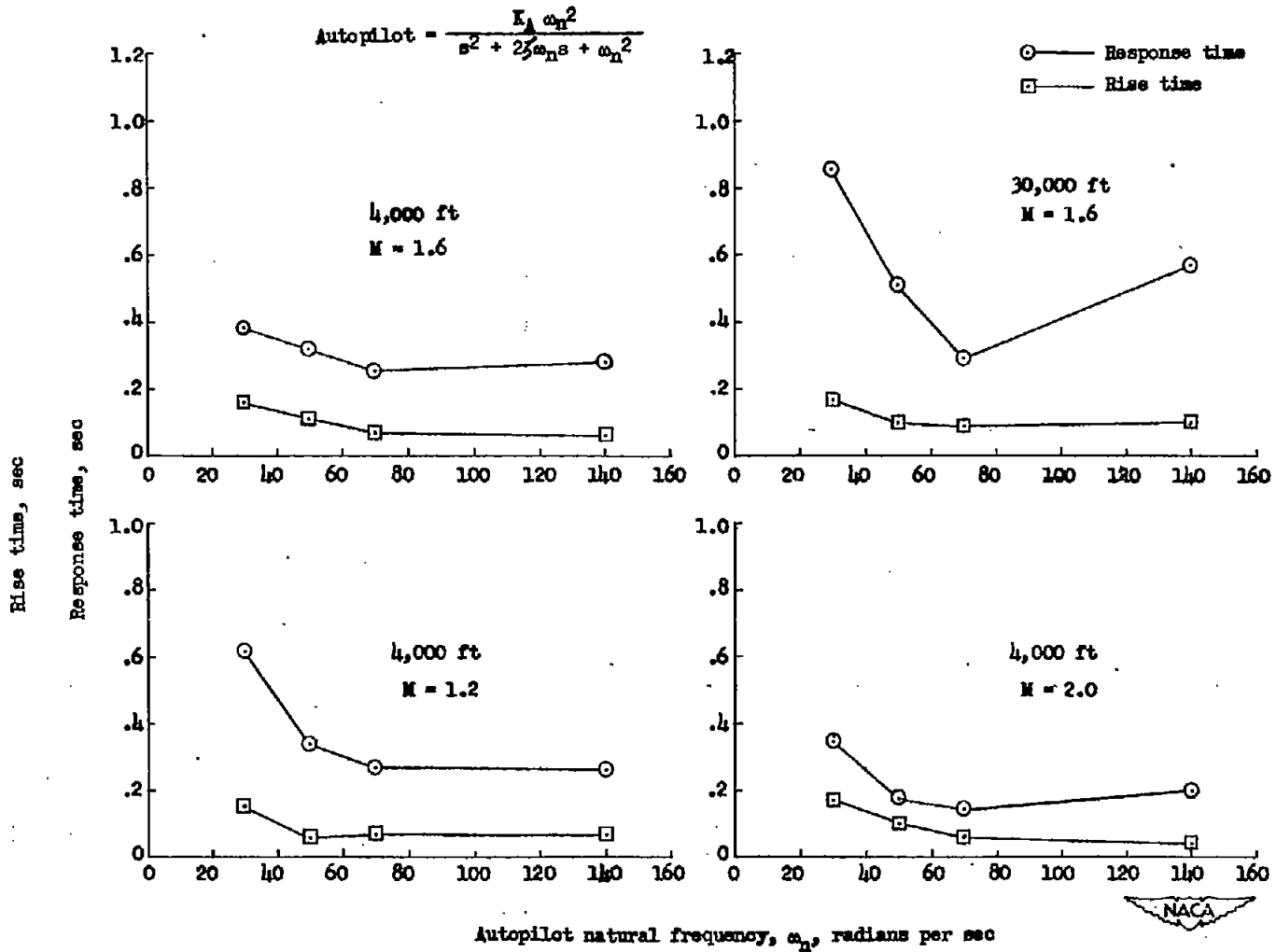
Figure 9.- Pitch-angle transient characteristics, response time, and rise time plotted against autopilot natural frequency. Static margin, 0.0948 at M = 1.6; \zeta of autopilot, 0.5.
