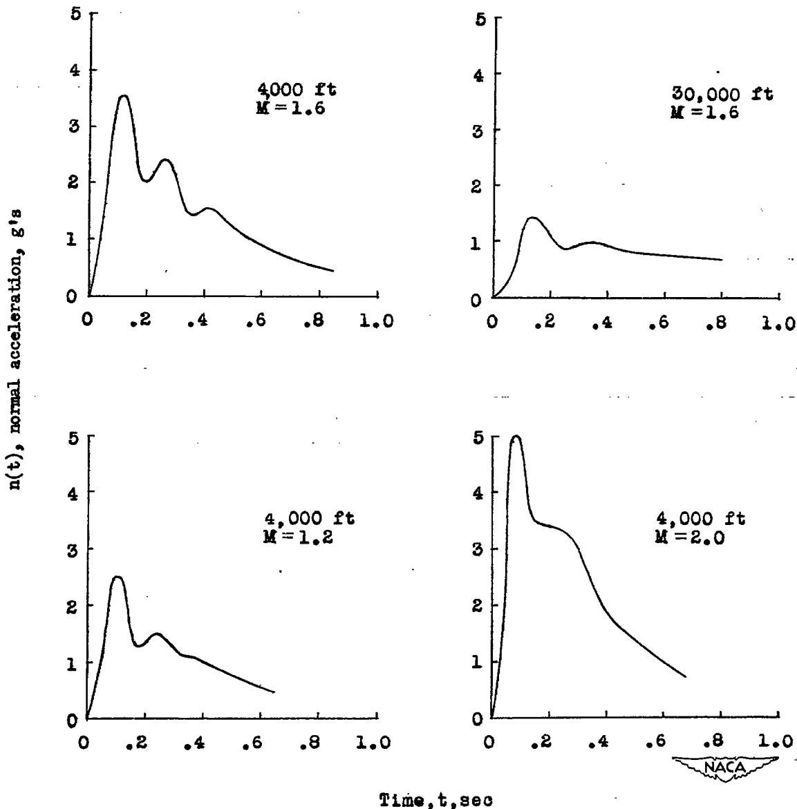
Figure 15.- Longitudinal transient responses for normal acceleration n(t) of the missile to a unit step input signal calling for a change in attitude of 1^\circ . Static margin, 0.094E at M = 1.6 ; K_r = 0.16 ; K_A = 2.82 .
