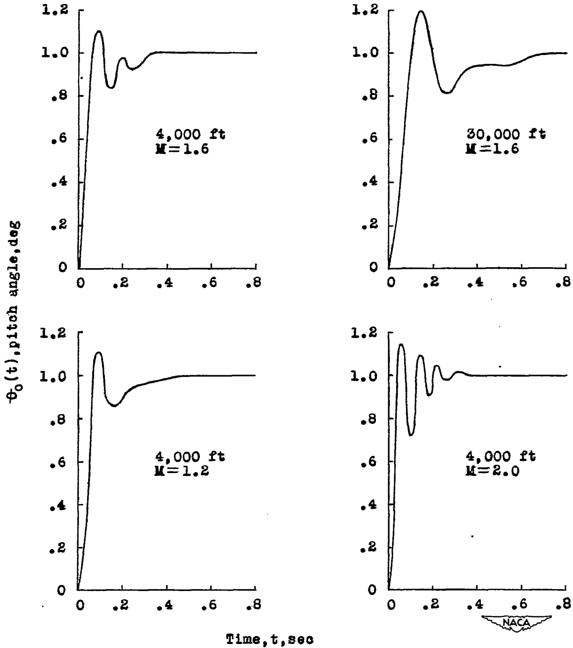
Figure 8.- Longitudinal transient responses \theta_0(t) of the missile to a unit step input signal calling for a change in attitude of 1^\circ . Static margin, 0.094\bar{c} at M = 1.6 ; K_r = 0.08 ; K_A = 2.32 .
