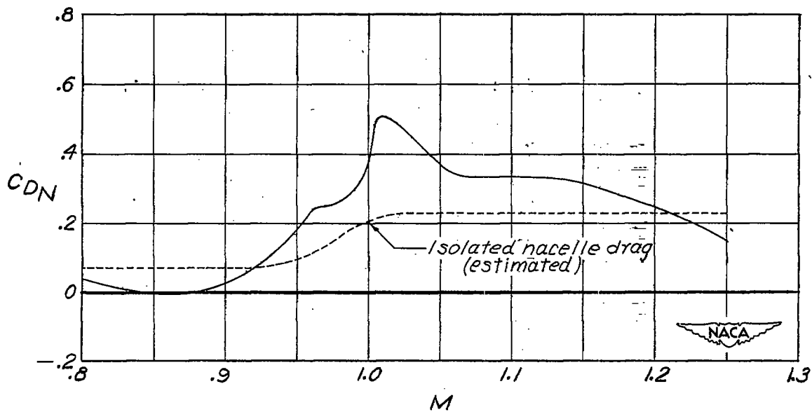
(c) Nacelles located at the wing 0.40 semispan station.
