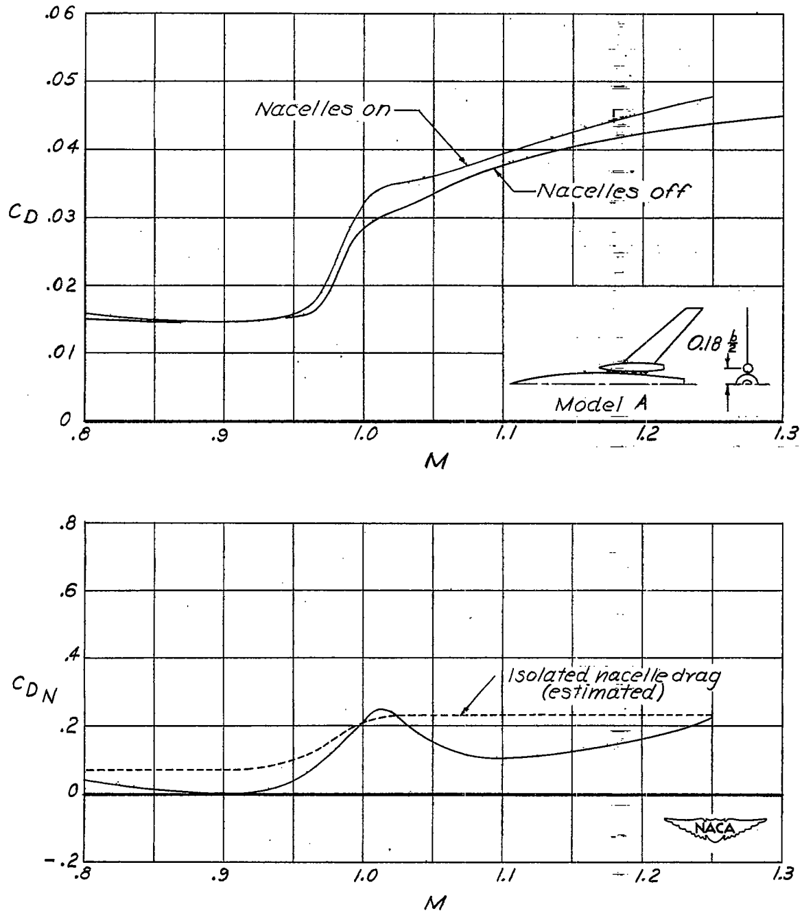
(a) Nacelles located at the wing 0.18 semispan station.
