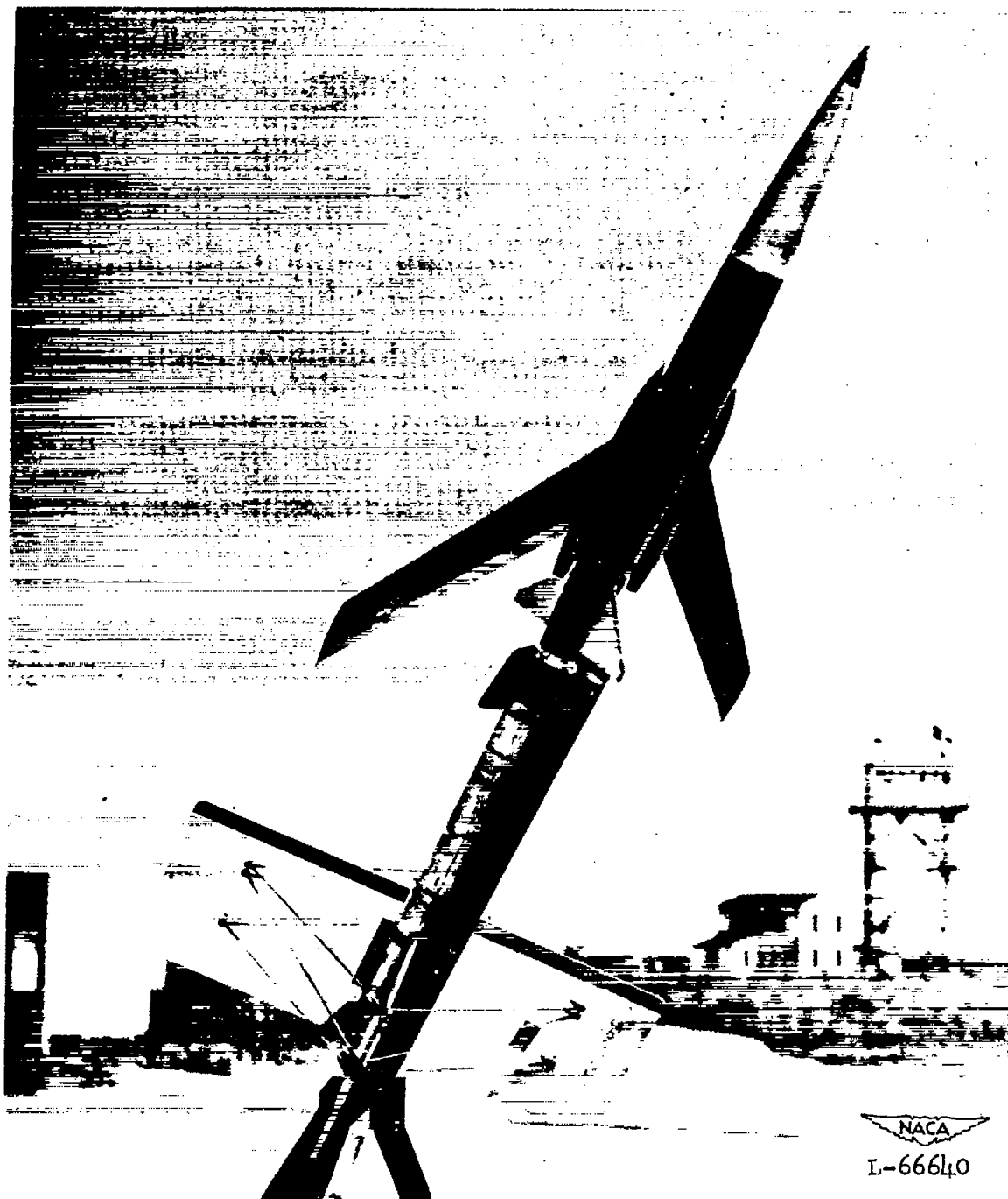
(a) Test model with nacelles. Model and booster arrangement in rail launcher.
