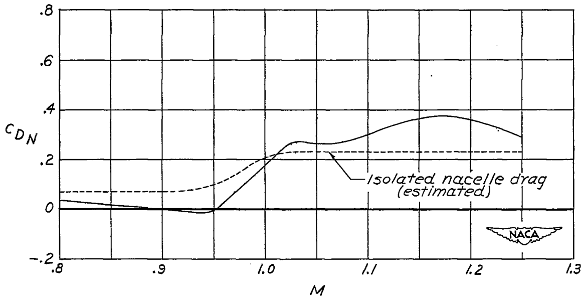
(b) Nacelles located at the wing 0.25 semispan station.
