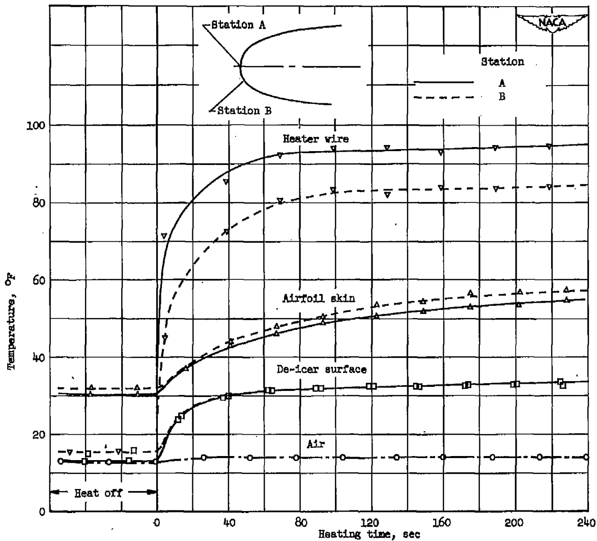
Figure 4. - Time history of heater temperatures during application of power. Airspeed, 250 miles per hour; air temperature, 14° F; angle of attack, 0°; power density, 5.2 watts per square inch.
