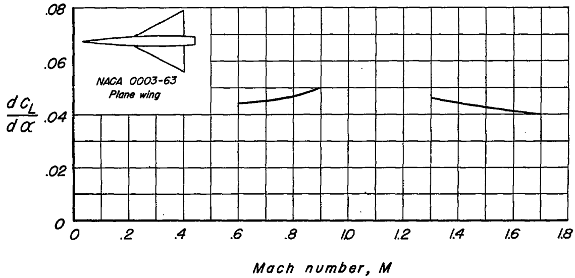
(a) \frac{dC_L}{d\alpha} vs M
