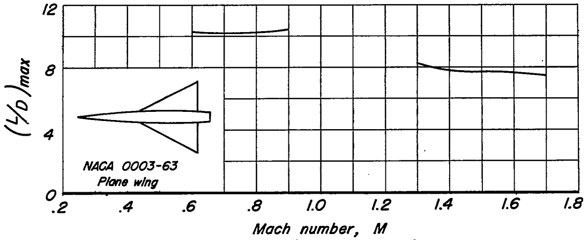
(c) (L/D)_{max} vs M
