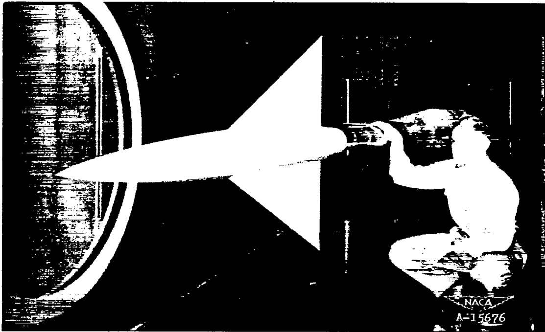
Figure 1.-- Model mounted in the Ames 6- by 6-foot supersonic wind tunnel.
