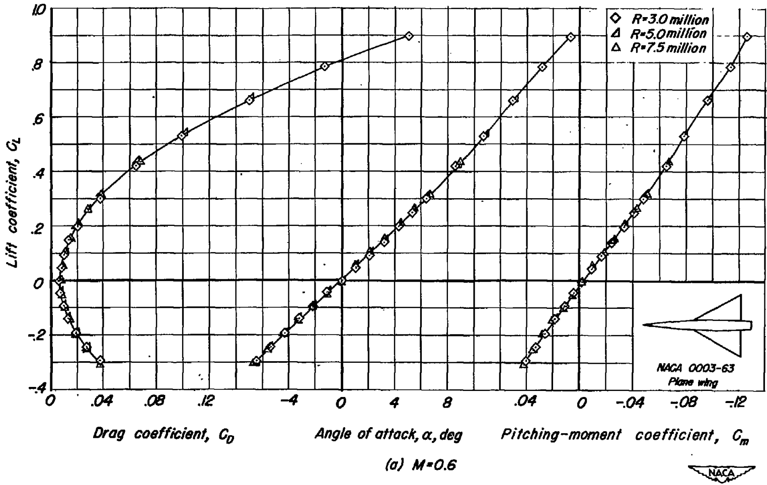
Figure 4.- The variation of the aerodynamic characteristics with lift coefficient at various Reynolds numbers.
