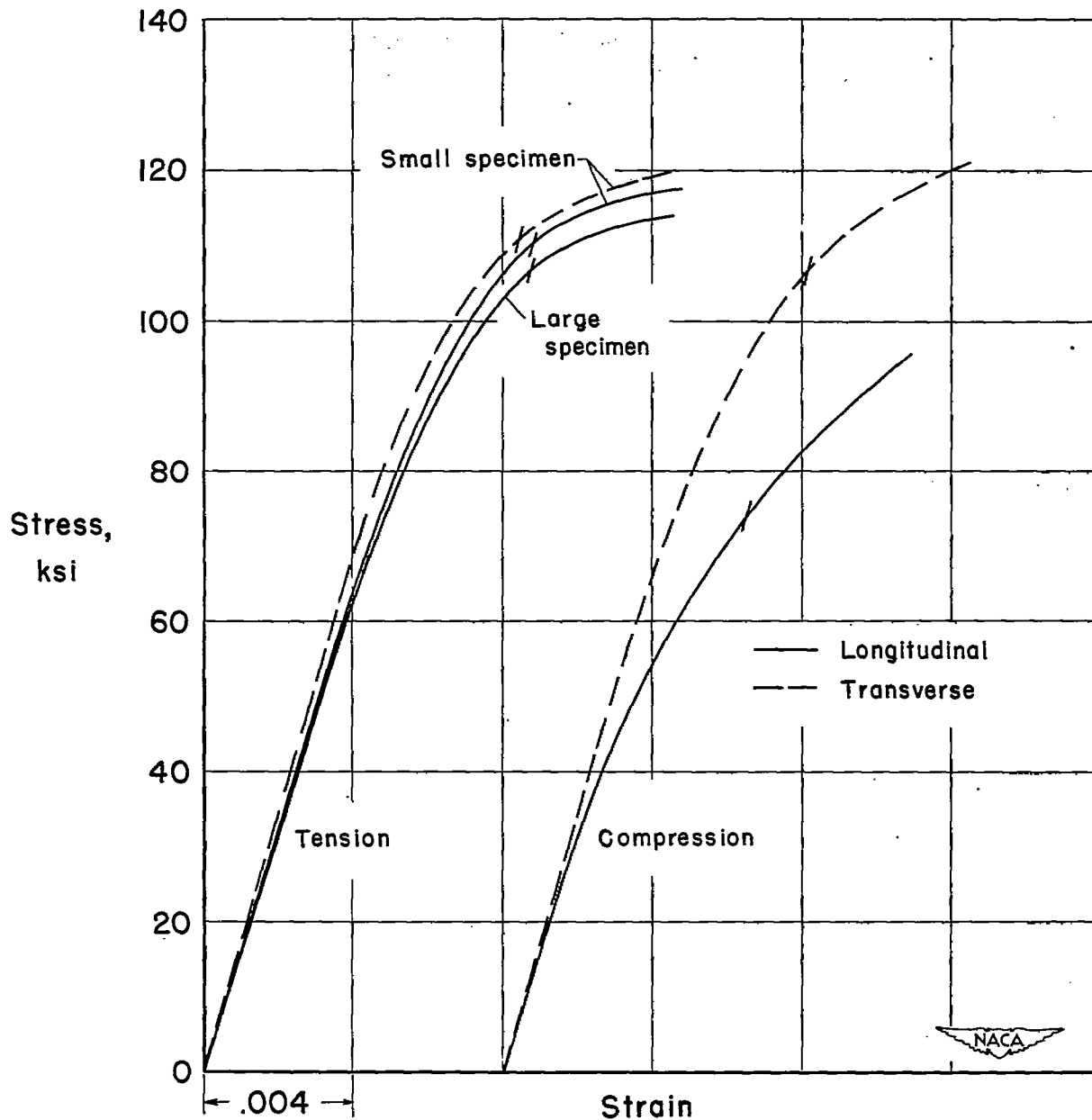
Figure 5.—Comparison of tensile and compressive properties of 20-percent cold-worked titanium sheet for both longitudinal and transverse grain directions at room temperature. (For tensile specimen dimensions, see fig. 1.)
