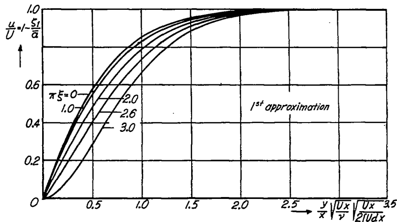
Figure 3.- A few laminar velocity profiles on the circular cylinder (first approximation).
