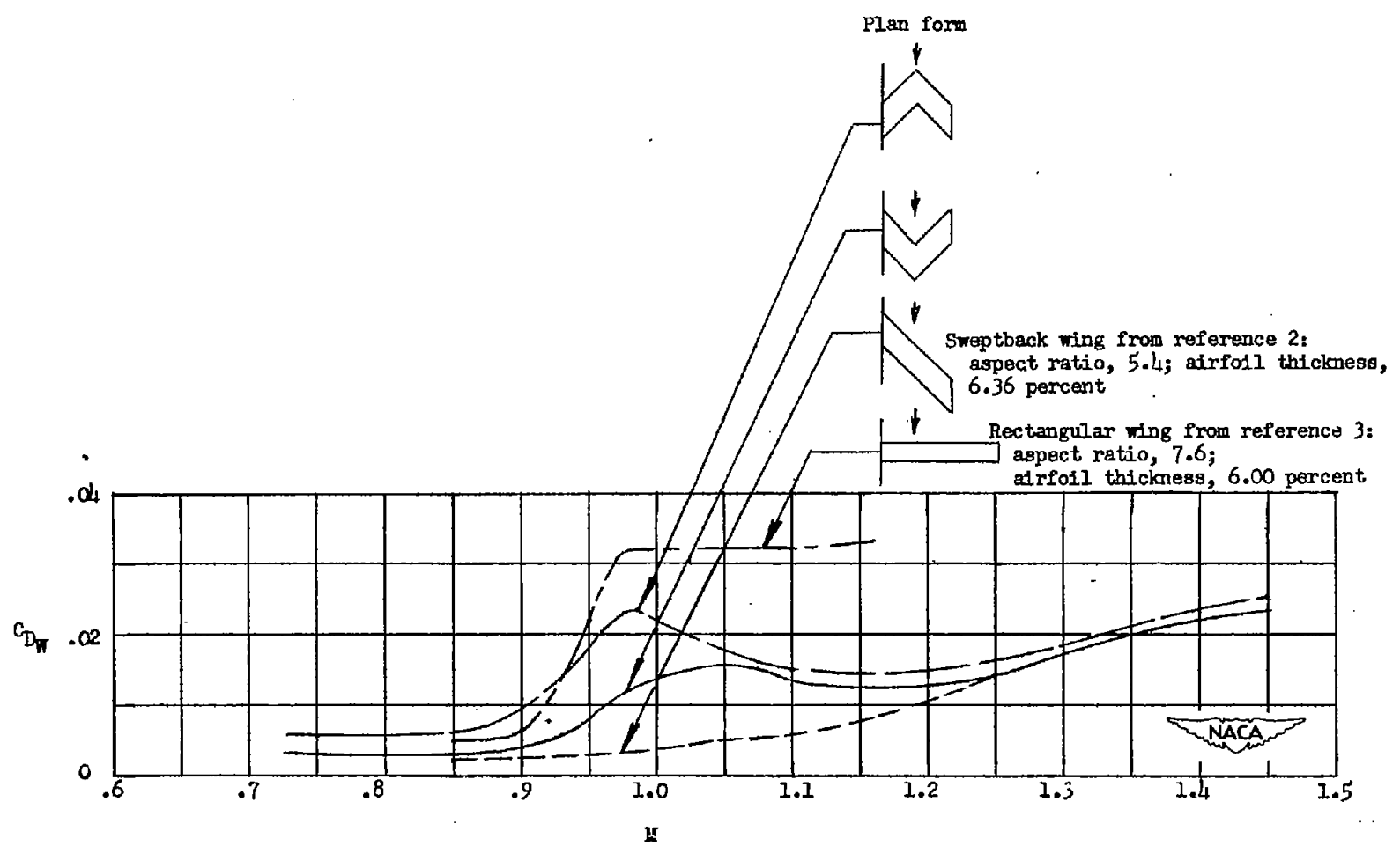
(a) Wings of aspect ratio 4 with NACA 65-006 airfoil sections. Also shown are drag coefficients for reference rectangular and sweptback wings with NACA 65-series airfoil sections.
