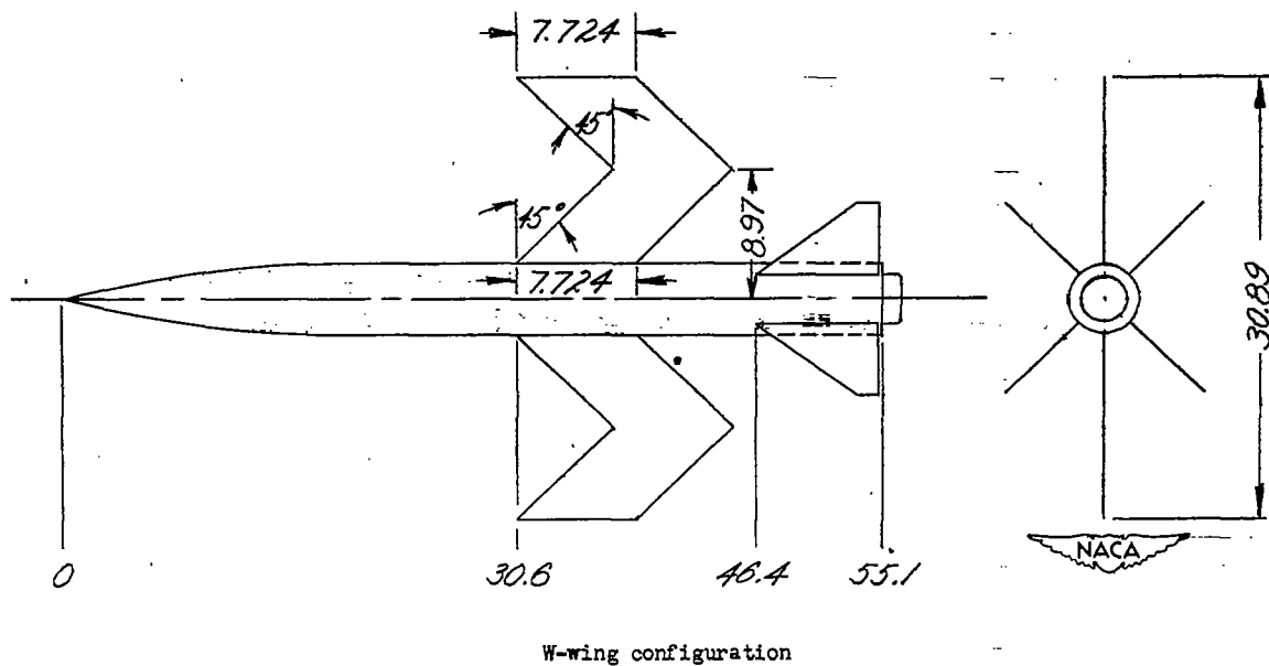
(a) General arrangement. All dimensions shown in inches.
