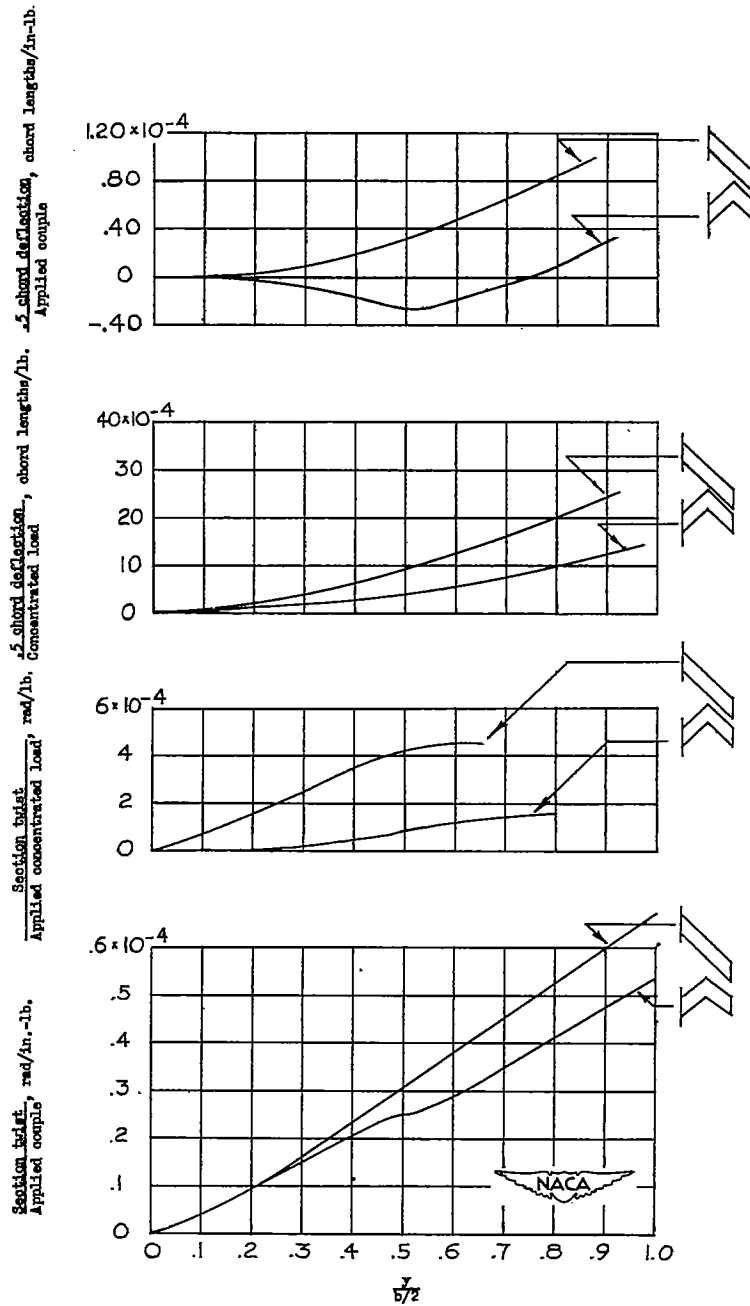
(a) Aspect ratio 8.
