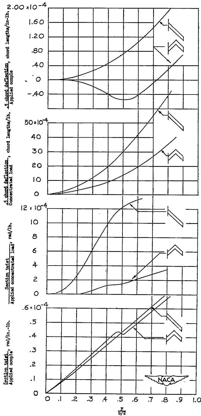
(c) Aspect ratio 12.
