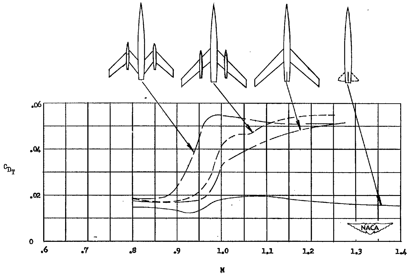
(b) Wings of aspect ratio 6 and NACA 65A009 airfoil sections.
