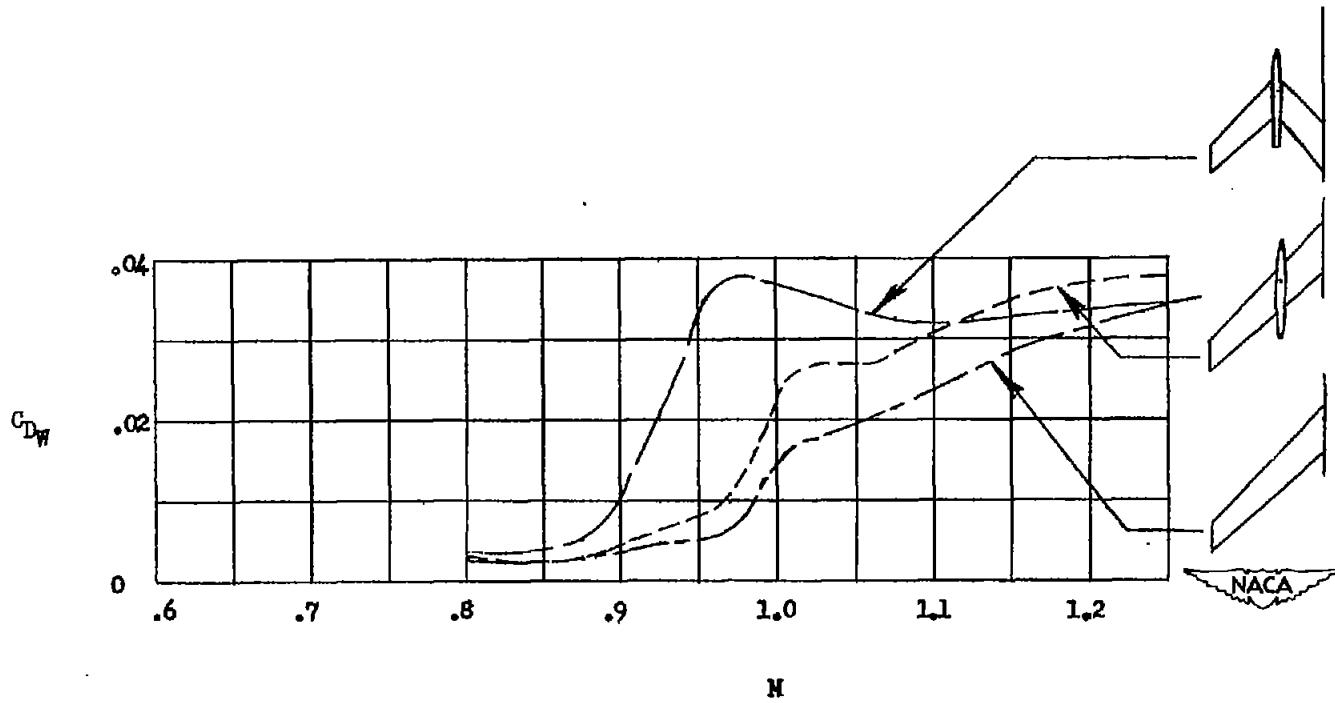
(b) Wings of aspect ratio 6 with NACA 65A009 airfoil sections.
