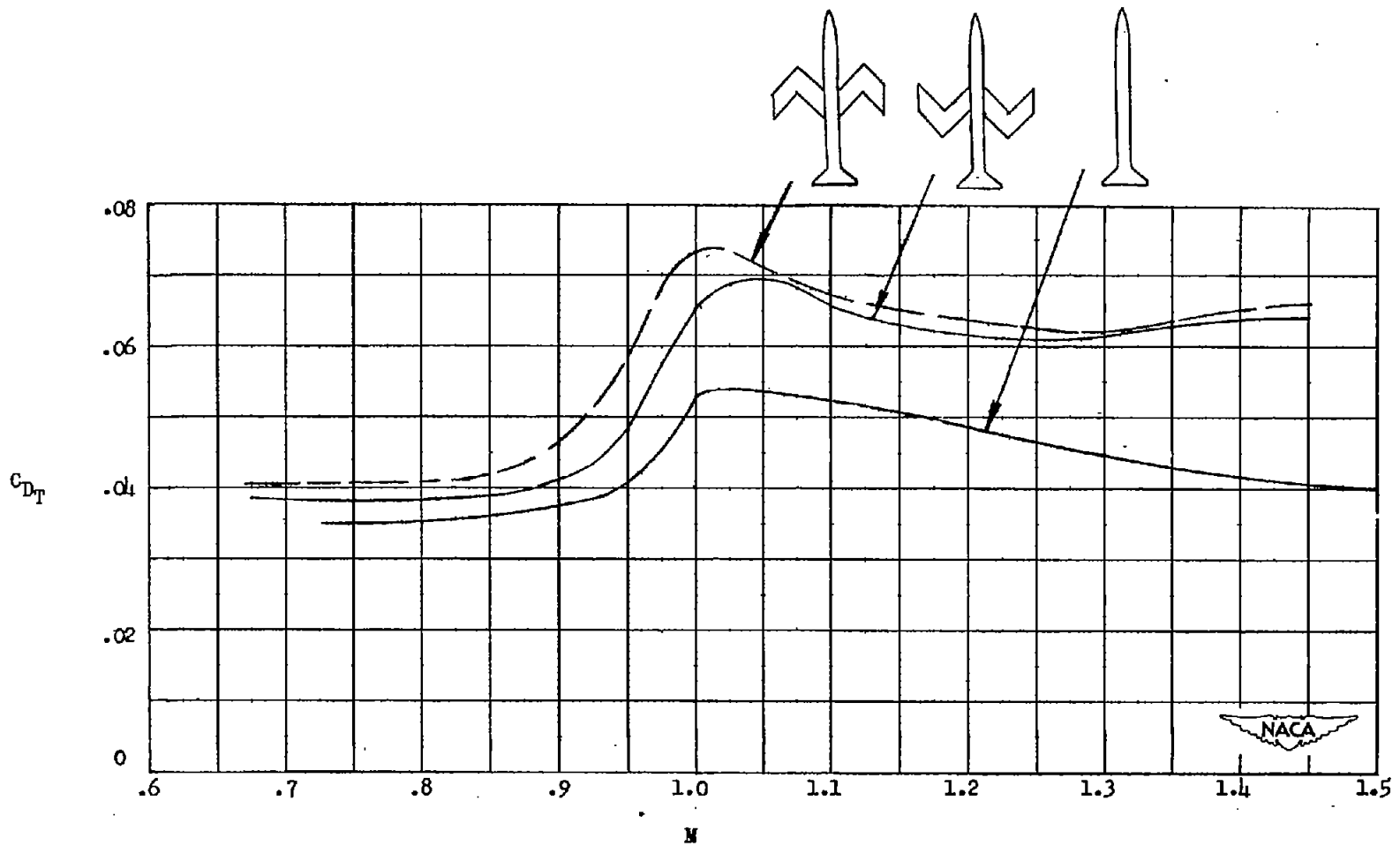
(a) Wings of aspect ratio 4 and NACA 65-006 airfoil sections.
