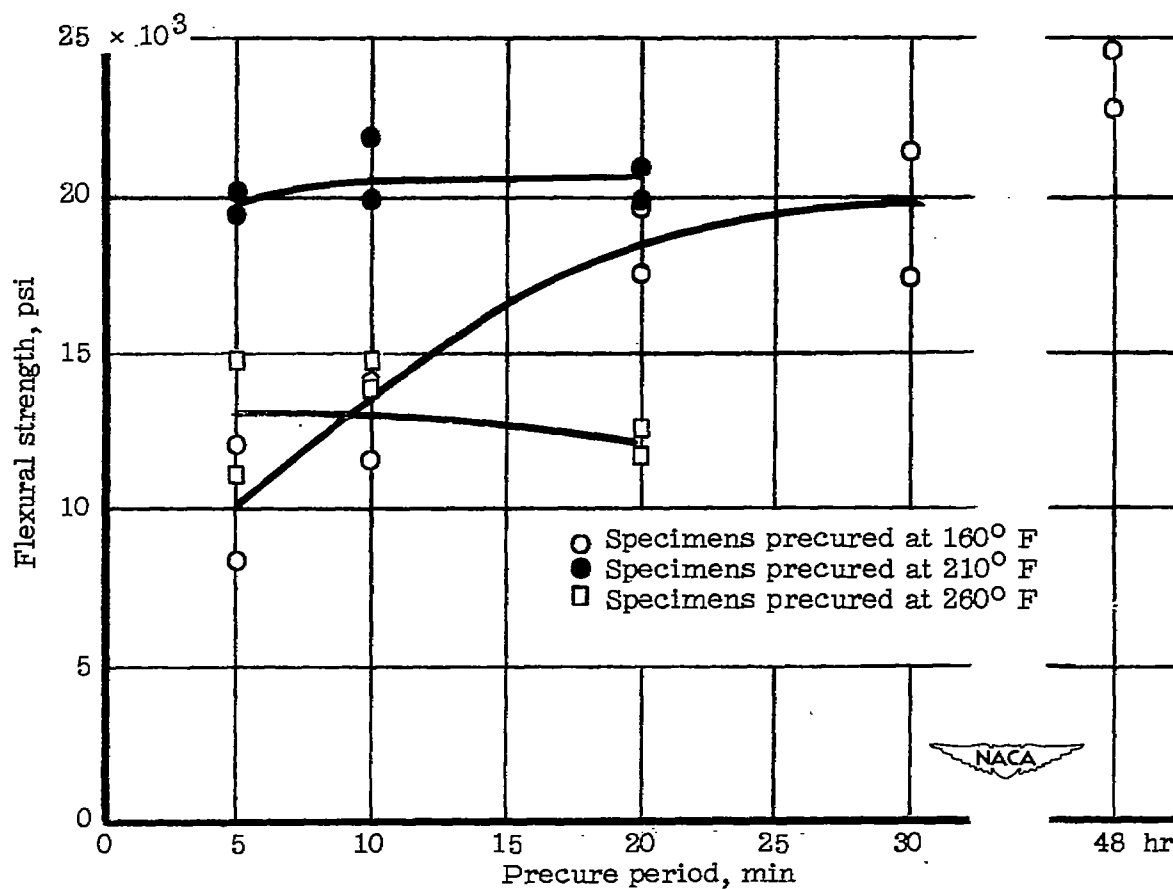
Figure 5.- Effect of variations in precure molding cycle on dry flexural strength.
