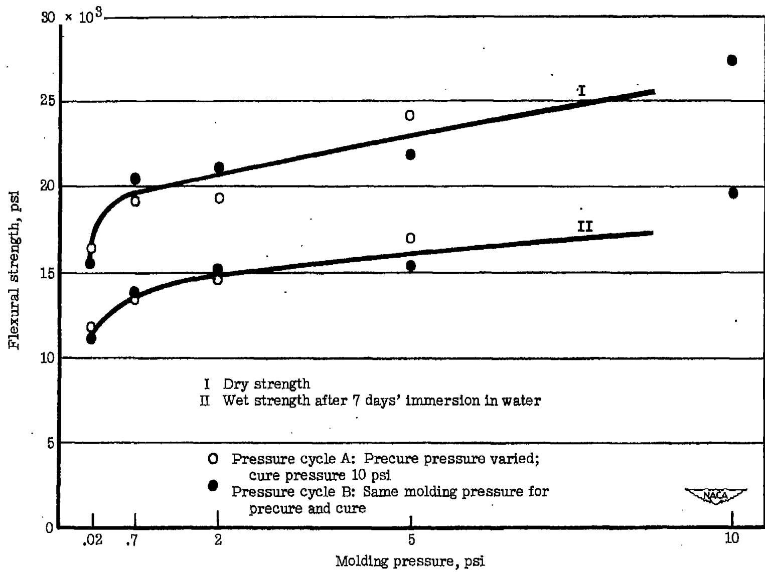
Figure 1.- Effect of molding pressure on flexural strength.
