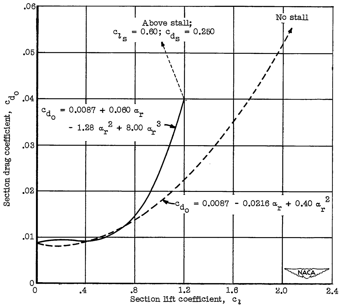
Figure 6.- Section drag polars (two different assumptions). a = 5.60 per radian.
