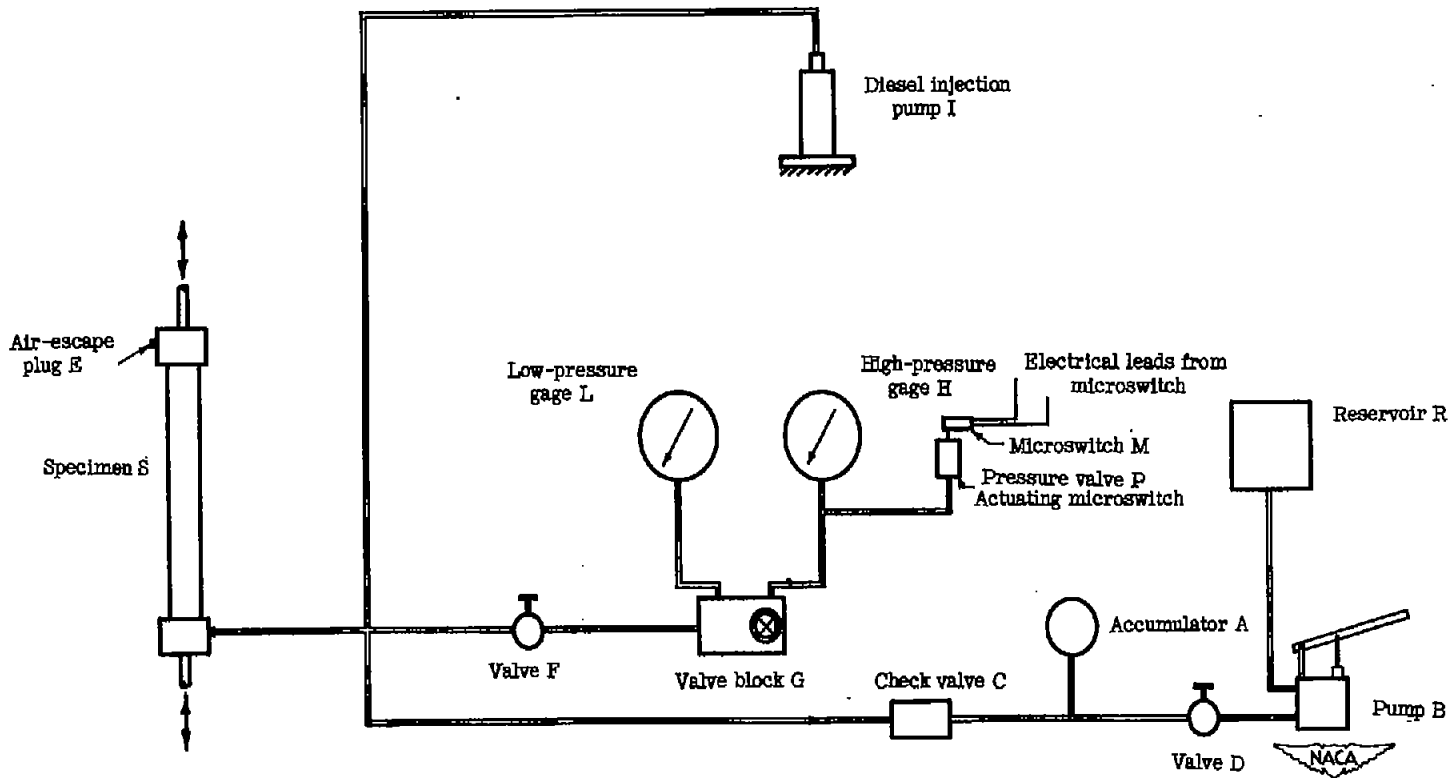
Figure 5.- Internal-pressure loading arrangement.
