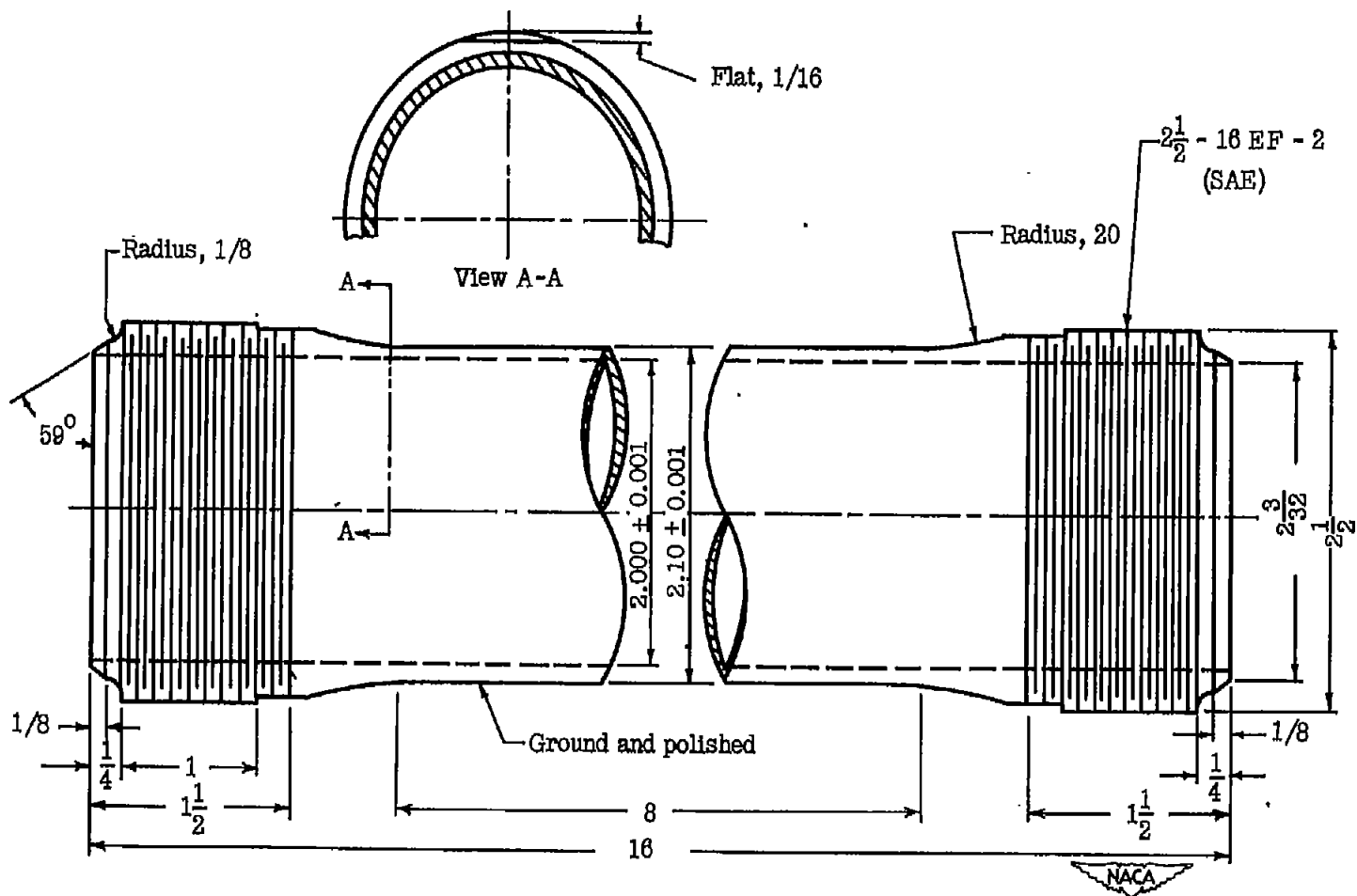
Figure 3.- Biaxial stress specimen. All dimensions are in inches.
