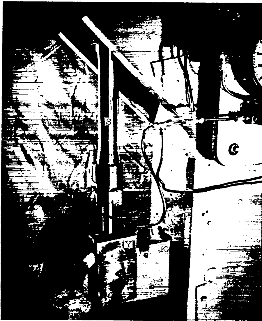
Figure 11.- Specimen in position for testing.
