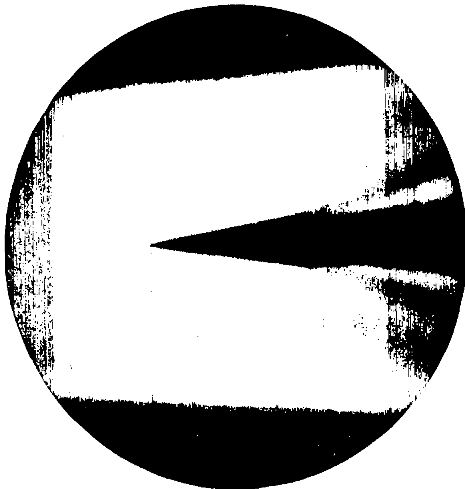
Figure 5.- Photograph of afterglow flow pattern over a 15^\circ double-wedge model at a stagnation pressure of 60 millimeters of mercury and an indicated Mach number of 2.6.
