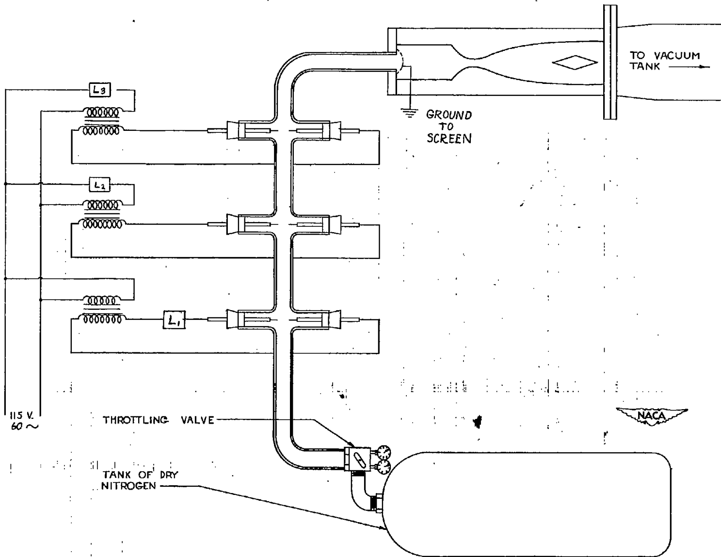
Figure 1.— Sketch of apparatus for producing afterglow in a supersonic stream of nitrogen.
